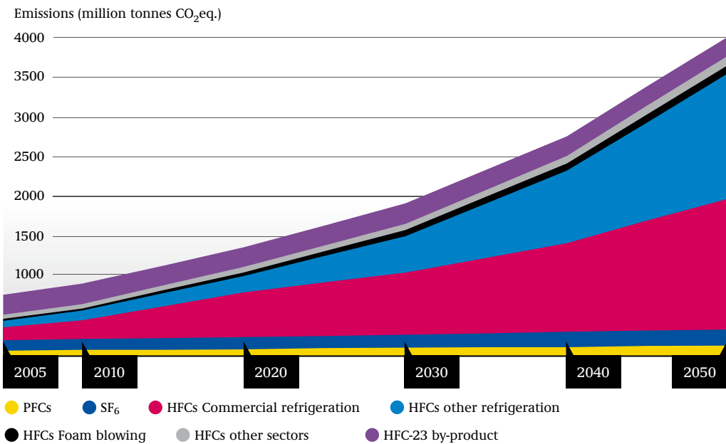
GLOBAL FORECASTS OF FLUORINATED GREENHOUSE GAS EMISSIONS IN THE MAIN FIELDS OF APPLICATION IN MILLION TONNES CO 2 EQUIVALENT (“BUSINESS-AS-USUAL SCENARIO”)
