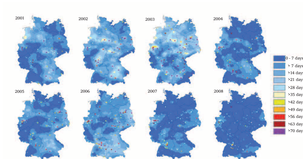
Figure 10: PM 10 pollution – number of days with PM 10 daily mean values in excess of 50 µg/m 3 - in Germany 2001 to 2008 with “spots”.
