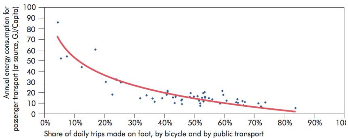
Figure 2-2. Energy consumption for passenger transport vs. Modal share. IEA 2008.
