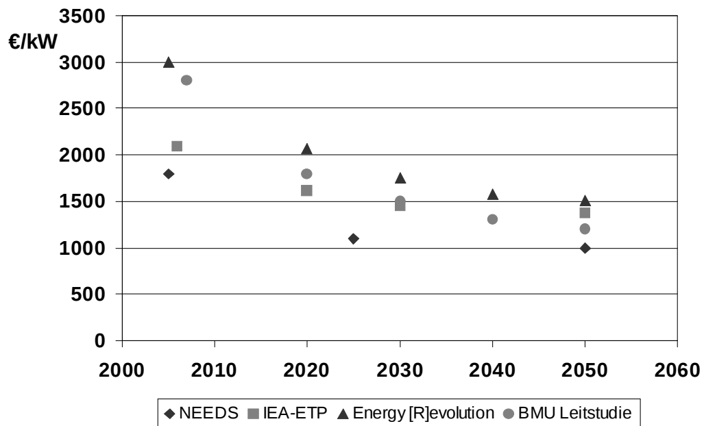
Figure 2-5: Comparison of offshore wind investment cost projections
