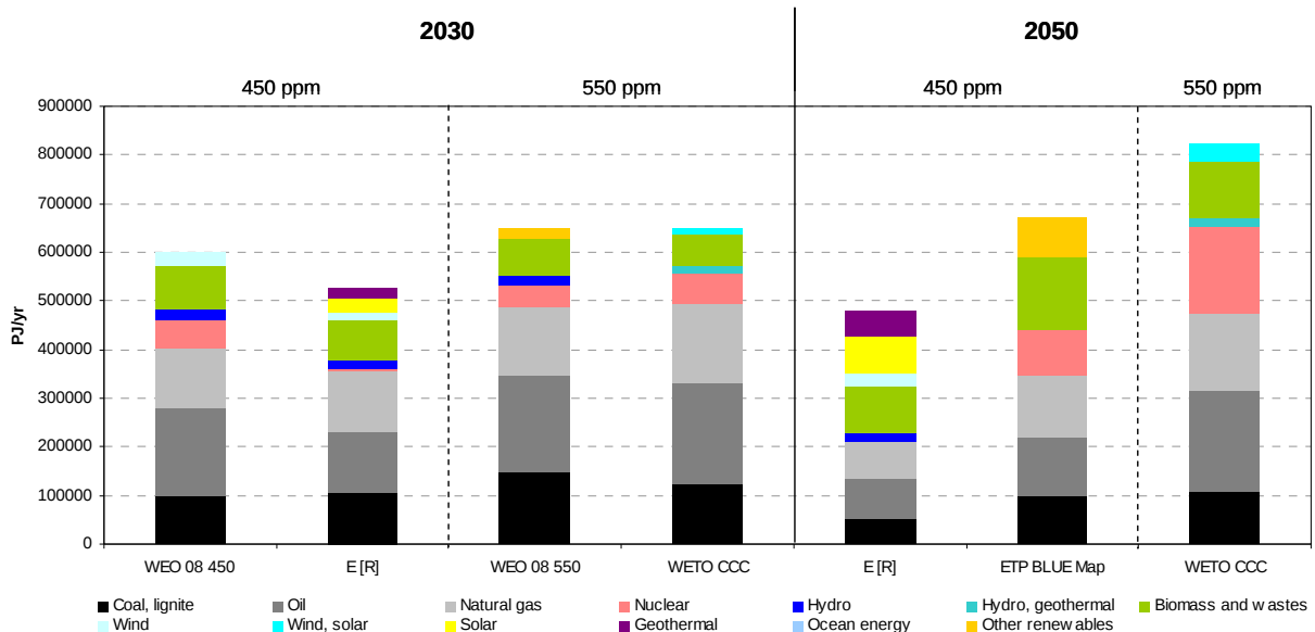
Figure 3-1: Primary energy demand. Segmentation follows time and climate target.
