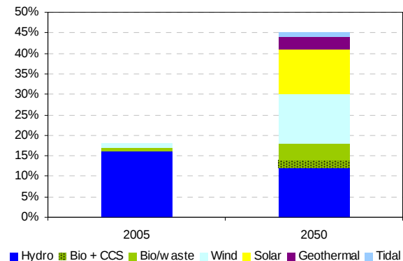
Figure 2-39: IEA ETP 2008 BLUE Map, Share of renewable energy in electricity generation
