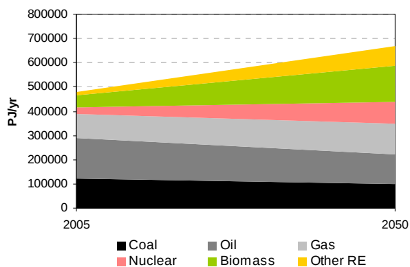
Figure 2-34: IEA ETP 2008 BLUE Map, Primary energy demand
