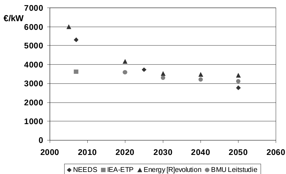
Figure 2-3: Comparison of CSP investment cost projections
