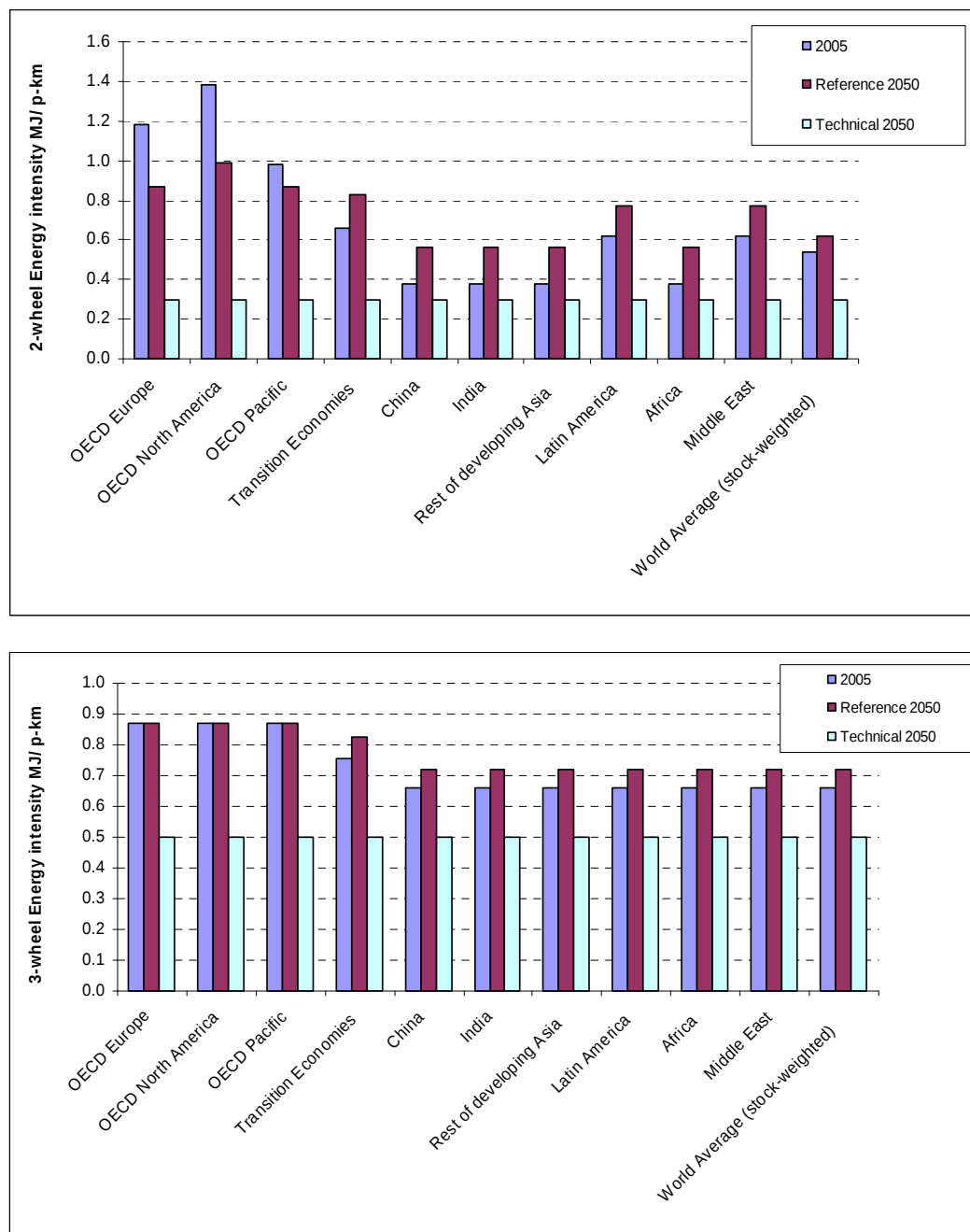
Figure 33: Reference scenario and 2050 technical potential energy intensities for different regions for 2 and 3-wheel vehicles, respectively
