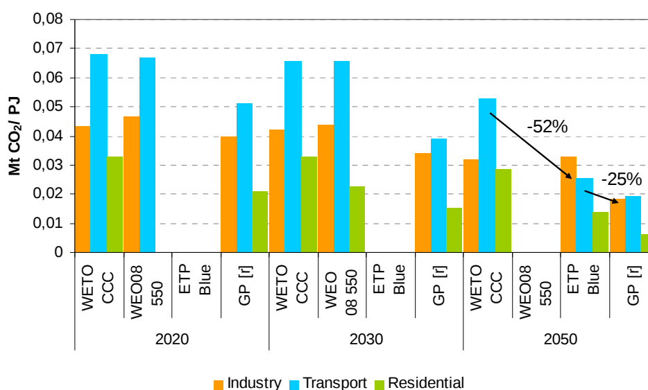
Figure 3-3: Carbon intensity of final energy demand
