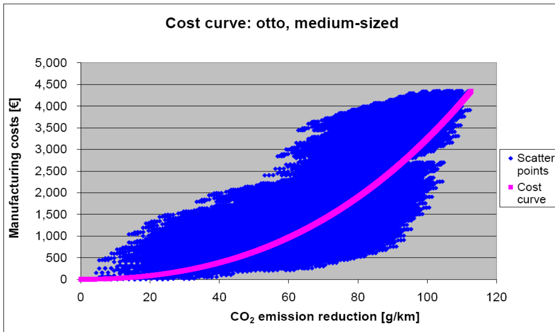
Annex 6: Potentials and manufacturing costs of all packages of measures, resulting additional cost curve. Cars with medium-sized otto engines (capacity 1.4 - 2.0 litres)
