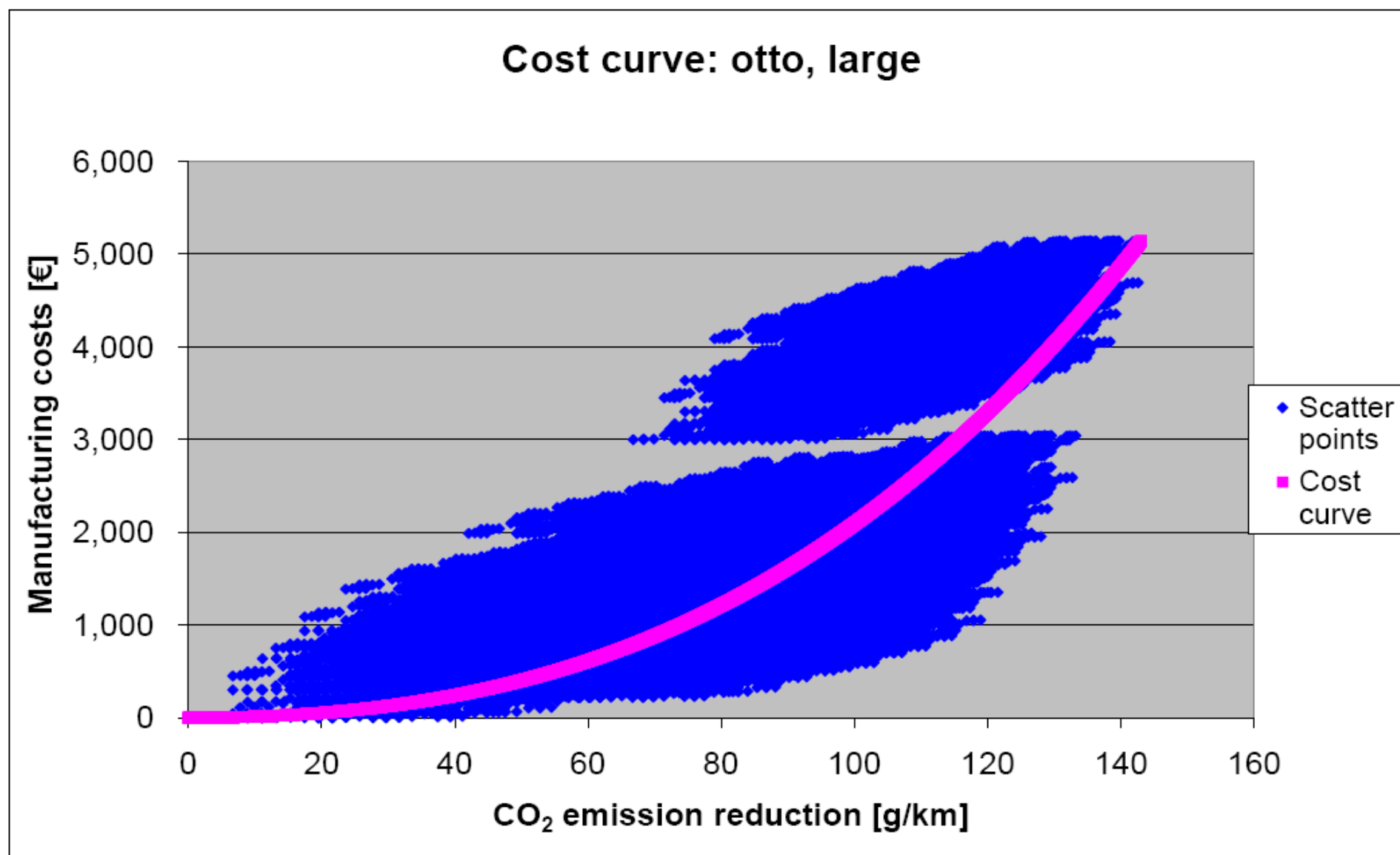
Annex 7: Potentials and manufacturing costs of all packages of measures, resulting additional cost curve. Cars with large otto engines (capacity >2.0 litres)
