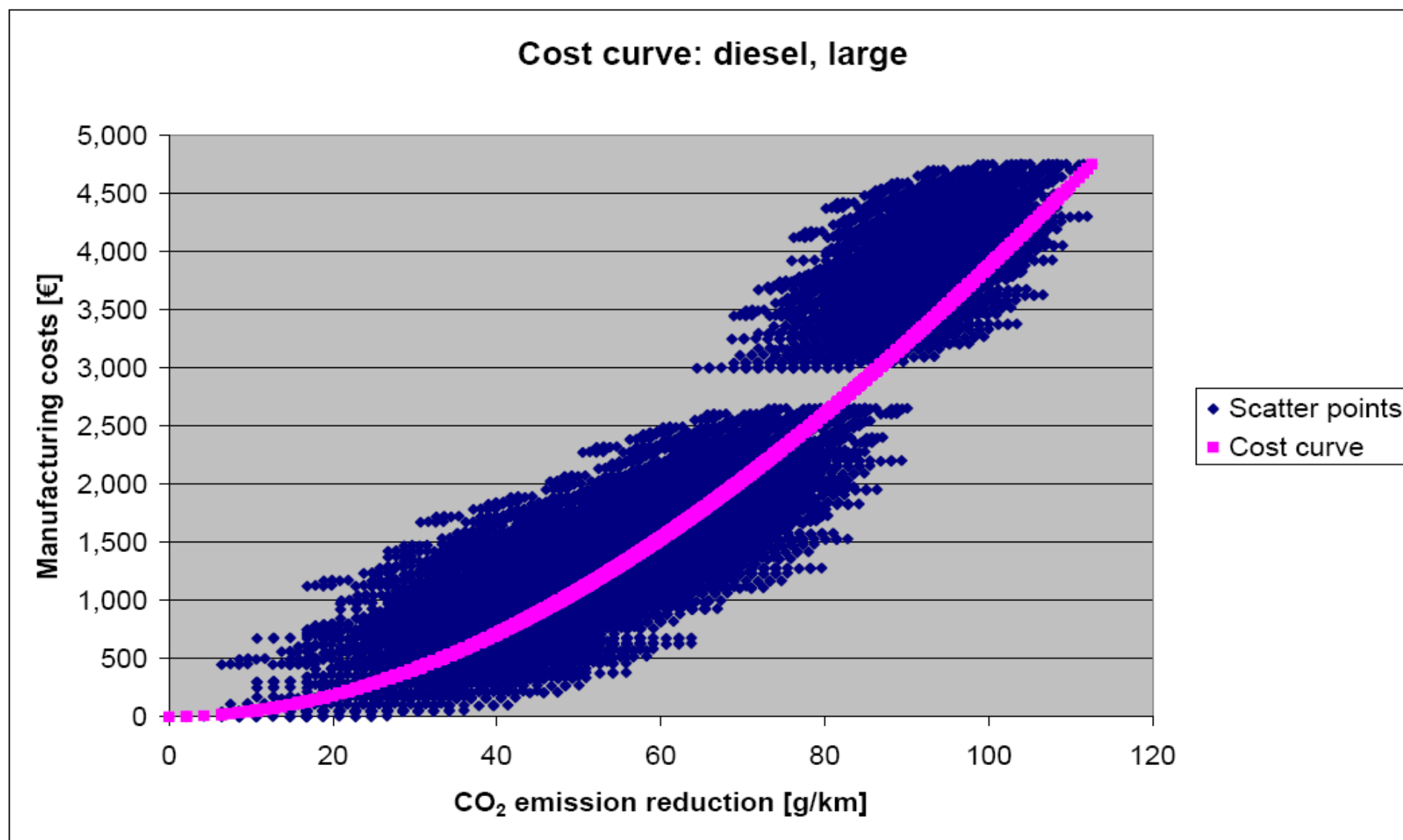
Annex 10: Potentials and manufacturing costs of all packages of measures, resulting additional cost curve. Cars with large diesel engines (capacity > 2.0 litres)
