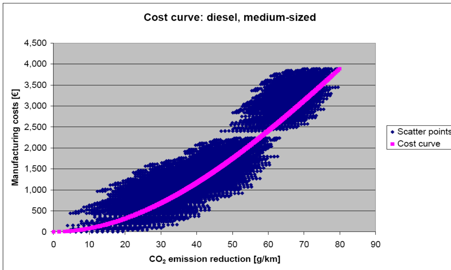
Annex 9: Potentials and manufacturing costs of all packages of measures, resulting additional cost curve. Cars with med.-sized diesel engines (capacity 1.4-2.0 litres)
