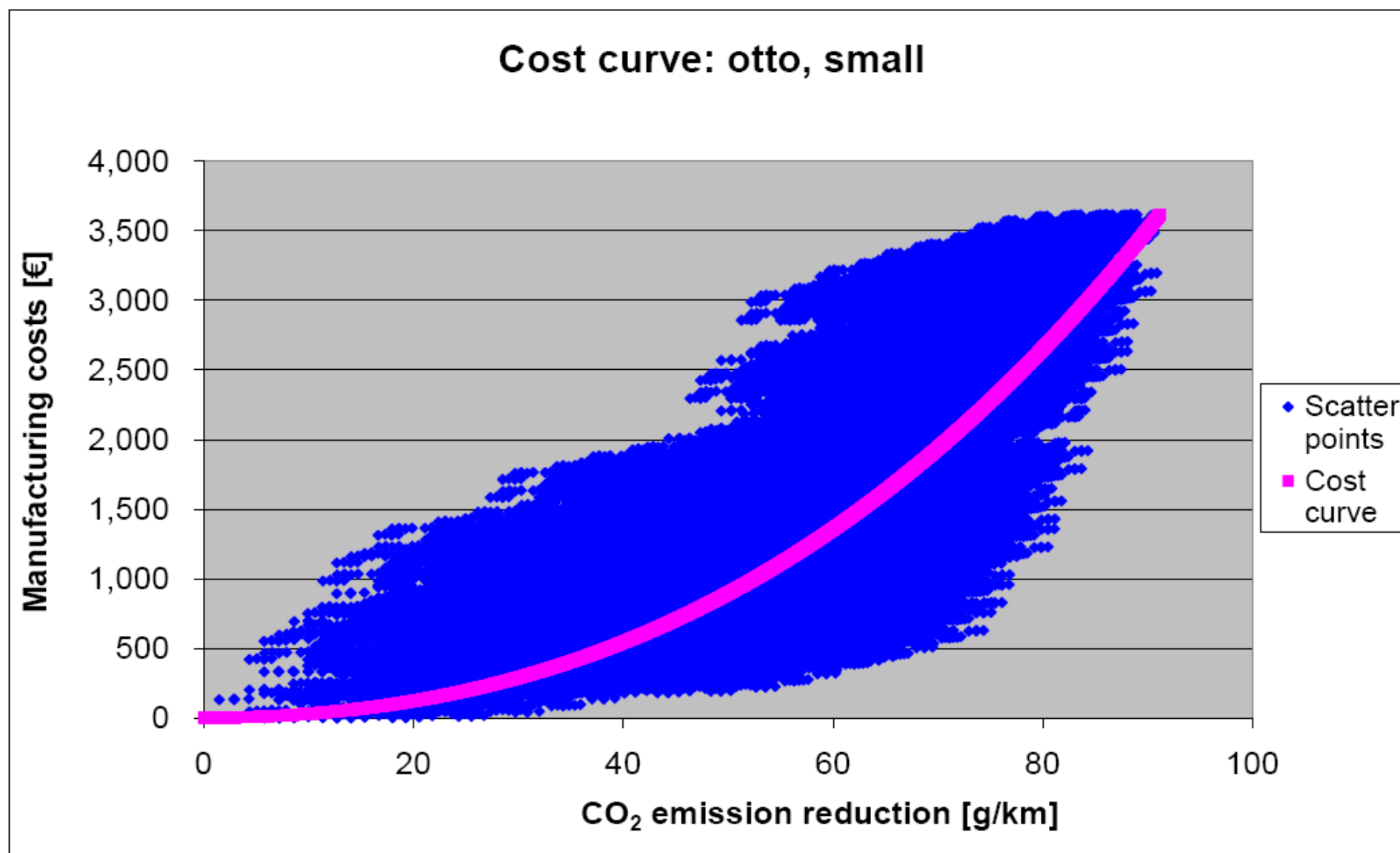
Annex 5: Potentials and manufacturing costs of all packages of measures, resulting additional cost curve. Cars with small otto engines (capacity < 1.4 litres)
