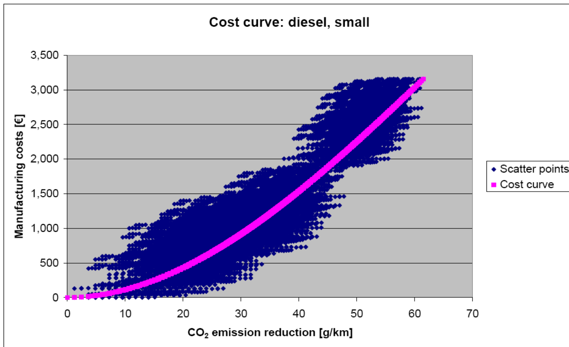
Annex 8: Potentials and manufacturing costs of all packages of measures, resulting additional cost curve. Cars with small diesel engines (capacity <1.4 litres)
