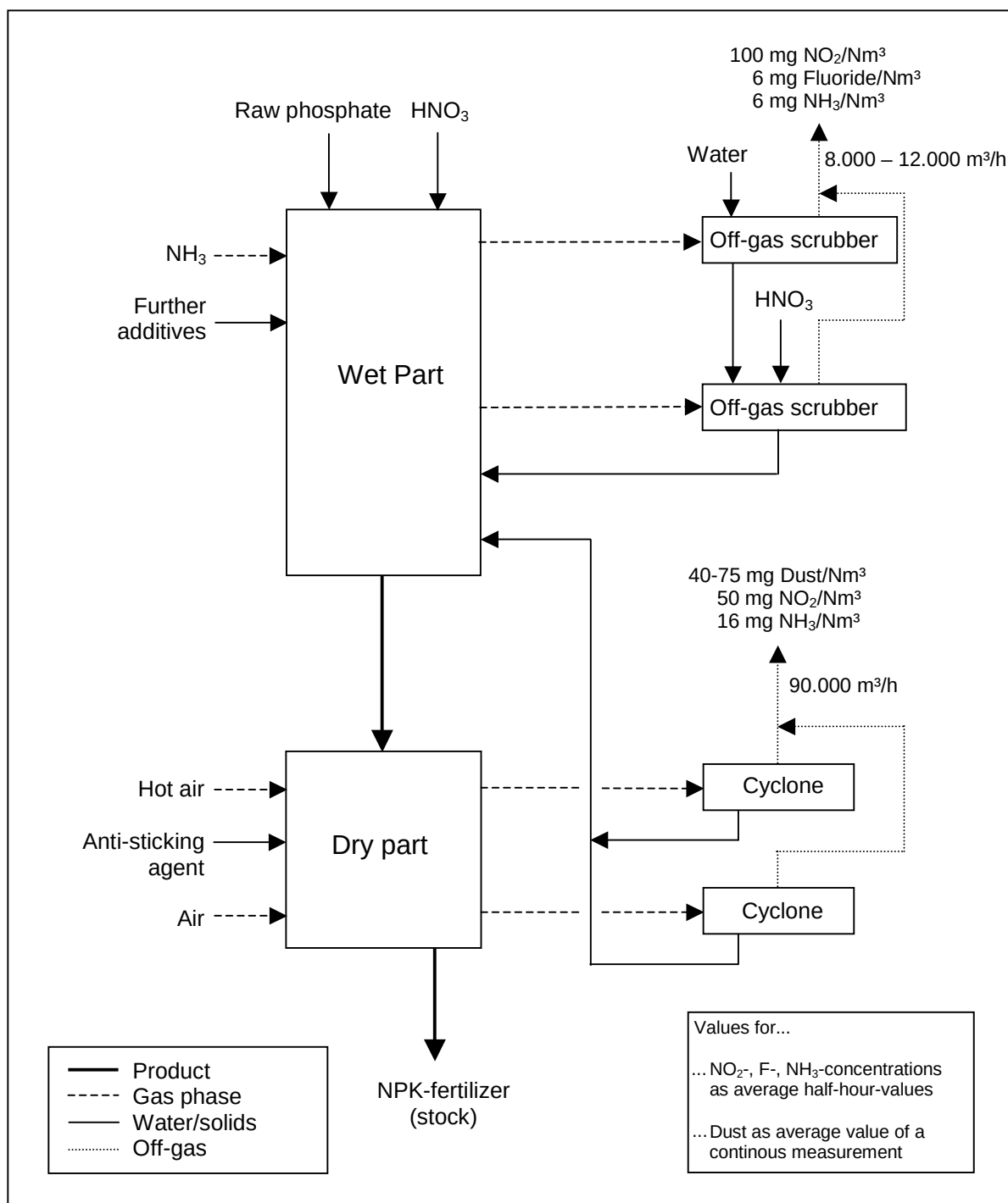
Figure 2: Emission Sources and Off-gas Concentrations
