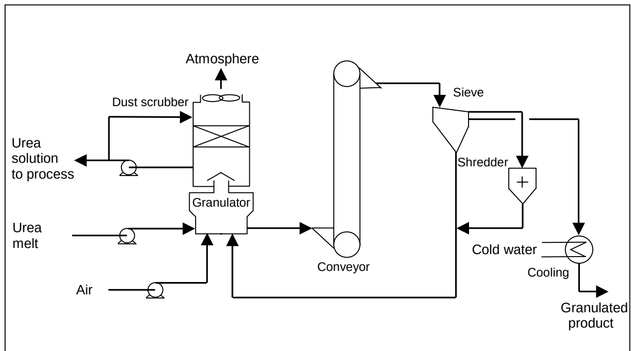
Figure 4: Granulation Technology of Toyo Engineering
