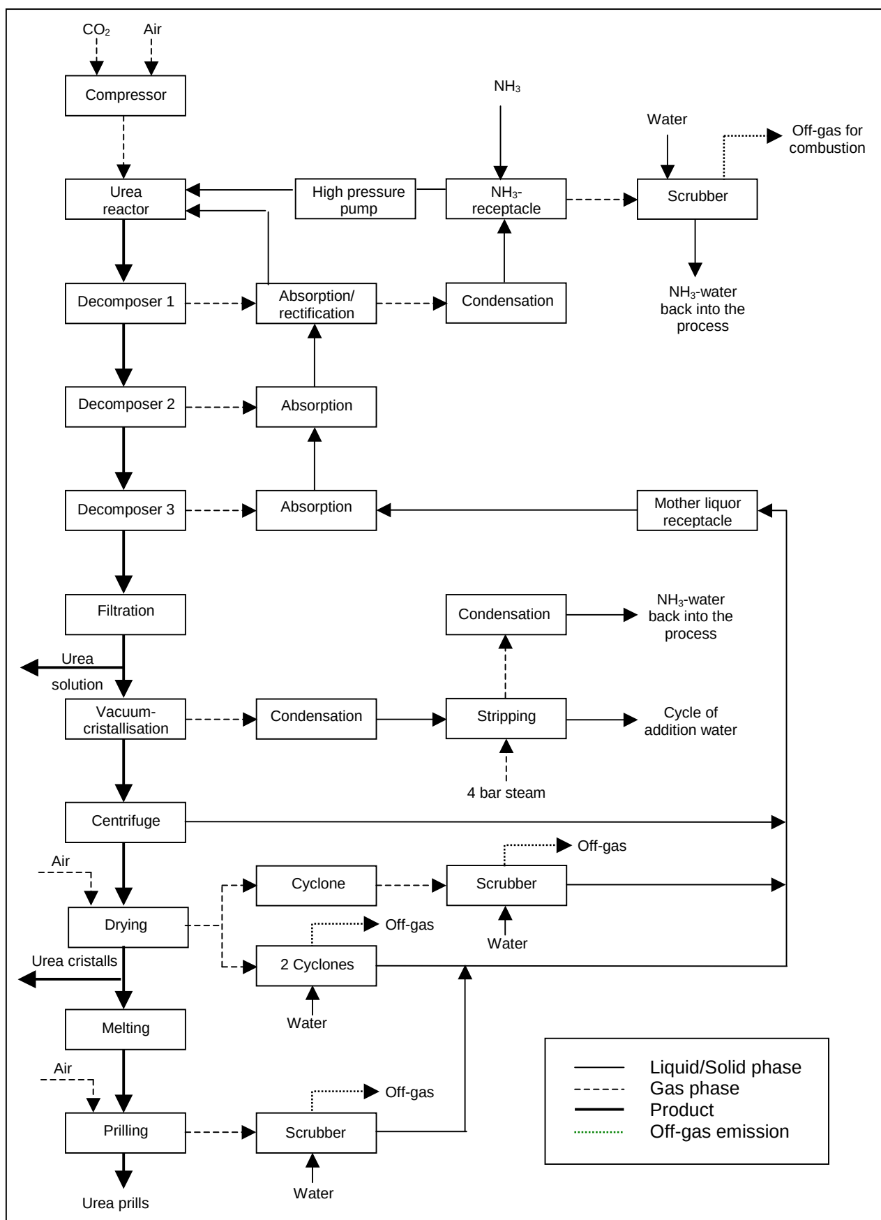
Figure 1: Total Recycle Technology
