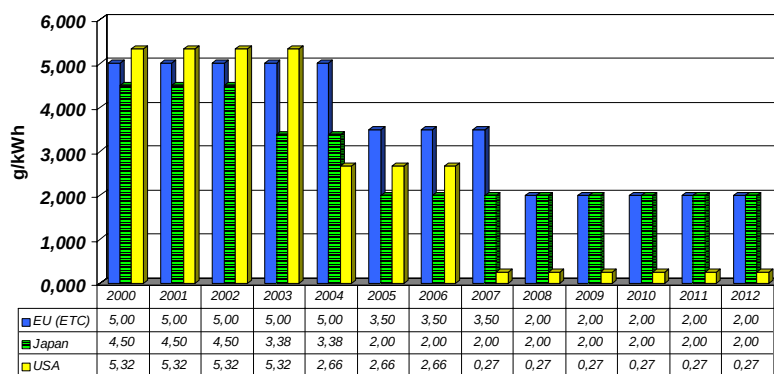
NOx limit values for heavy-duty engines in g/kWh
