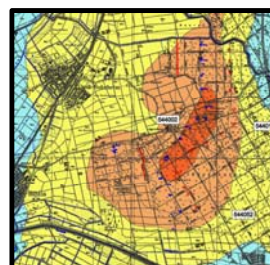
Differenzenplan
