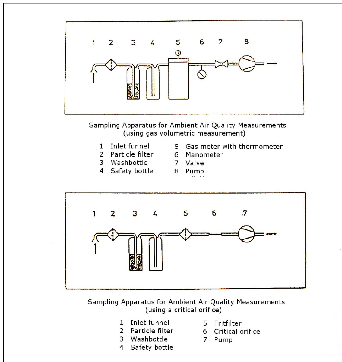
Figure 9: Sampling Apparatus for Ambient Air Quality Measurements
