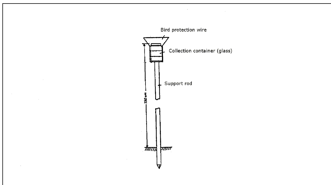
Figure 16: Bergerhoff Sampler
