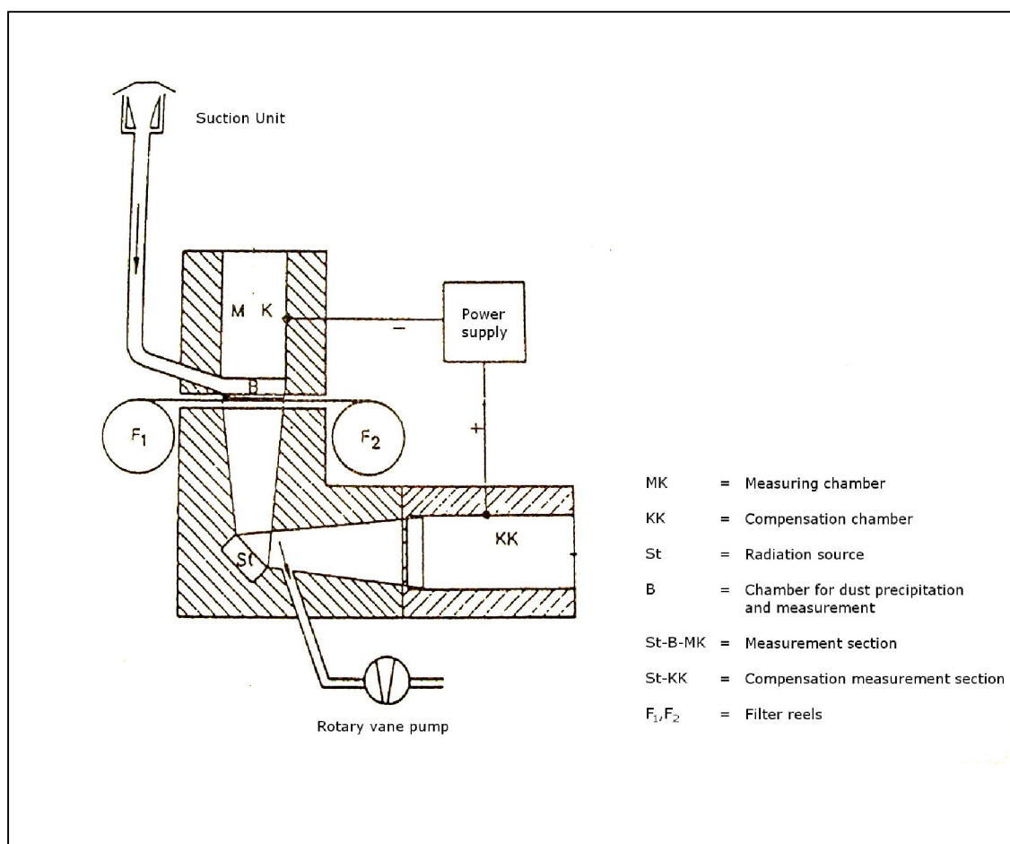
Figure 8: Suspended Particulate Matter Measurement with Beta-Ray Absorption
