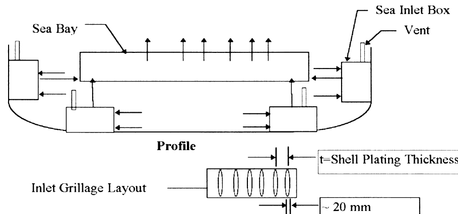
Typical Sea Cooling System Schematic on Russian Icebreakers
