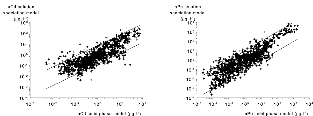
Figure 6 Comparison of metal concentrations of Cd an Pb calculated with the Dutch C-Q transferfunctions and measured concentrations
