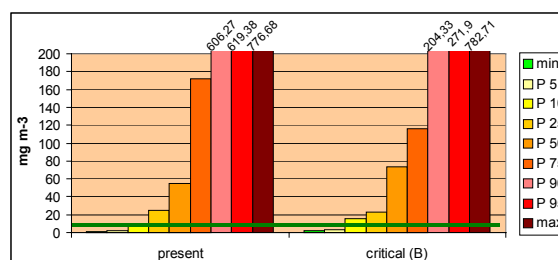
Figure 1 a-d: Distribution of calculated present and critical concentration of cadmium and lead in soil solution for two types of ecosystems.
