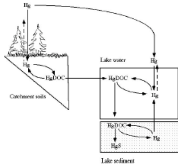
Figure 4: Mass flow diagram for the transfer of mercury from deposition to fish in lakes. In the soil, mercury very rapidly adsorbs to organic matter. In the lake a number of processes occur. Mercury is transported there mostly as bound to dissolved organic matter and organic matter particles. In the lake, fast cycles transfer organically bound to methylated and back to organically bound. A majority of the mercury remain as bound to organics. A significant amount sedimentates to the bottom where a significant fraction will remain buried. Under anoxic conditions, mercury will be precipitated as mercury sulfide. This is very stable and can be seen as a permanent storage.
