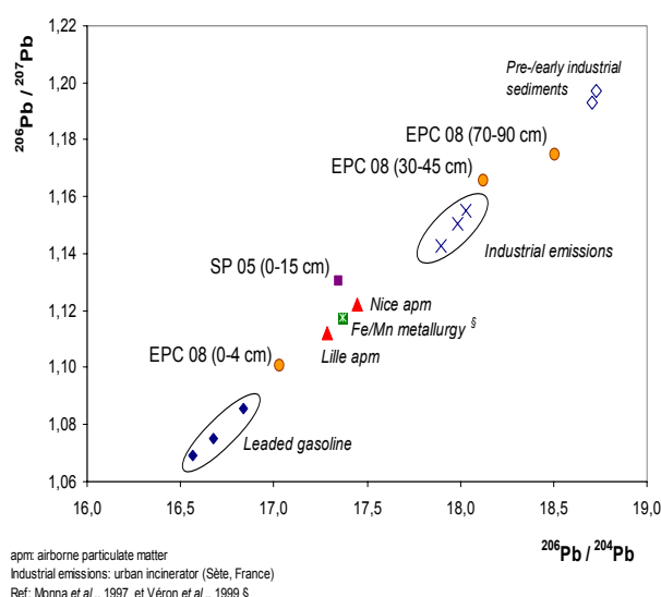
Figure 3. Pb isotopic composition diagram ( 206 Pb/ 207 Pb vs. 206 Pb/ 204 Pb) for EPC 08 profile and SP 05 surface horizon
