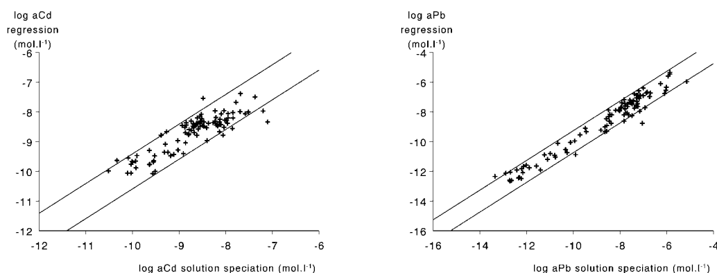
Figure 7 Comparison of metal activities of Cd an Pb calculated with the UK a-Q transferfunctions (table ..)and activities calculated from soil solution speciation (Model VI)
