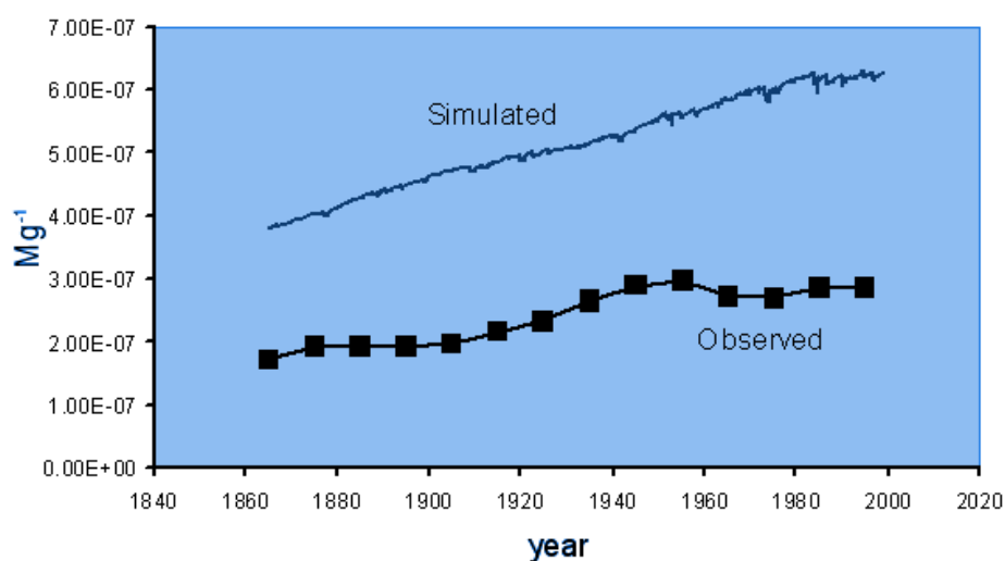
Figure 1. Simulated and observed concentrations of Cu in ^{210}\text{Pb} dated Lochnagar sediments.
