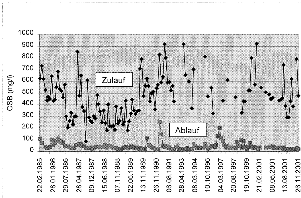
Abb. 4.6: CSB Anlage See
