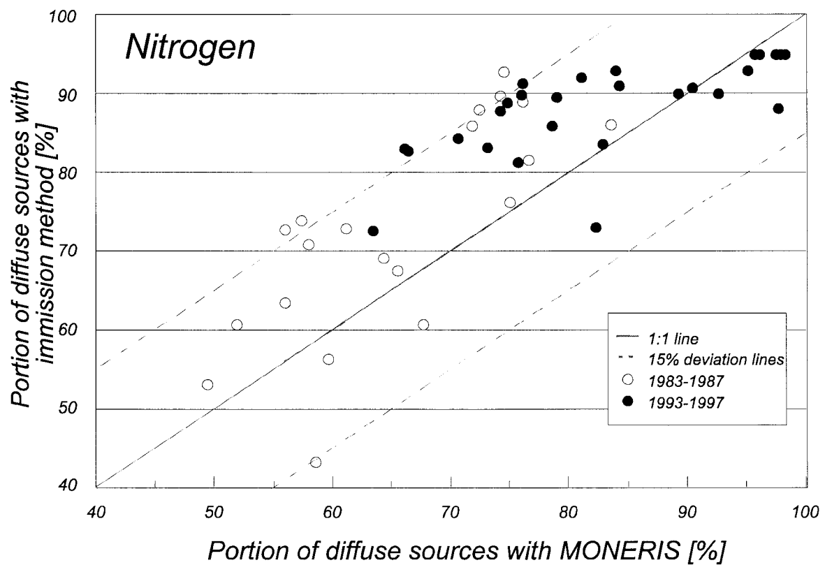
Figure 4.24: Comparison of the proportion of diffuse inputs of phosphorus and nitrogen estimated with the immission method and with MONERIS.
