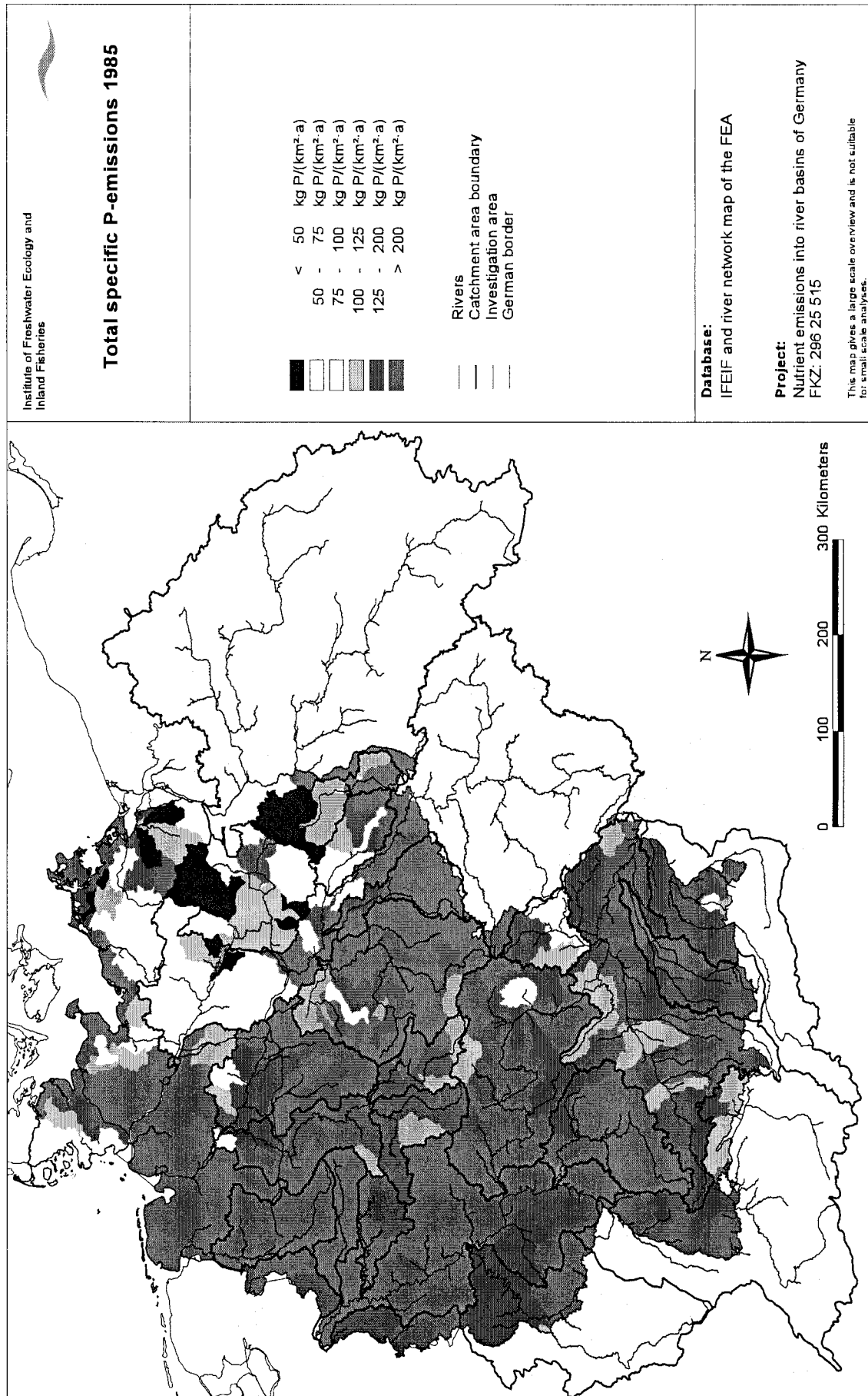
Map 4.23: Total specific P-emissions 1985.
