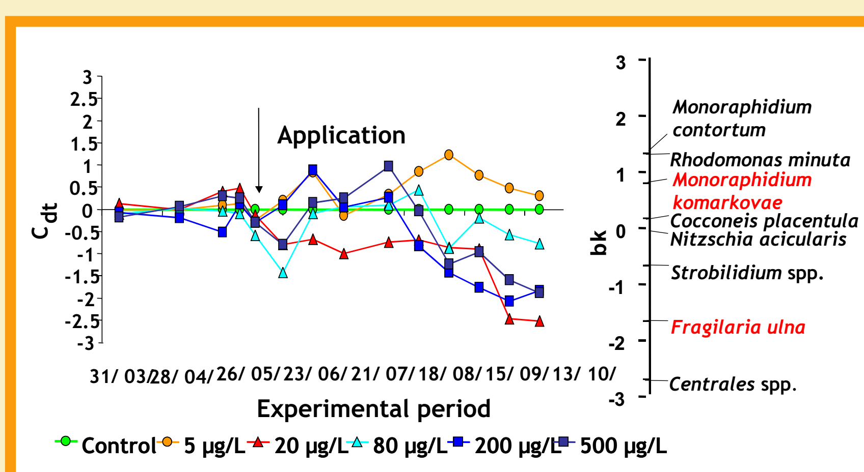
Fig. 4: PRC-analysis of the reduced phytoplankton data set in the stream mesocosms. Of total treatment variance (21.1 %), 30.5 % is explained by the PRC diagram. Species weight = bk value, arrow indicates date of application.
