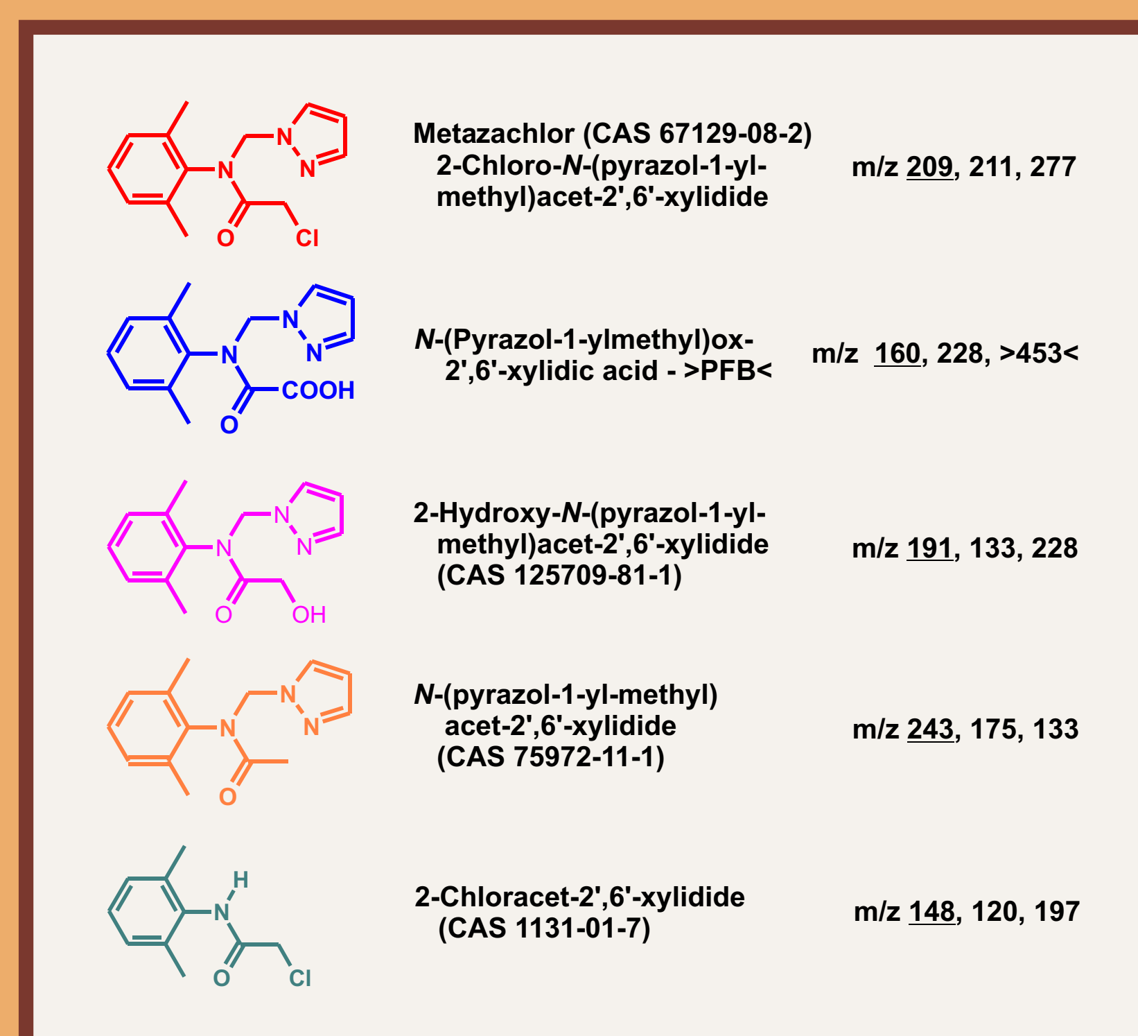
Fig. 3: Metazachlor and analyzed metabolites
