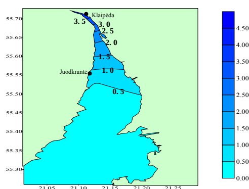
Fig. 4 Long-term distribution of the surface water salinity in the Curonian Lagoon
