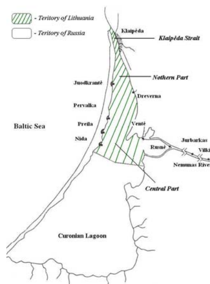
Fig. 1 Curonian Lagoon scheme
