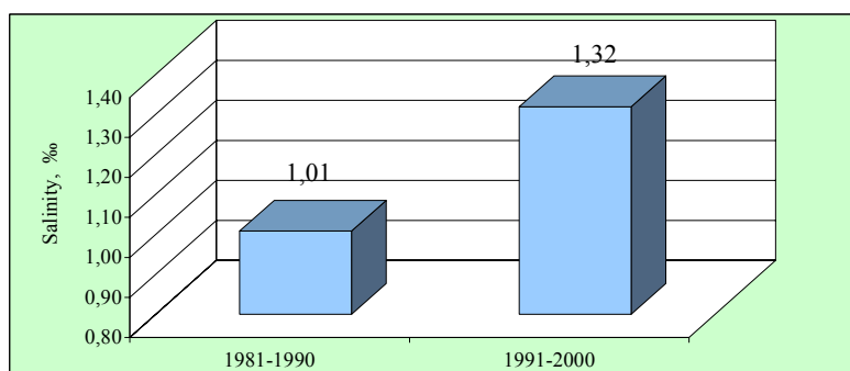
Fig. 6 The mean water salinity during the periods of 1981-1990 and 1991-2000 near Juodkrante
