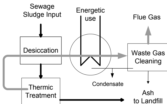
Figure 18 Sewage sludge incineration with separated drying and combustion
