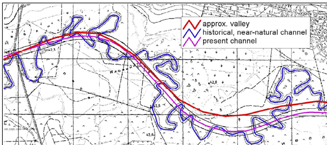
Figure 8: Scheme of morphological alteration (Example: Osam River)
