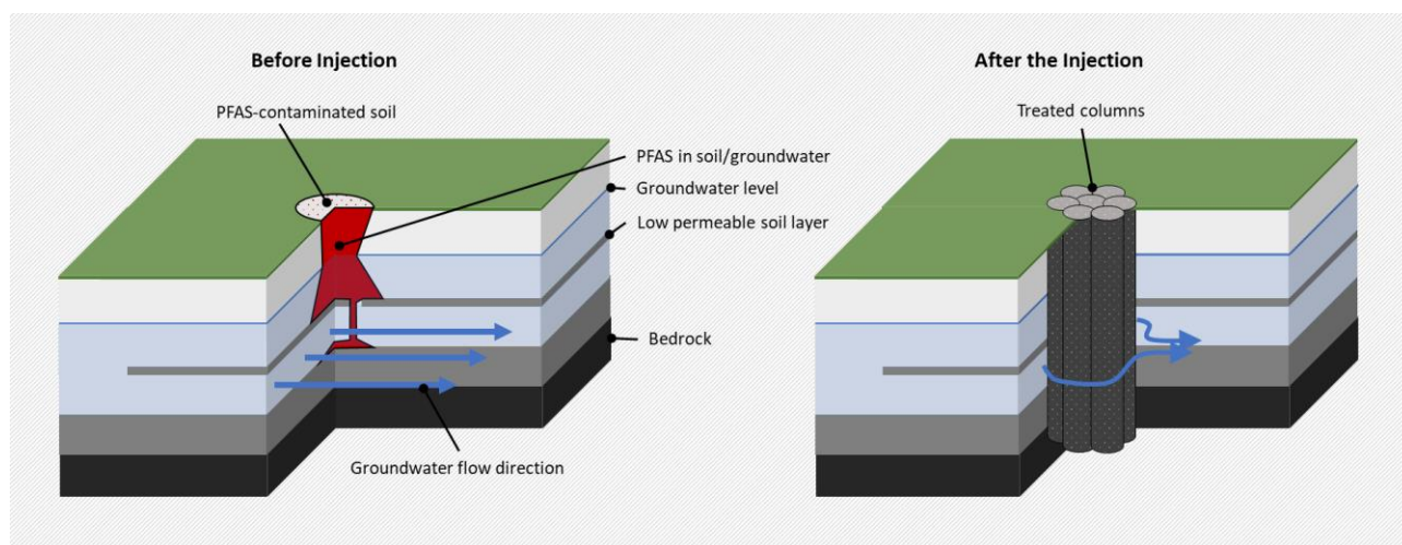
Figure 28 Principle of the In-Situ-Soil-Mixing-Technology
