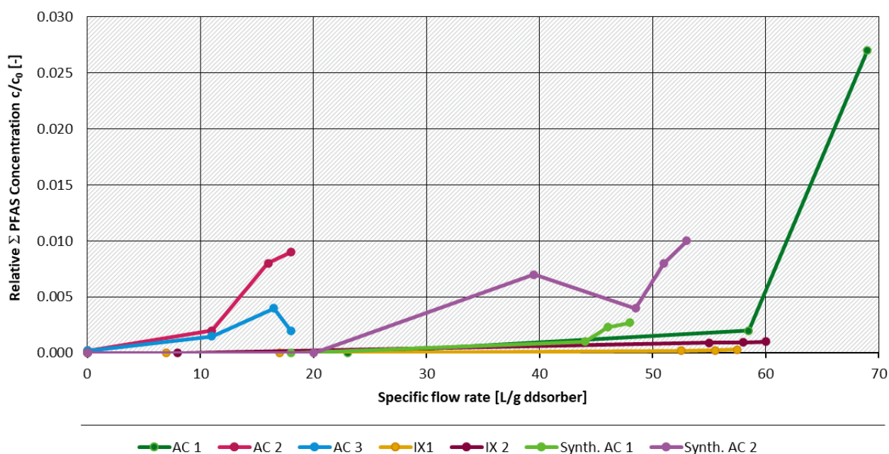
Figure 6 Breakthrough curves of different sorption materials (AC = activated carbon, IX = ion exchanger)
