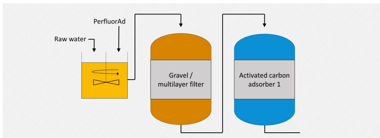
Figure 13 PerfluorAd®-Process scheme
