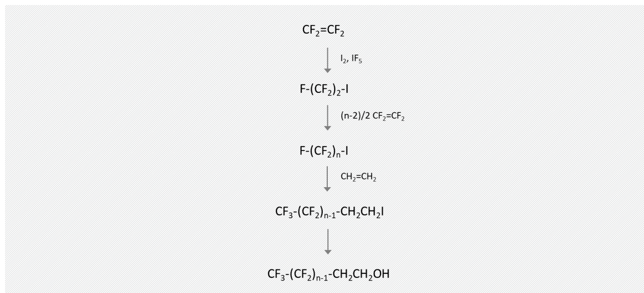
Figure 2 Telomerization
