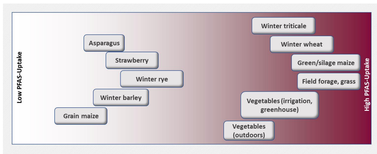
Figure 38 PFAS uptak through various crops
