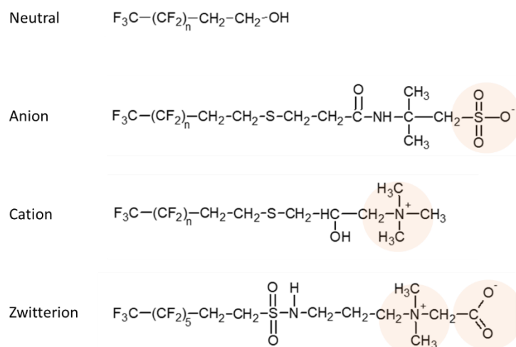
Figure 5 Examples of differently charged precursors
