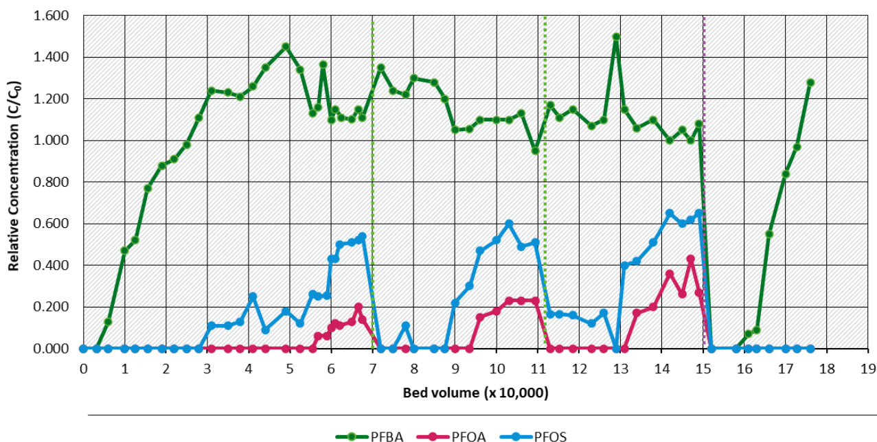
Figure 7 Breakthrough curves for various PFAS compounds
