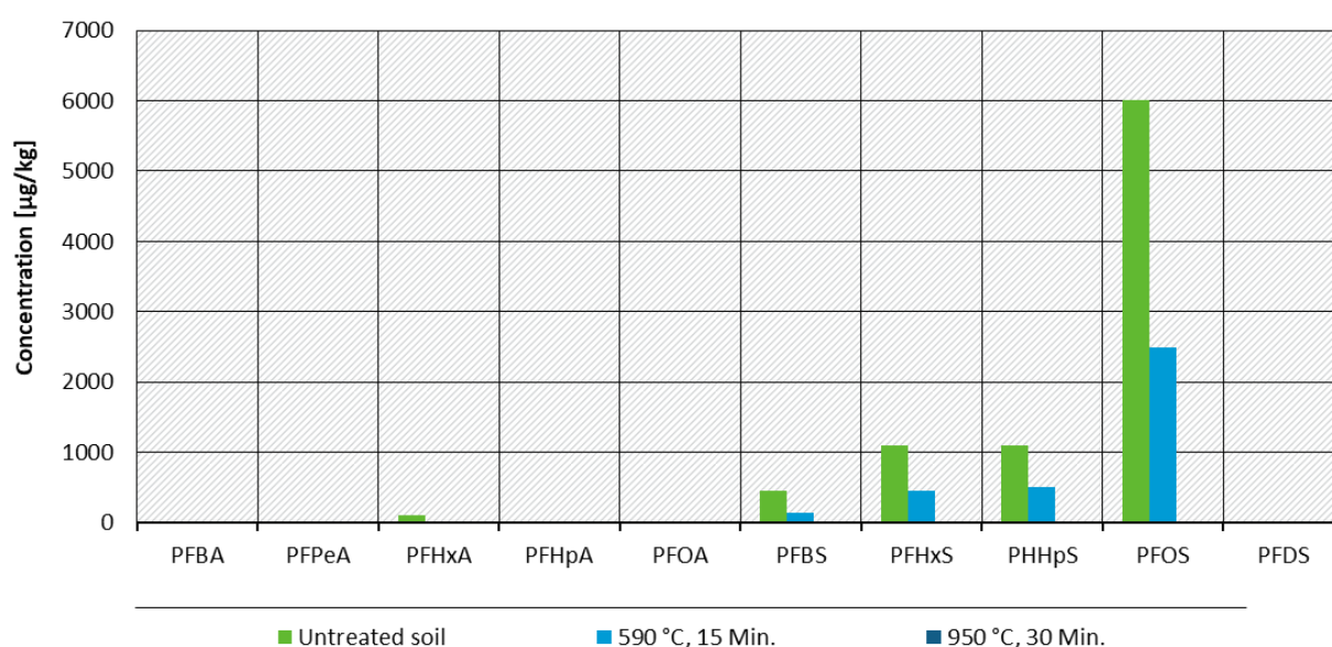
Figure 27 Results of the thermal desorption at 590 °C and 950 °C
