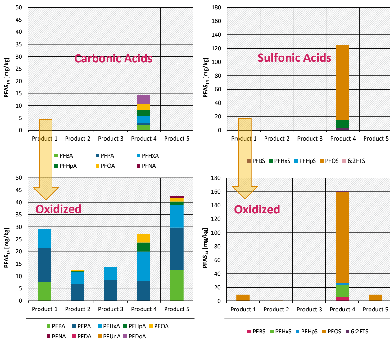
Figure 43 Formation of perfluoroalkane acids out of AFFF
