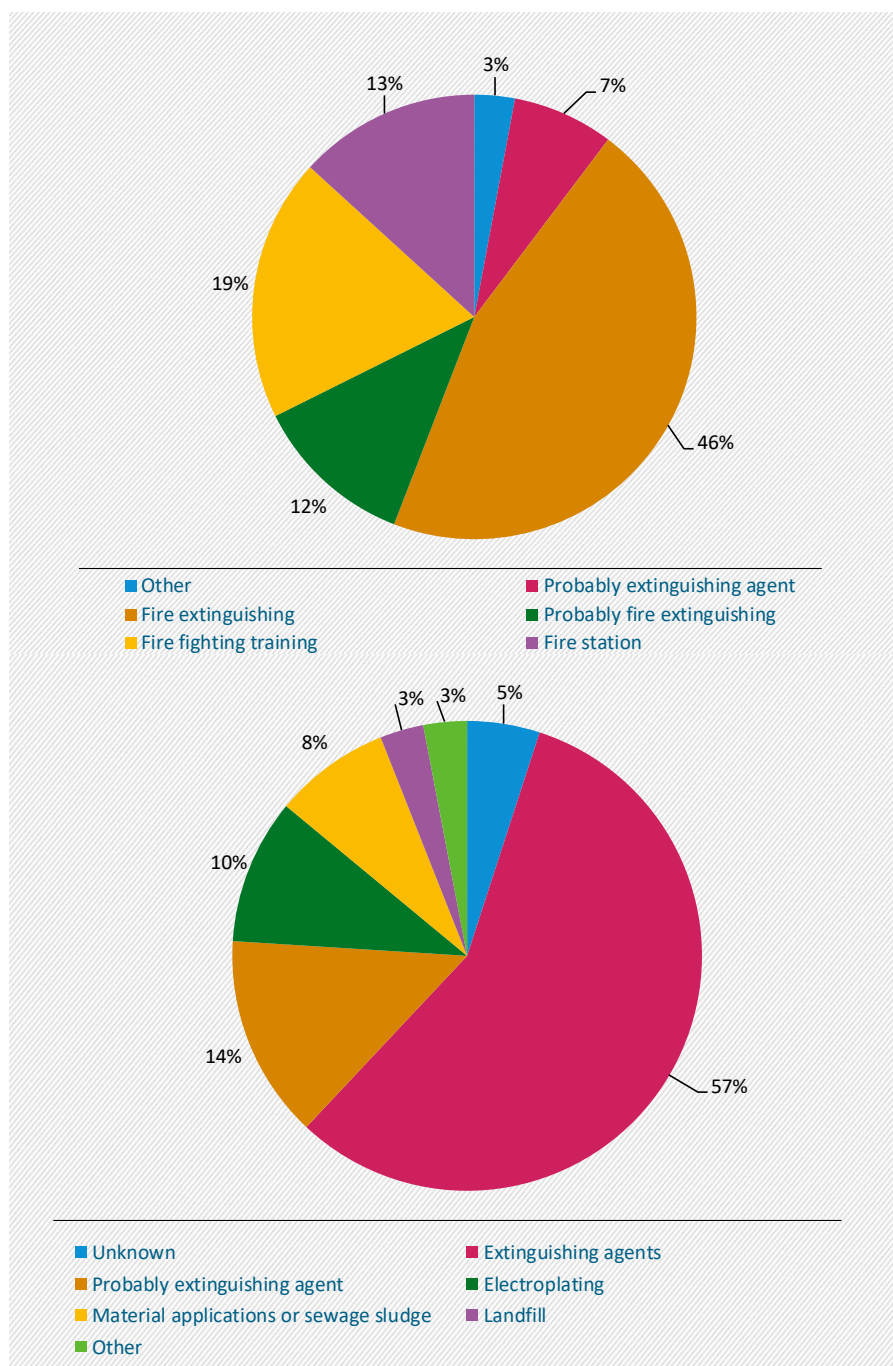
Figure 50 PFAS cases in Northrhine Westphalia (status: 04/2017) according to causes (top, n = 93) and extinguishing agent differentiated (bottom, n = 66)
