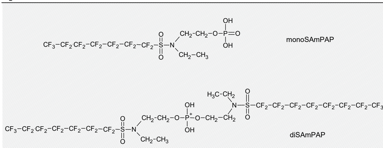
Figure 47 Chemical structure of SAmPAP
