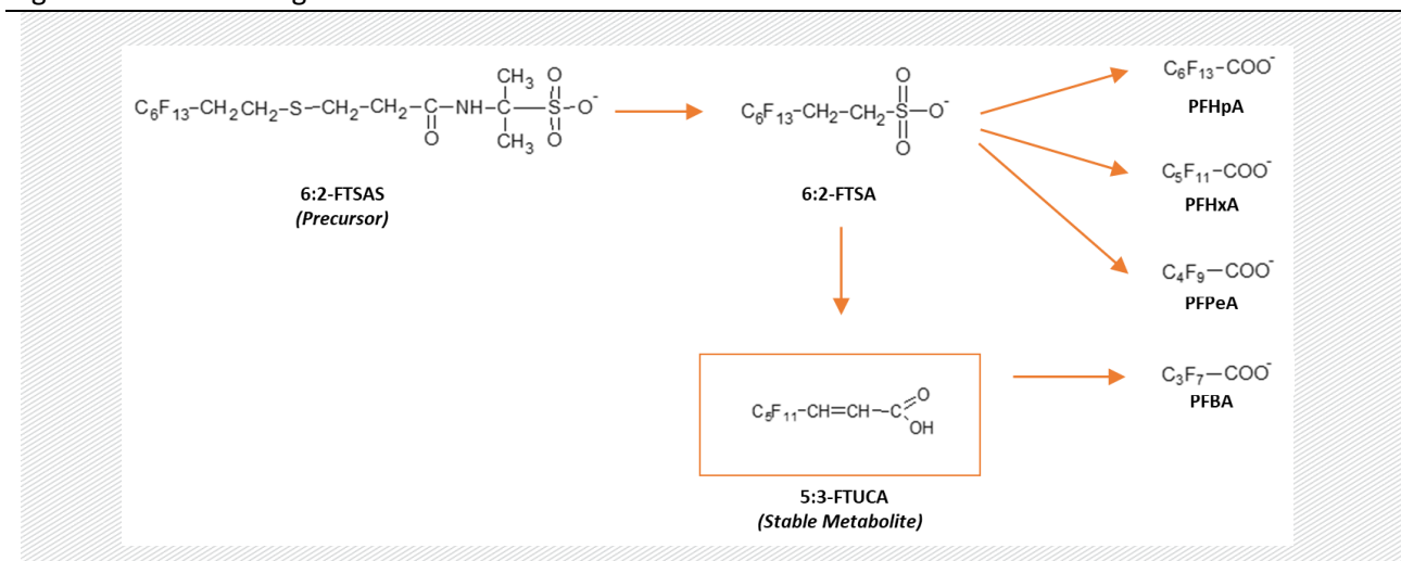
Figure 34 Degradation of 6:2-FTSAS
