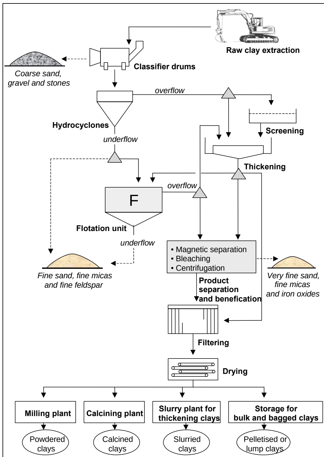
Figure 3.54: Typical kaolin process flow sheet [40, IMA, 2002]
