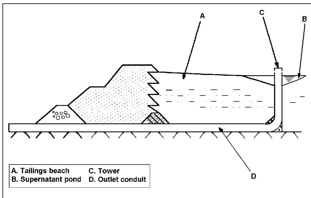
Figure 2.43: Tower decanting system [8, ICOLD, 1996]
