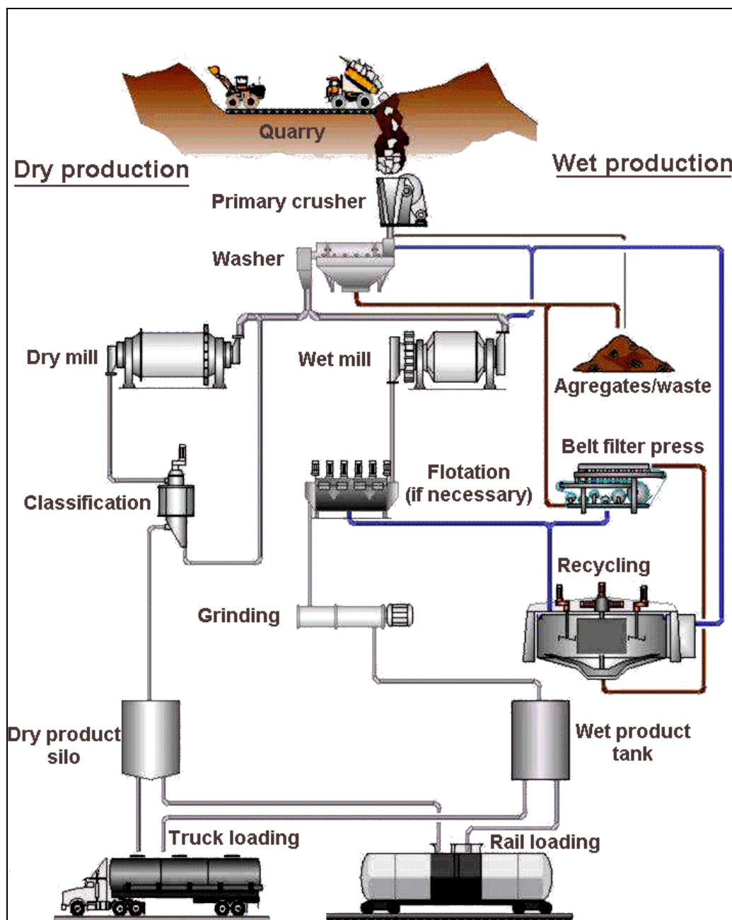
Figure 3.56: Calcium carbonate process flow sheet [42, IMA, 2002]
