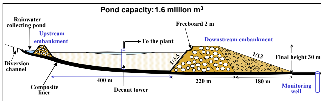
Figure 3.37: Cross-sectional drawing of Ovatic tailings pond [56, Au group, 2002]
