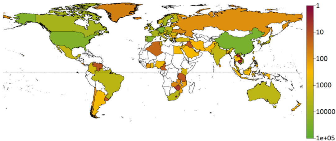
Figure 3: Global distribution of MEC values published until 2020
