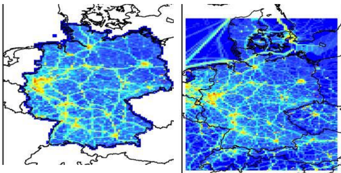
Figure 26 RegridDED NO x emissions 2005 Germany by IER / IZT (left) and TNO PAREST default (Right)
