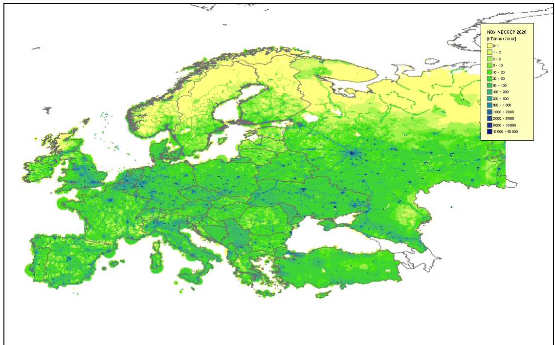
Figure 1 Distribution of \text{NO}_x emission in 2020 according to NEC6_current_policy (Table 2).
