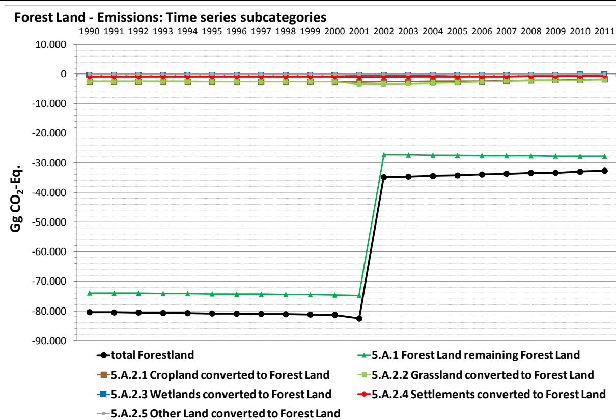
Figure 51: Greenhouse gas emissions [Gg CO 2 -eqs.] from forest land, as a result of land use and land-use changes, 1990 – 2011, by sub-categories
