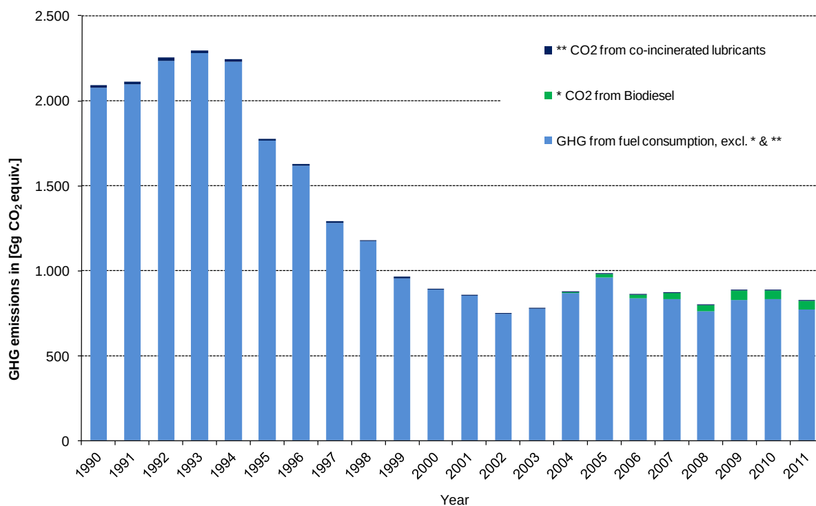
Figure 33: Development of greenhouse-gas emissions in inland shipping, 1990 – 2011
