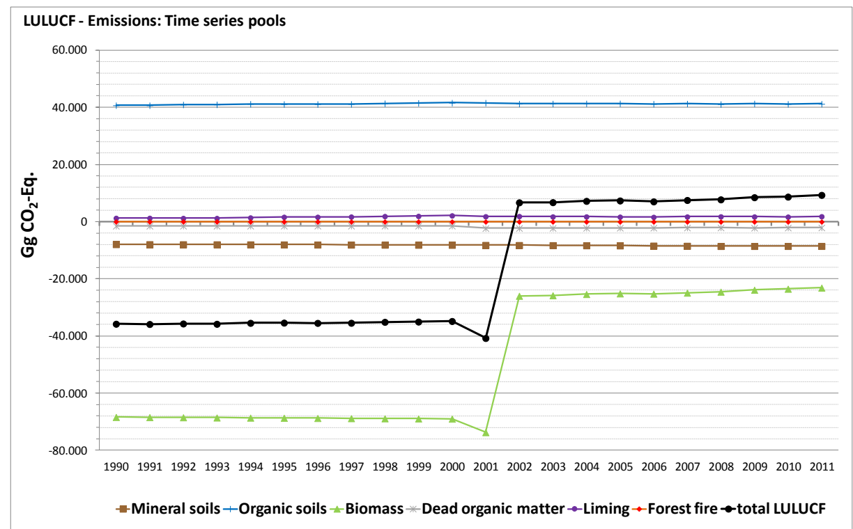
Figure 47: Time series for greenhouse-gas emissions and sinks [Gg CO 2 equivalents] in the LULUCF sector since 1990, differentiated by source categories
