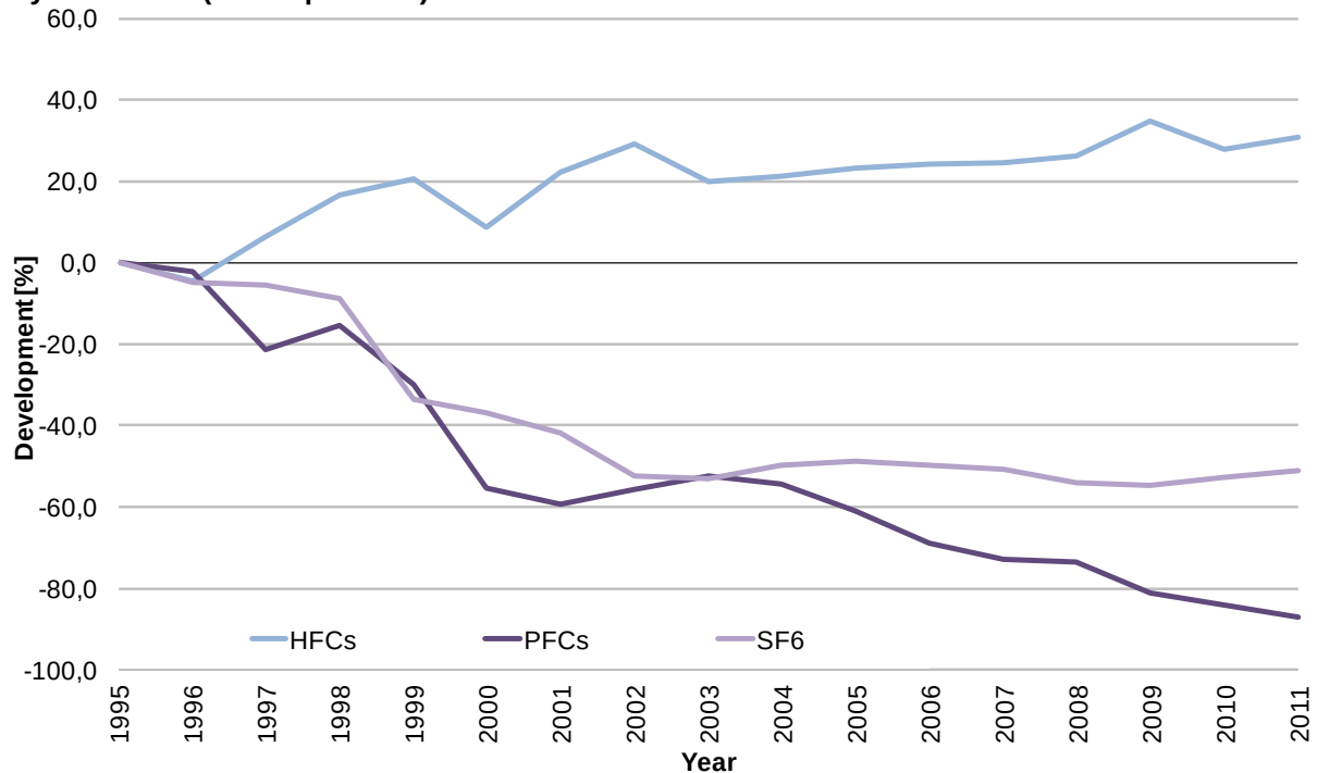
Relative development of F-gas emissions since 1995, by substance (CO 2 equivalent)
