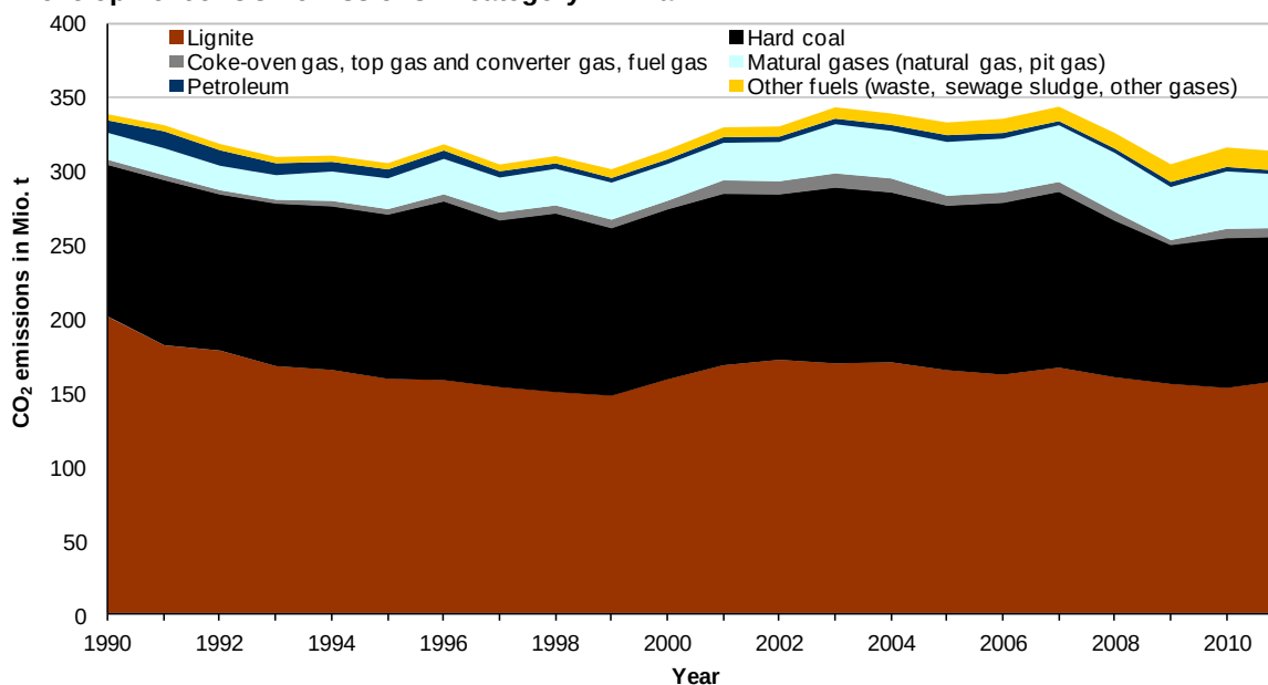
Figure 26: Development of CO 2 emissions in source category 1.A.1.a
