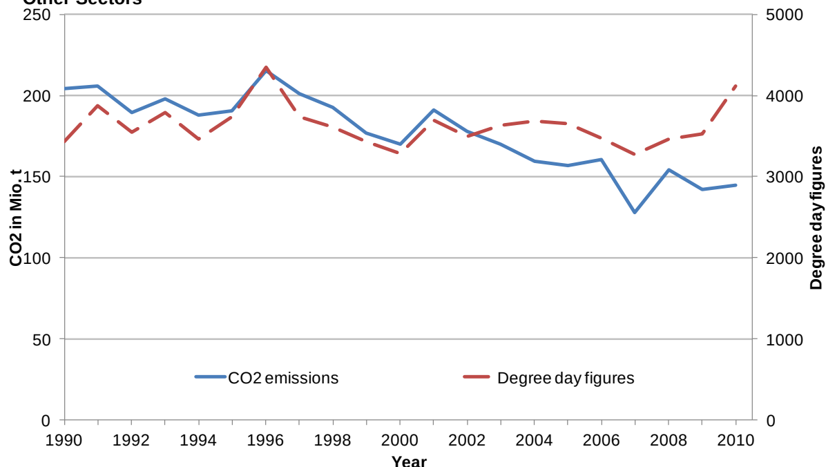
Figure 34: Change in total emissions of 1.A.4, as a function of temperature
