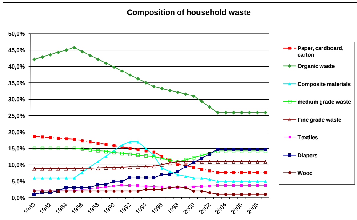
Figure 69: Trends in waste composition (old German Länder) between 1980 and 2009
