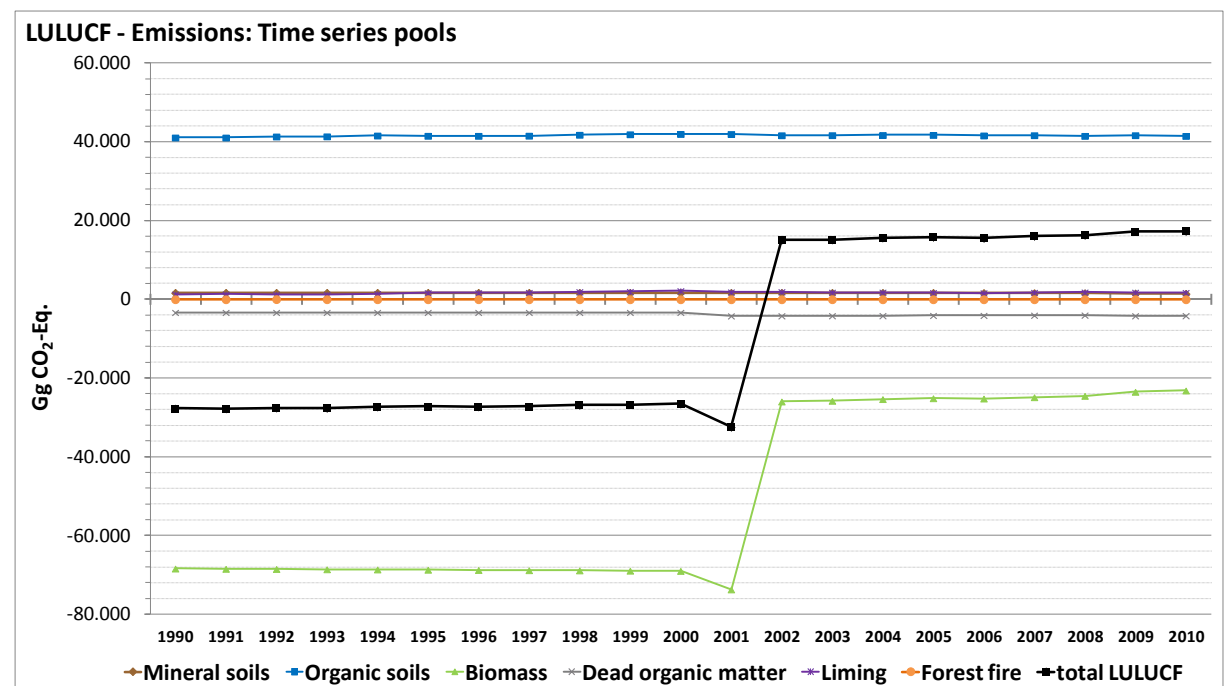
Figure 48: Time series for greenhouse gas emissions and sinks [Gg CO 2 equivalents] in the LULUCF sector since 1990, differentiated by source categories
