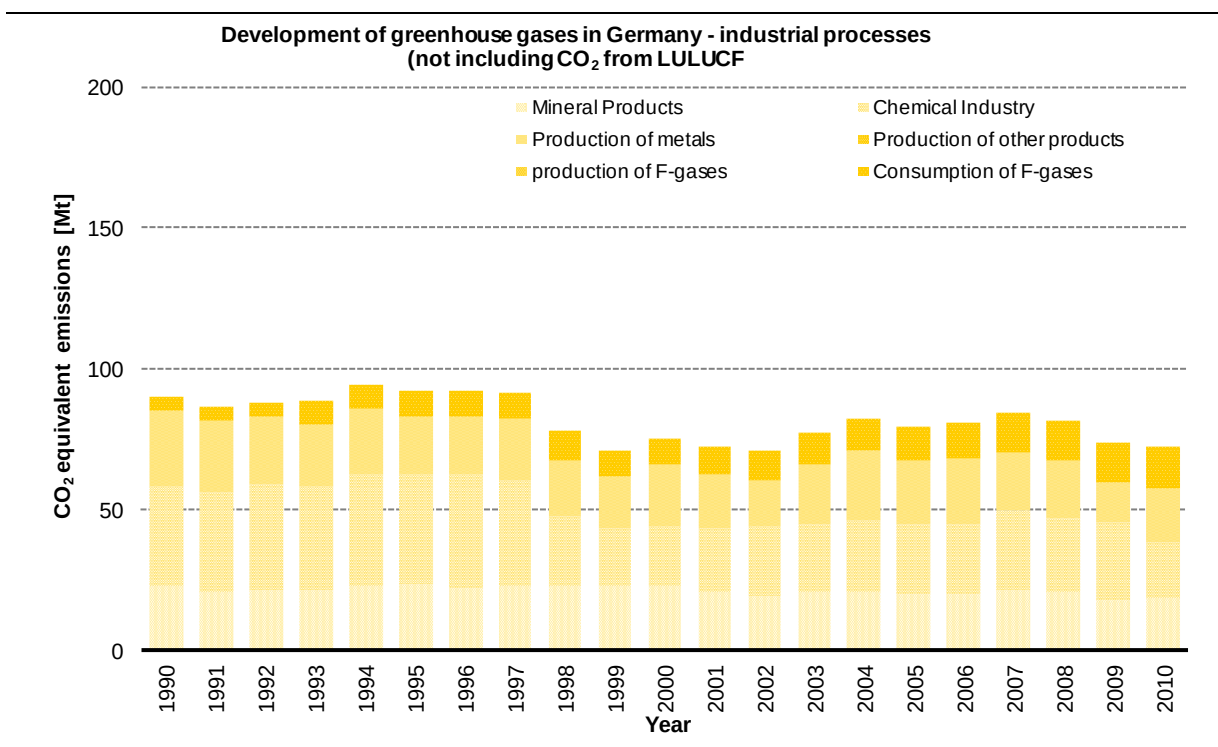
Figure 41: Overview of greenhouse-gas emissions in CRF Sector 2
