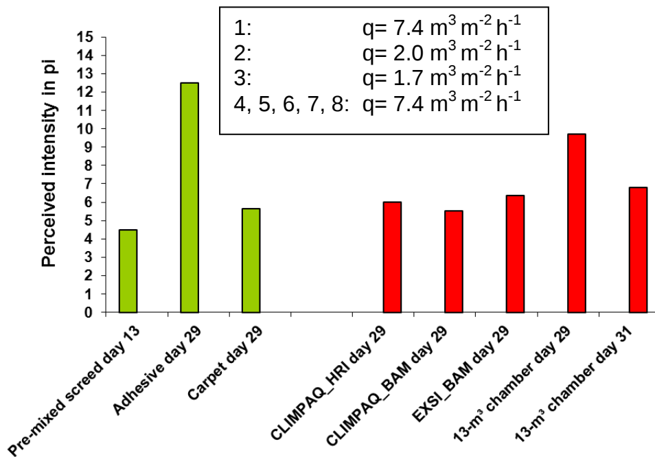
Figure 5-42: Test results for a combination of building products (pre-mixed screed, floor covering adhesive, wall-to-wall carpet)
