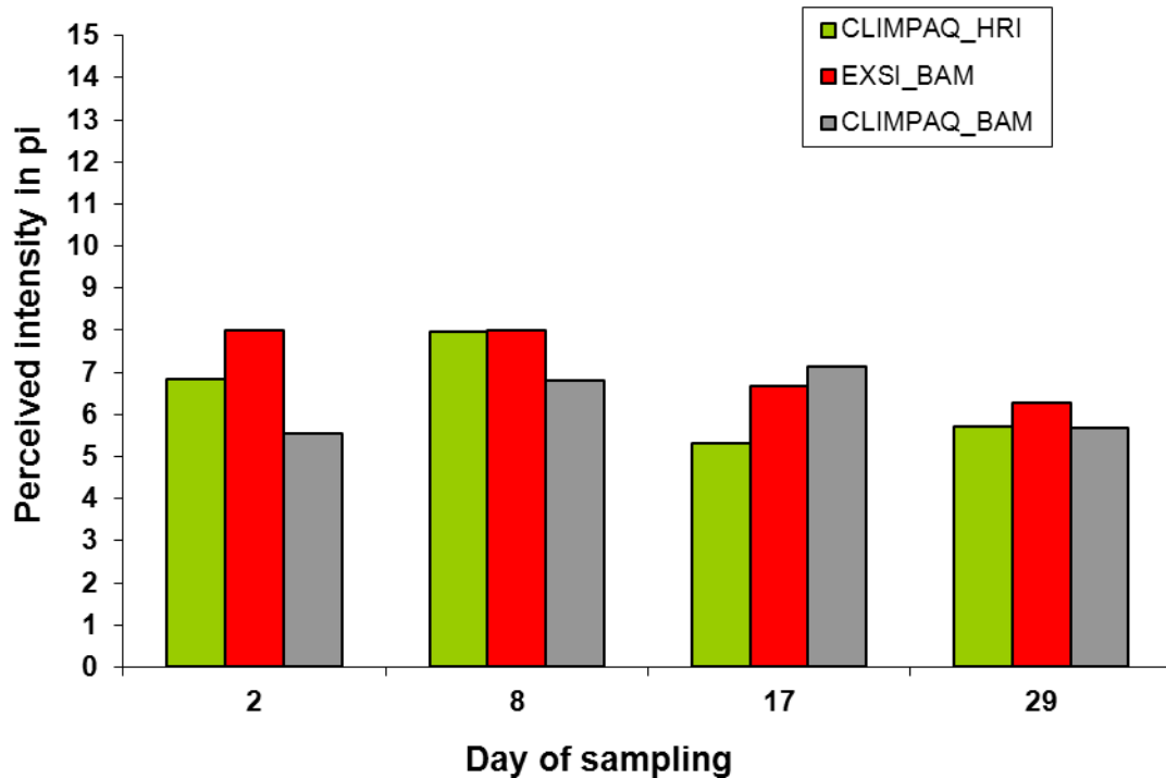
Figure 5-29: Comparison of the results of intensity tests in different emission chambers (PVC floor covering No. 4101)
