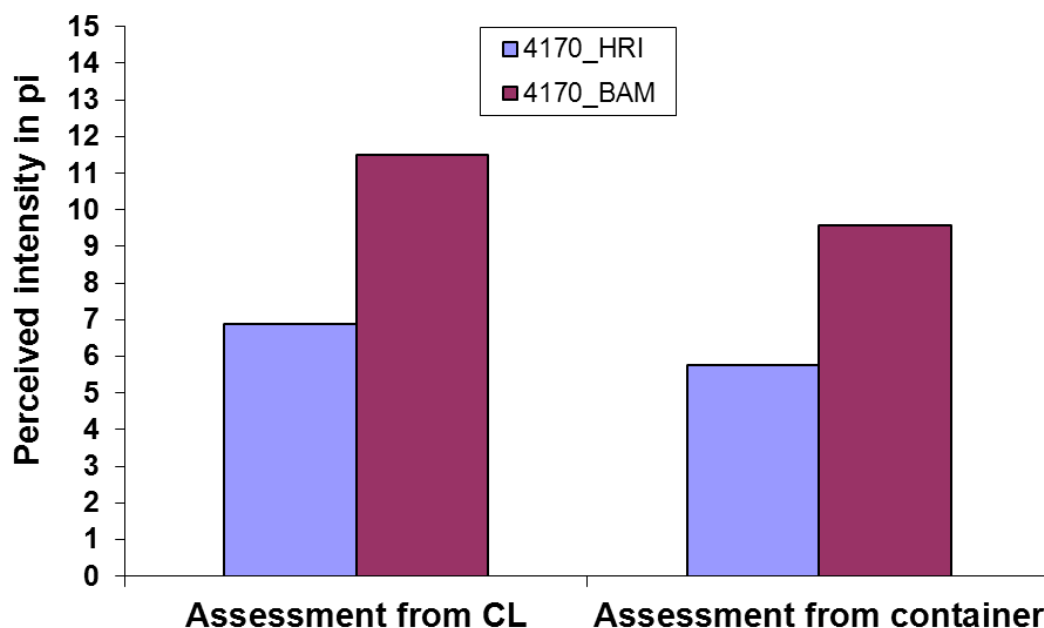
Figure 5-33: Comparison between assessments from CLIMPAQ and Tedlar containers® for product PVC 4170
