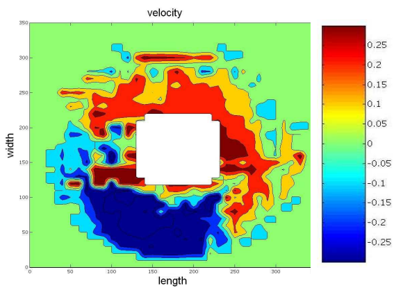
Figure 5-34: Flow profile in the 24-litre chamber
