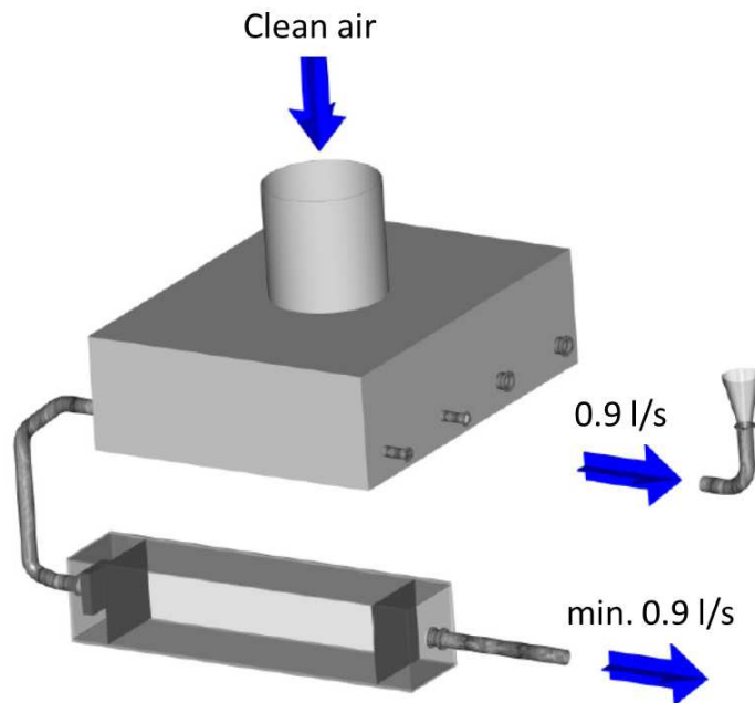
Figure 4-2: Air circulation in CLIMPAQ
