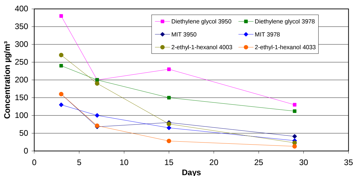
Figure 5-22: Concentration of some typical VOC as a function of time from floor covering adhesives
