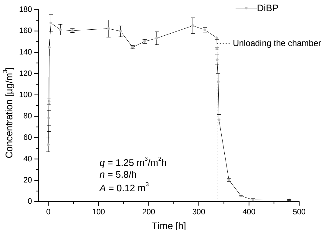
Figure 5-16: DiBP concentration from PVC floor covering 4004 as a function of time. 24-litre chamber test [38]
