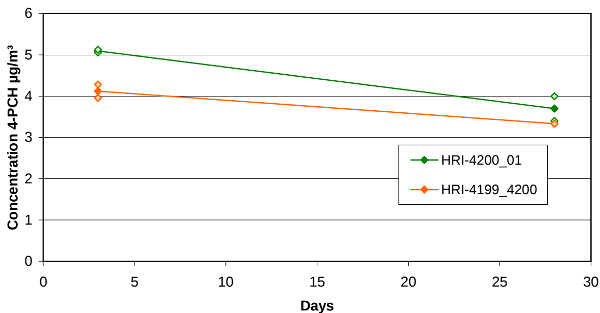
Figure 5-49: 4-PCH concentrations for product combinations in HRI's CLIMPAQs
