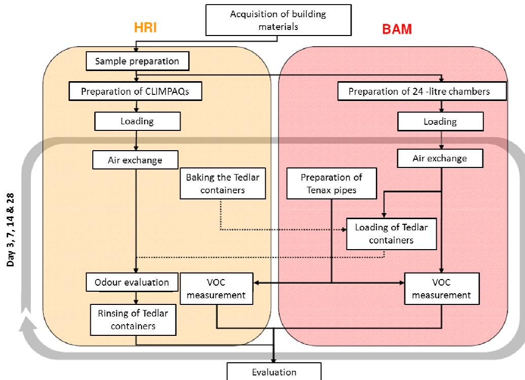
Figure 4-1: Measurement flowchart
