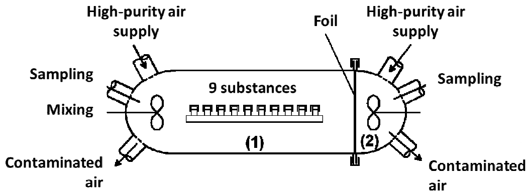
Figure 4-24: Layout of the experimental setup to investigate the permeation behaviour of polymer foils
