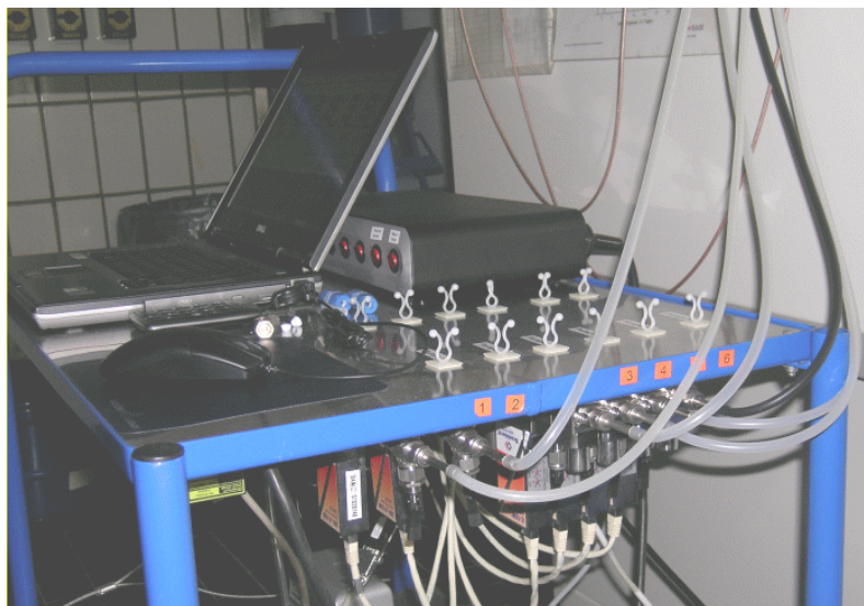
Figure 4-22: Pump trolley used for sampling at the emission test chamber
