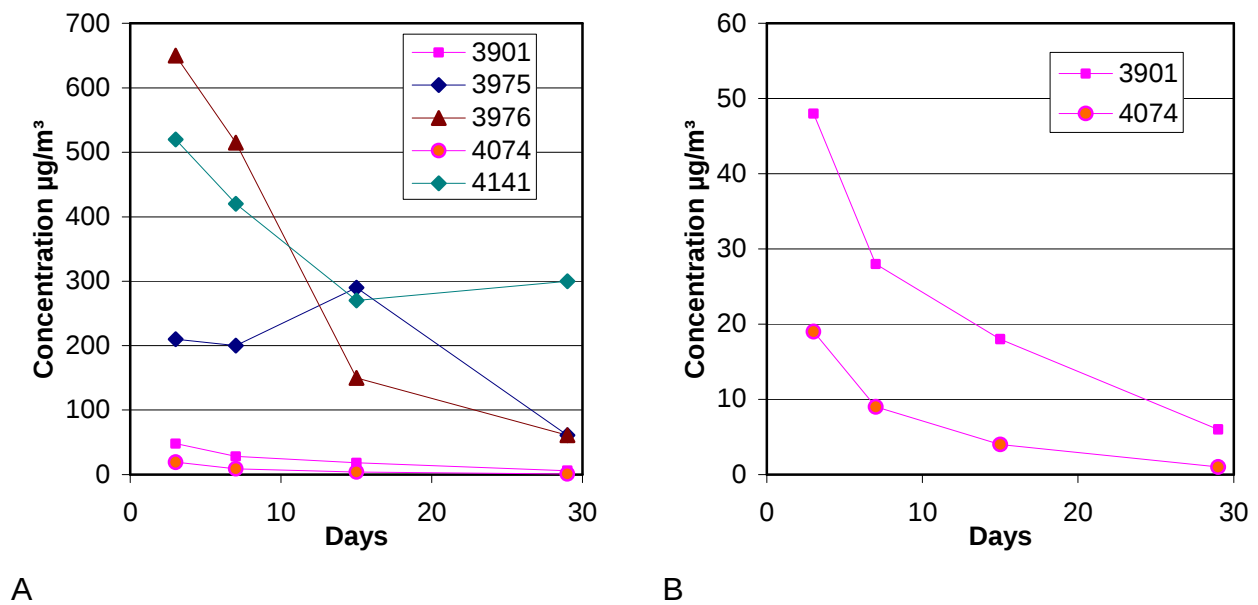
Figure 5-11: A: Concentration of 4-PCH as a function of time from five different textile floor coverings, B: Details for two low-emitting textile floor coverings
