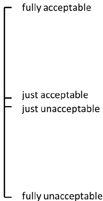
Figure 3-5: Acceptance scale
