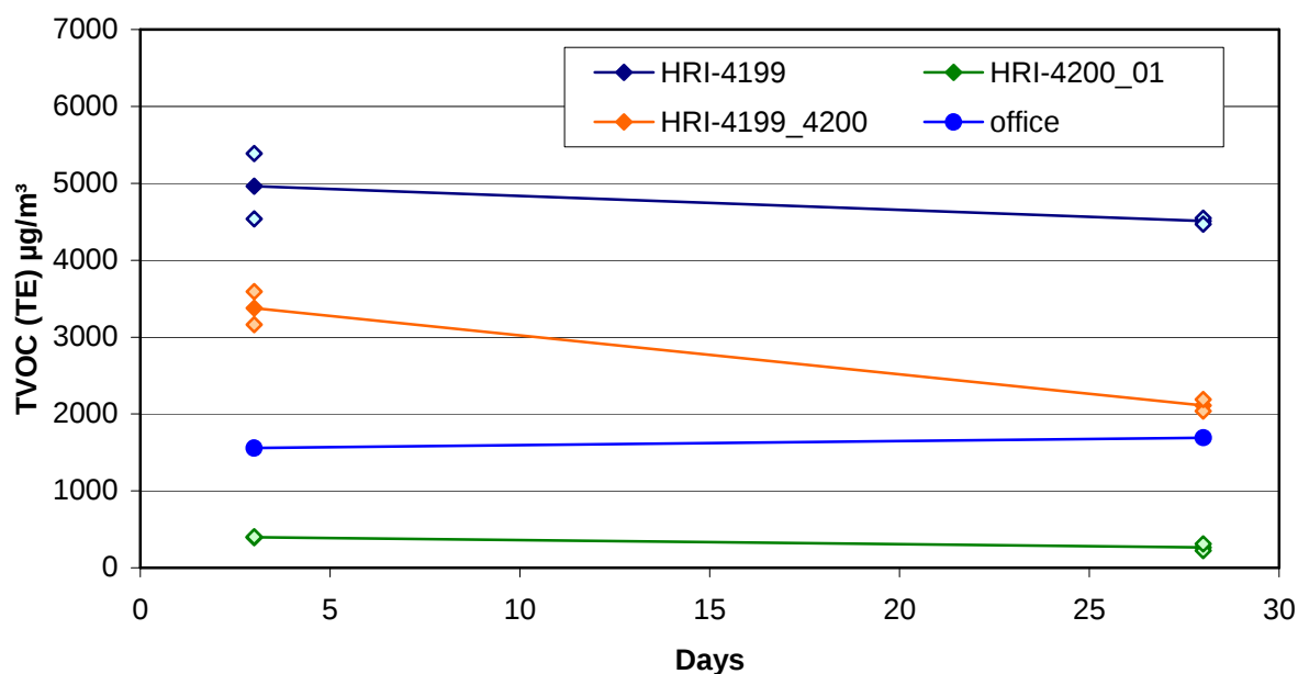
Figure 5-48: Results of combination tests in HRI's CLIMPAQs. Floor covering No. 4199 was placed into an office. TVOC values are given as toluene equivalents (TE).
