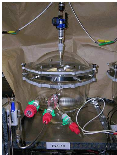
Figure 4-4: 24-litre chamber
