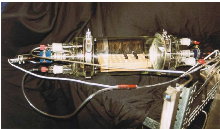
Figure 4-25: Test equipment to investigate the permeation behaviour of polymer foils
