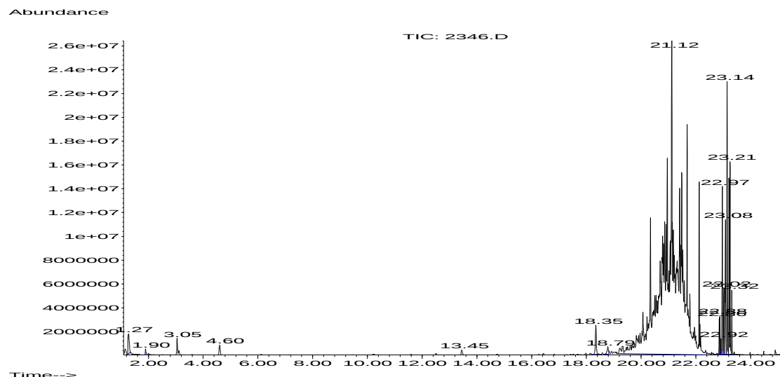
Figure 5-47: Chromatogram of PVC floor covering No. 4199 in HRI's CLIMPAQ on day 29
