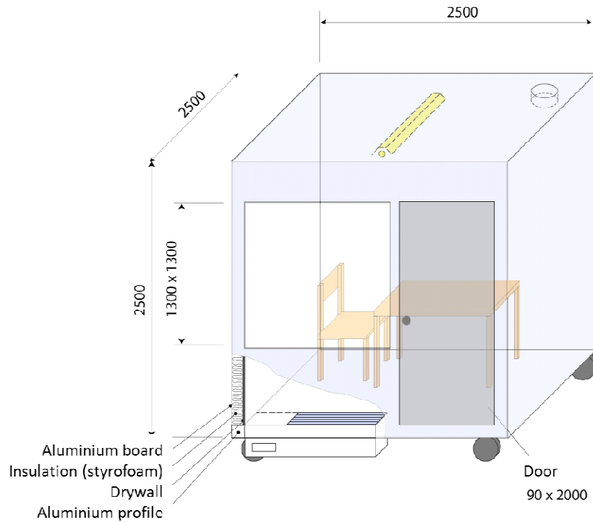
Figure 4-9: Scheme of the 13-m 3 chamber
