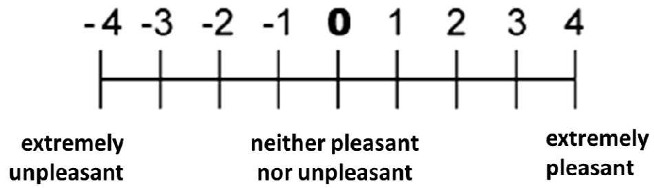
Figure 3-6: Hedonic scale
