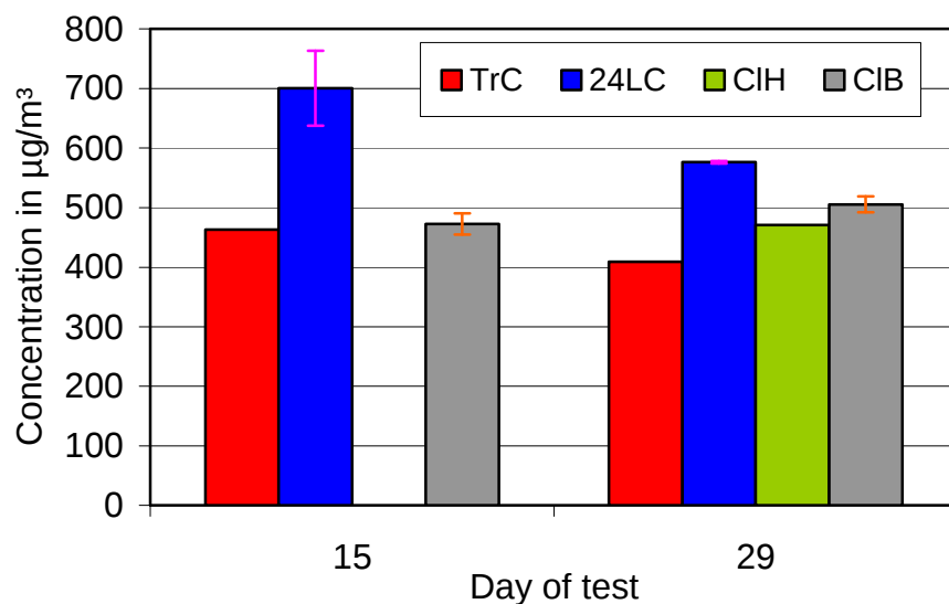
Figure 5-30: Comparison of ethanediol concentrations and up-down bars in different emission chambers (joint seal No. 4026) on days 15 and 29 for multiple tests (TrC: transport container; 24LC: 24-litre chamber; CIH: CLIMPAQ HRI; CIB: CLIMPAQ BAM)
