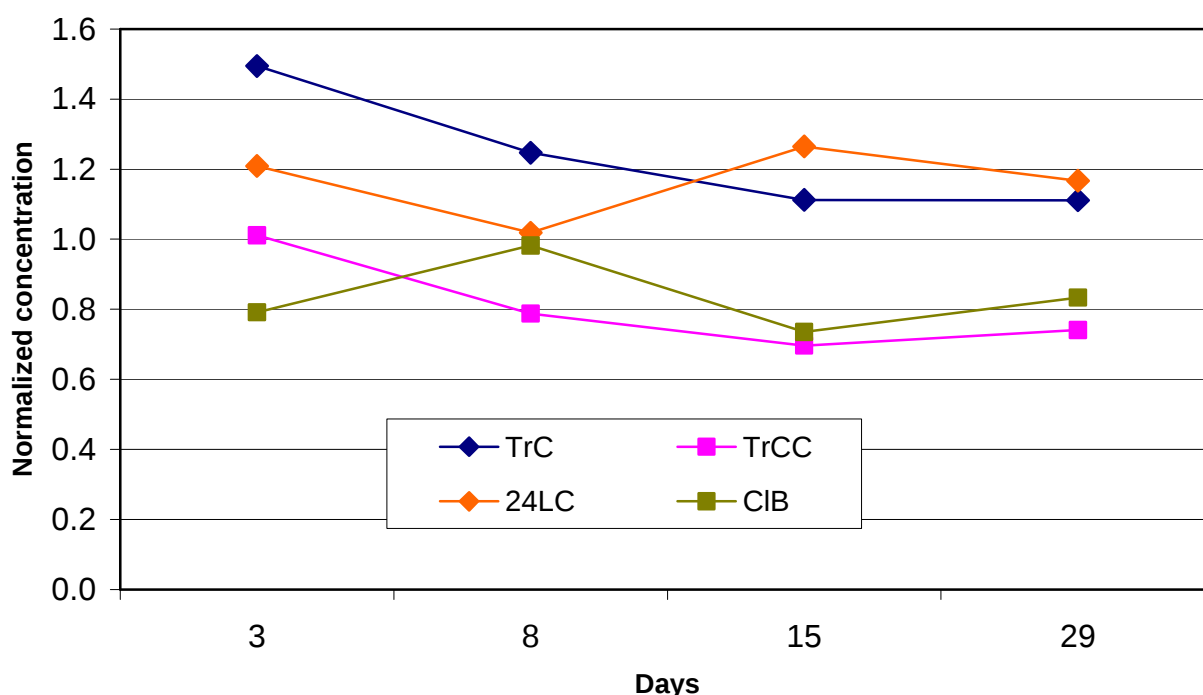
Figure 5-24: Normalized comparison (the mean value of the two chambers equals 1) of the emissions of the chambers compared to the emissions from the transport containers. (TrC: transport container 24-litre chamber; TrCC: transport container CLIMPAQ; CIB: CLIMPAQ BAM)
