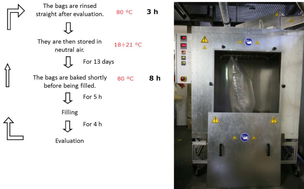
Figure 4-12: Handling of Tedlar® containers and the baking cabinet
