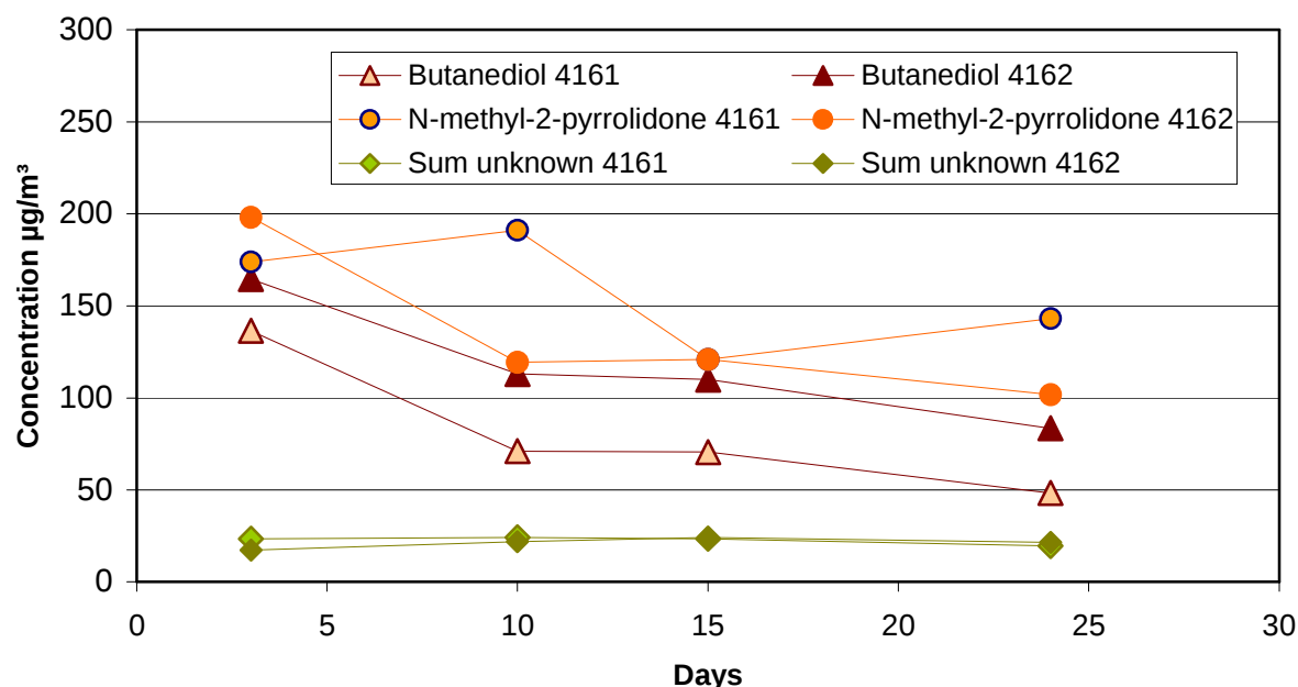
Figure 5-14: Concentration of various VOC from PVC floor coverings 4161 and 4162 over 24 days
