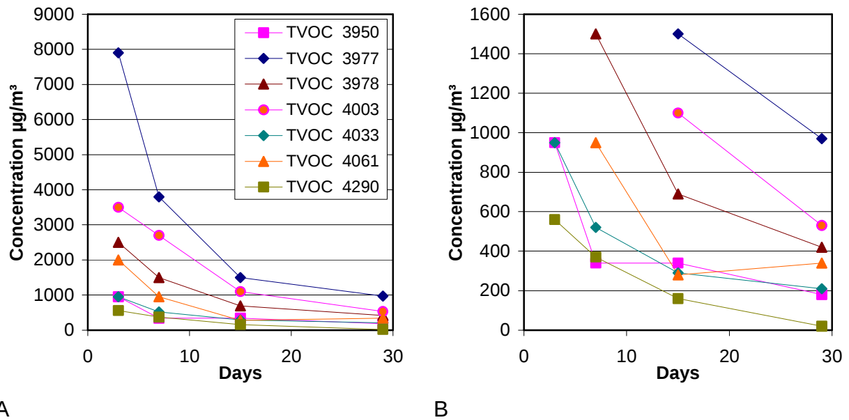
Figure 5-20: TVOC concentration as a function of time for floor covering adhesives tested in the project (Diagram B is an enlargement of an excerpt from A)
