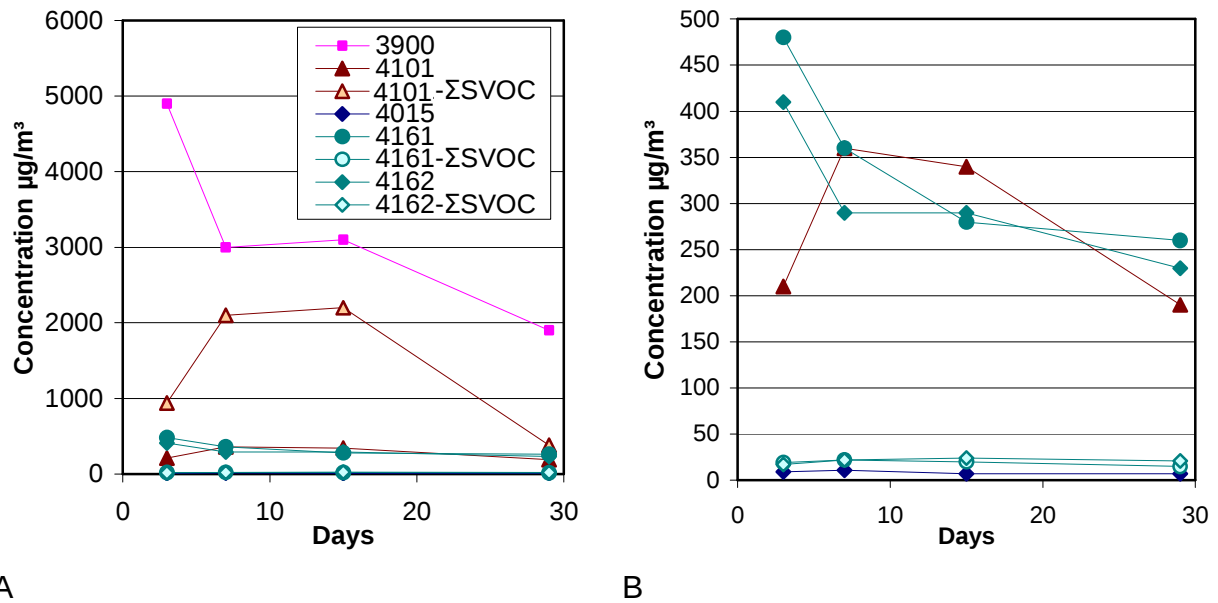
Figure 5-13: TVOC concentration as a function of time for five different PVC floor coverings and SVOC cumulative values for three floor coverings (Diagram B shows details of some data from A)
