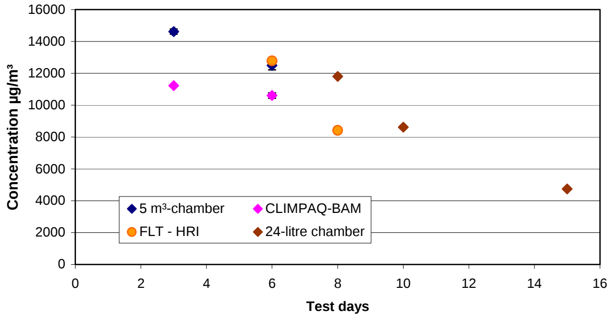
Figure 5-38: Total concentration of unknown VOC ( \Sigma VOC). Measurements simultaneous to direct sensory-based assessments of PVC 4170 at different chamber types
