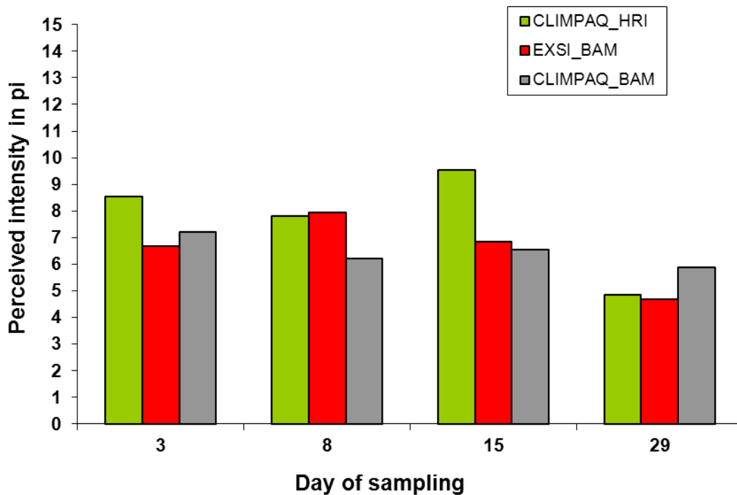
Figure 5-28: Comparison of the results of intensity tests in different emission chambers (joint seal No. 4026)
