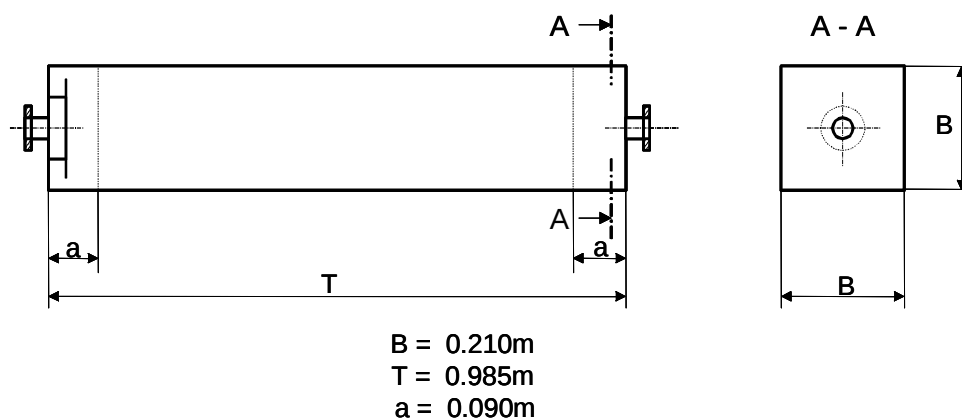
Figure 4-6: Structure of a CLIMPAQ
