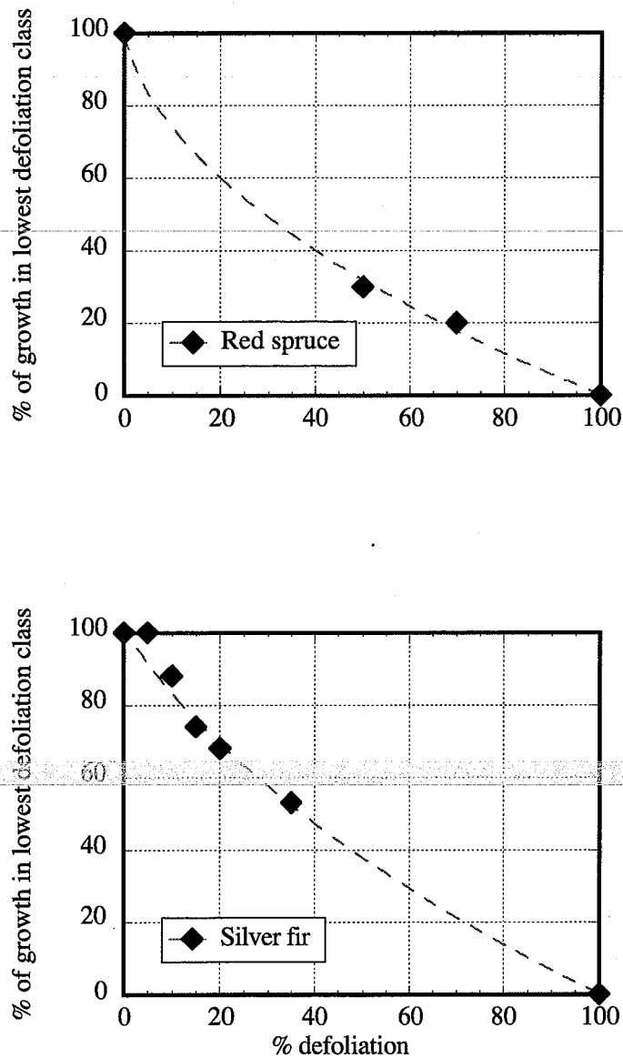
Figure 48: The relation between observed defoliation and stem growth for red spruce ( Picea rubens ), data from Barnard et al., (1989) and Silver fir ( Abies alba ), data from Becker (1991).
