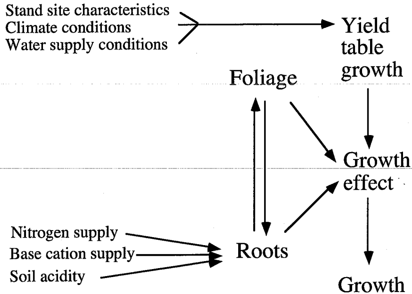
Figure 2: Basic approach to include soil acidity feedback on uptake used in calculations of critical loads in the PROFILE model. The response model used in PROFILE is based on the results presented in this report.
