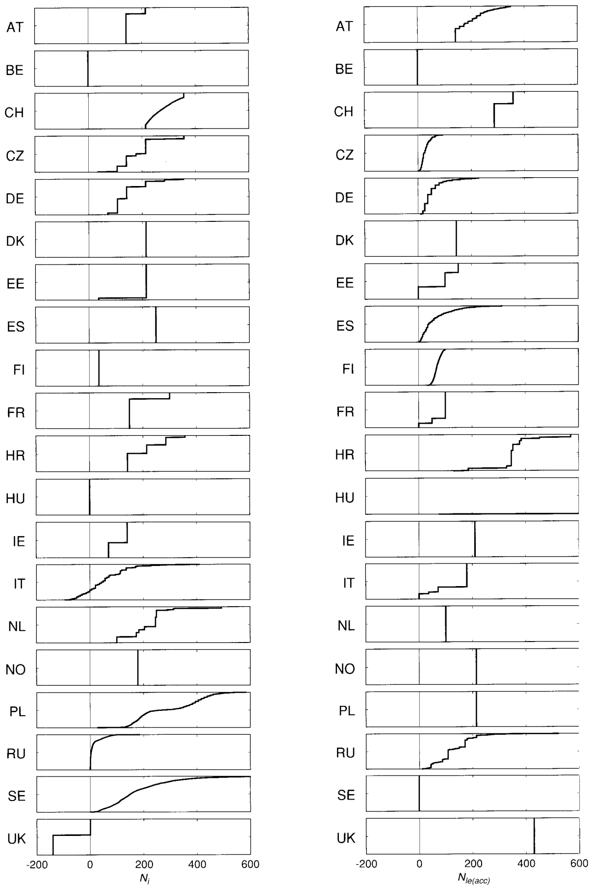
Figure 4-4. Cumulative distribution functions for nitrogen immobilization and acceptable nitrogen leaching (in \text{eq ha}^{-1} \text{yr}^{-1} ) used in the SMB calculations of critical loads for forest soils from national data contributions.
