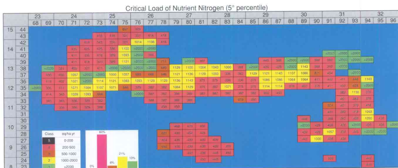
Figure IT-4. Critical load of nutrient nitrogen (5th percentile).
