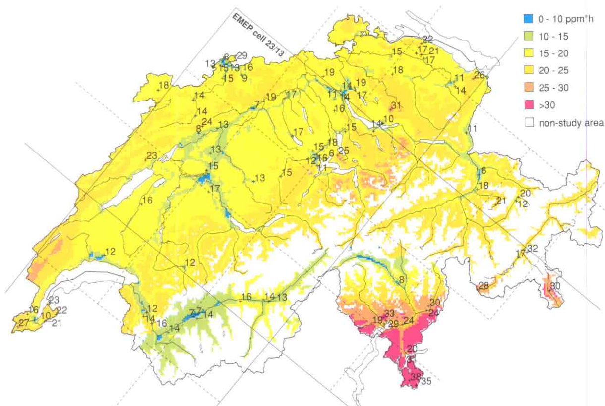
Figure CH-2. Interpolated ozone levels for forests in 1994: accumulated exposure over a threshold of 40ppb for daylight hours from April to September ( AOT_{40} ). (The critical level is 10ppm·h; the study area is below 2000m altitude.)
