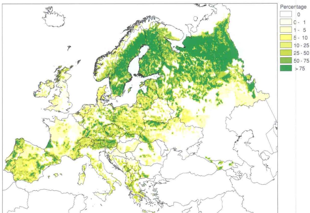
Figure 5-2. Percentage of mixed and coniferous forest per 10' x 10' grid cell.
