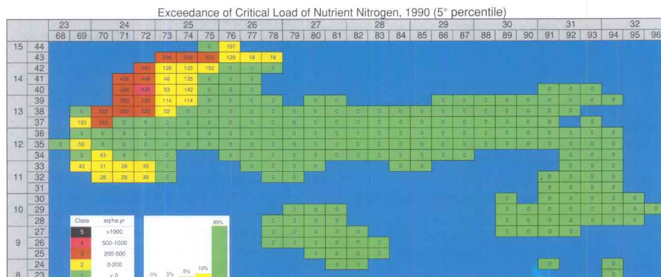
Figure IT-6. Exceedance of the critical load of nutrient nitrogen, 1990 (5th percentile).
