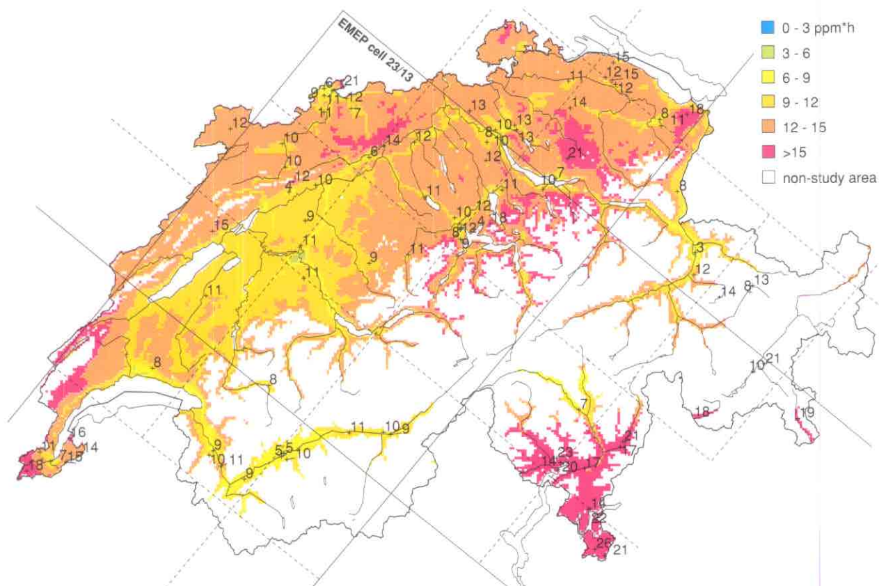
Figure CH-3. Interpolated ozone levels for crops in 1994: accumulated exposure over a threshold of 40ppb for daylight hours from May to July ( AOT_{40} ). (The critical level is 3ppm·h; the study area is below 1200m altitude.)
