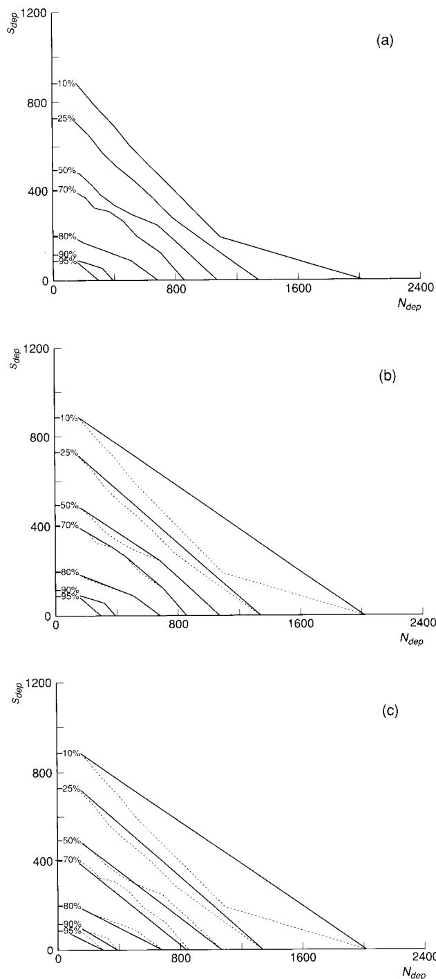
Figure 3-5. (a) Examples of protection isolines (computed from the critical load functions shown in Figure 3-4); (b) the convex hulls (solid lines) of those protection isolines (dotted lines); (c) the trapezoids (solid lines) constructed from the respective percentiles of CL_{max}(S) , CL_{min}(N) and CL_{max}(N) (protection isolines shown as dotted lines for comparison).
