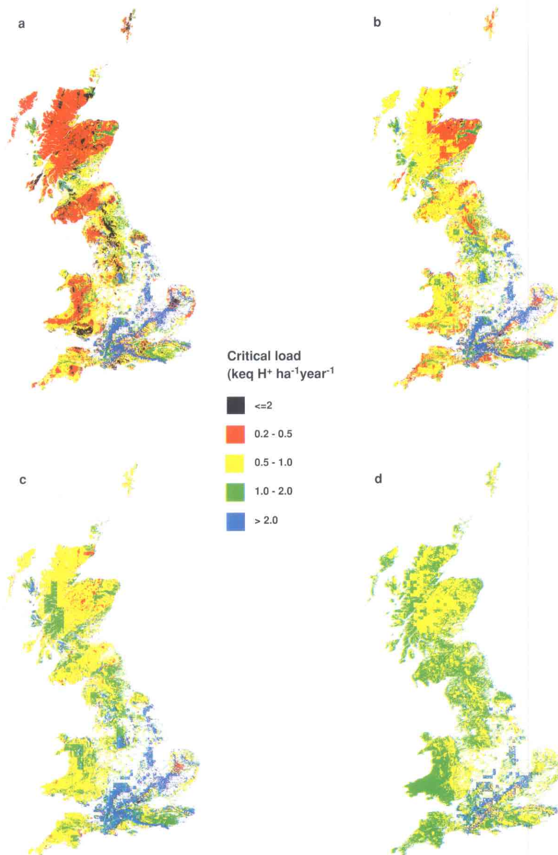
Figure UK-1. 5-percentile critical load maps for (a) acidity, (b) maximum sulfur ( CL_{max}(S) ), (c) maximum nitrogen ( CL_{max}(N) ), (d) nutrient nitrogen. The maps are based on 1 x 1 km 2 data for acid grassland, calcareous grassland, heathland, coniferous woodland and deciduous woodland ecosystems.
