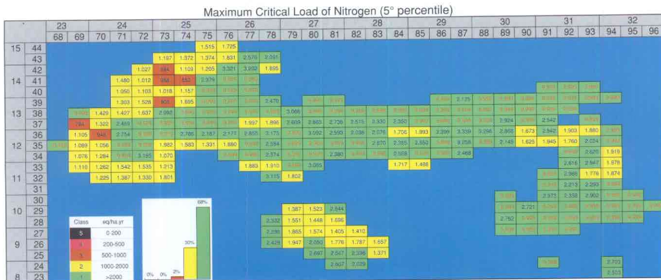
Figure IT-3. Maximum critical load of nitrogen (5th percentile).
