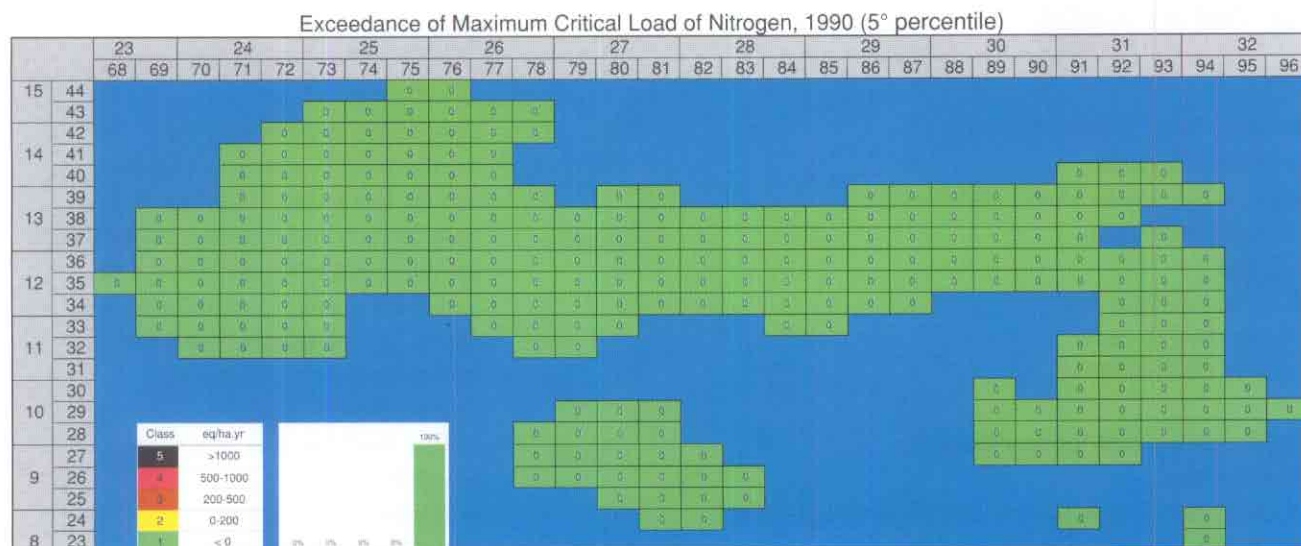
Figure IT-5. Exceedance of the maximum critical load of nitrogen, 1990 (5th percentile).
