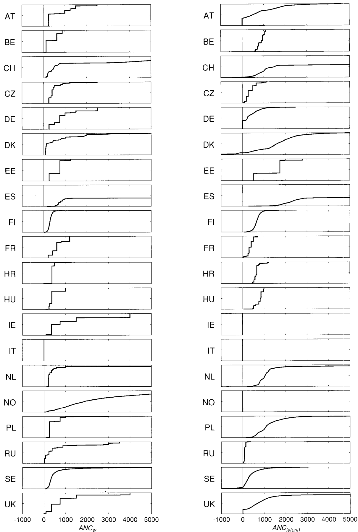
Figure 4-3. Cumulative distribution functions for critical ANC leaching and weathering (in eq\ ha^{-1}\ yr^{-1} ) used in the SMB calculations of critical loads for forest soils from national data contributions.
