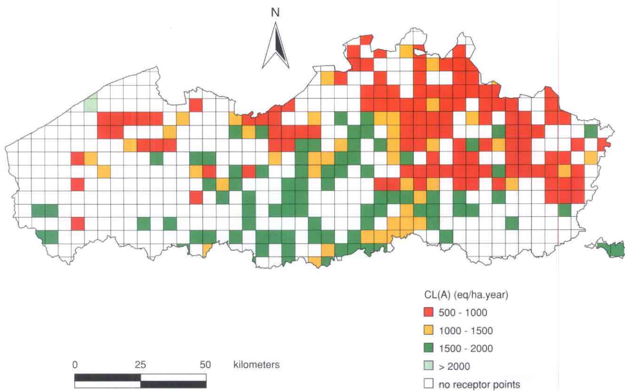
Figure BE-1. Critical load of acidity, CL(A) .
