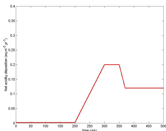
Figure FR-5. Acid deposition scenario (SO 2 only), used as input for the VSD and WiTCh models (eq m -2 a -1 ).
