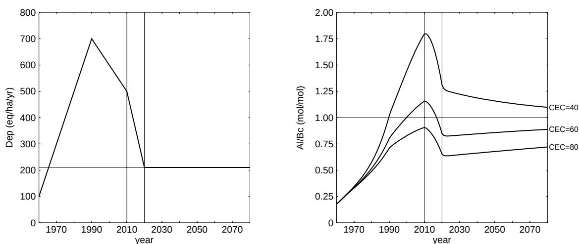
Figure 3-3. Temporal development of acidifying deposition (left) and corresponding molar Al/Bc ratio (right) for three soils varying in CEC . The vertical lines separate 50 years of “history”, 10 years (2010–2020) of implementation of emission reductions, and the future. Also shown are the critical load and the critical value ( Al/Bc_{crit}=1 ) as horizontal lines. The deposition drops to the critical load within the implementation period and the Al/Bc ratios (slowly) approach the critical value.
