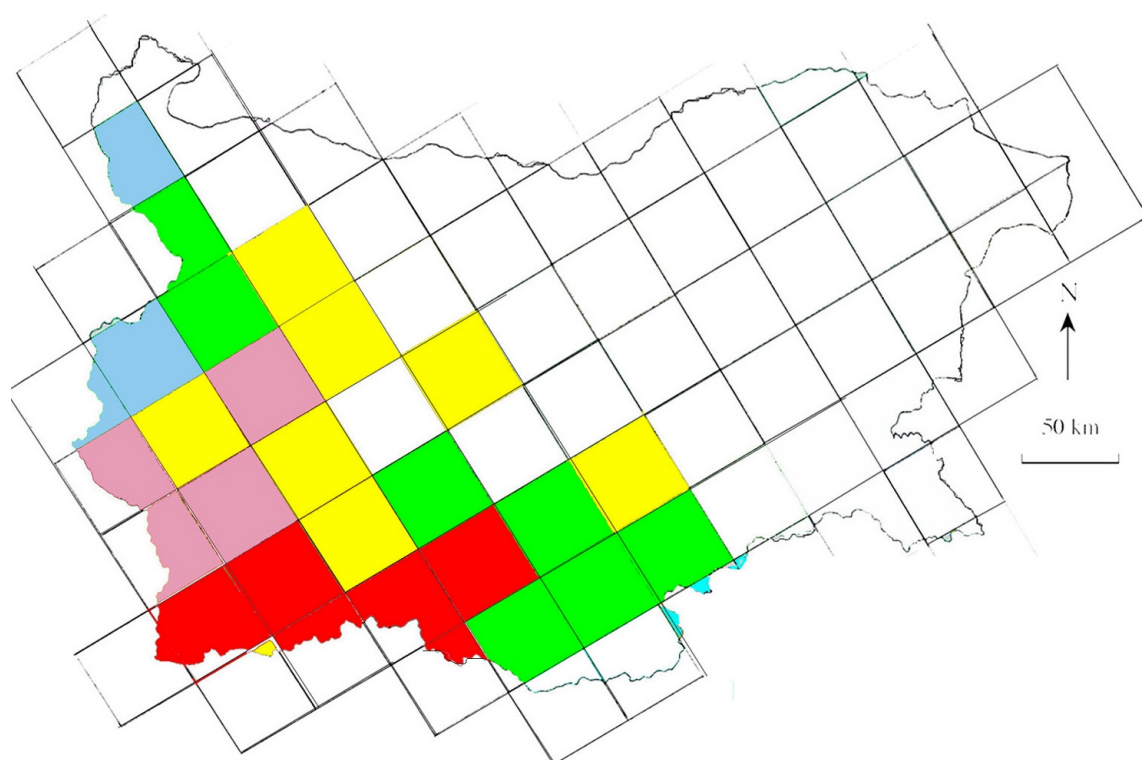
Figure BG-1. Maximum critical loads of sulphur for deciduous (top) and coniferous forests (bottom) in Bulgaria.
