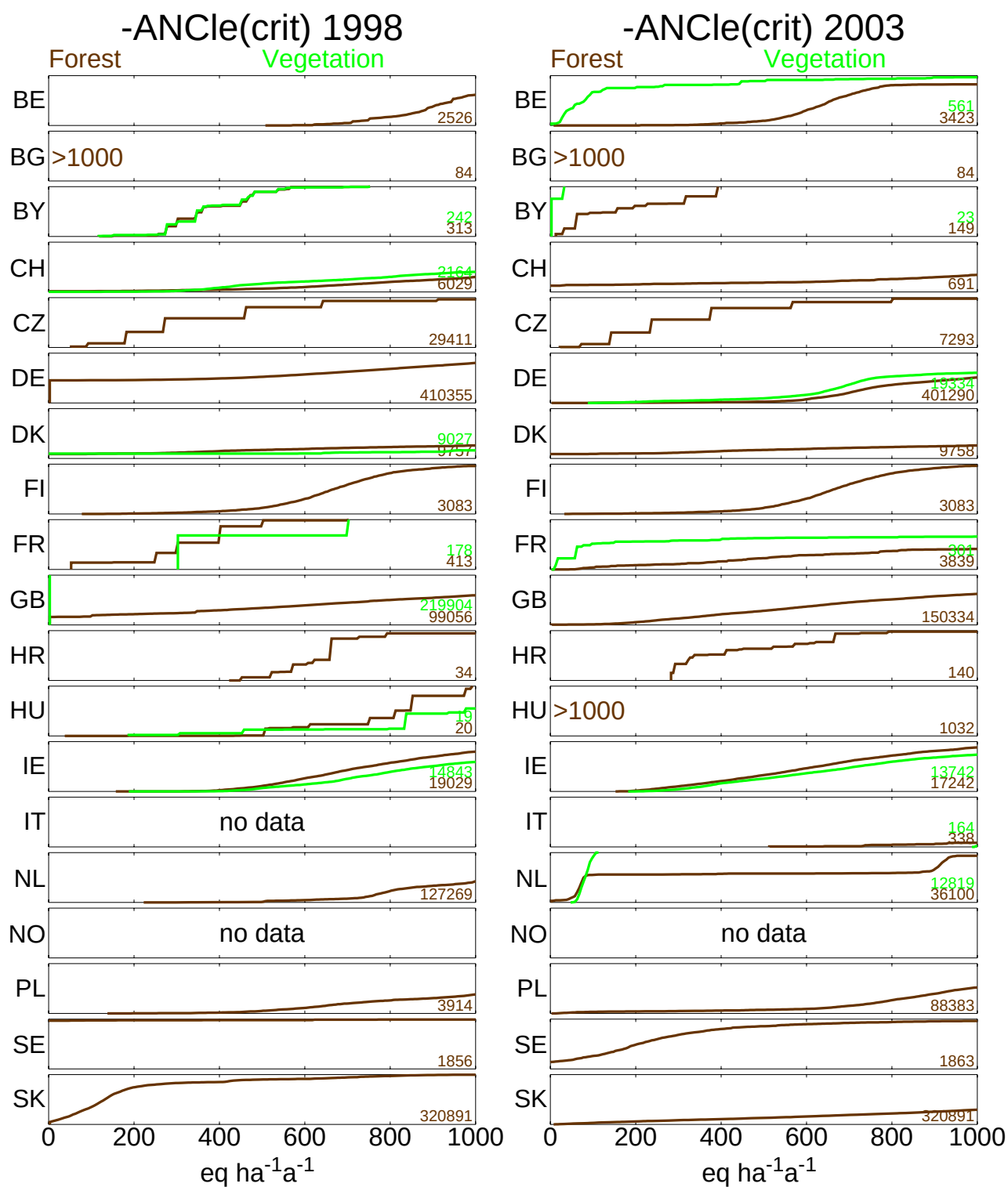
Figure 2-8. Critical leaching of acid neutralising capacity ( =Al_{le(crit)}+H_{le(crit)} ) from 1998 (left) and 2003 (right).
