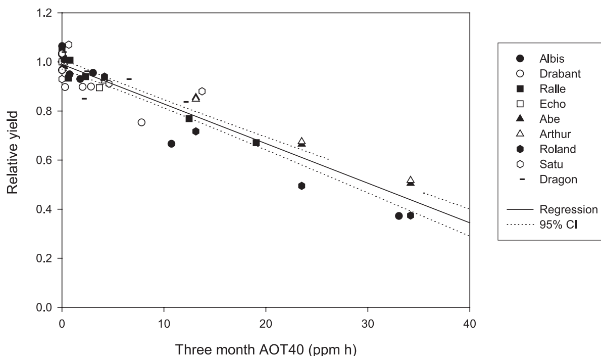
Figure 3.4: Wheat yield-response function used to derive the concentration-based critical levels for agricultural crops ( r^2 = 0.89 ) (Fuhrer et al. , 1997, Gelang et al. , 2000).
