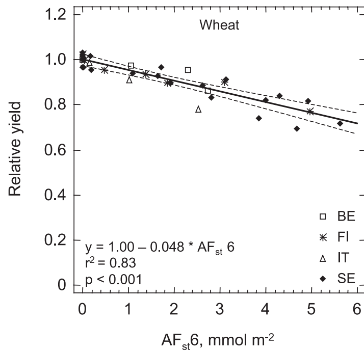
Figure 3.2: The relationship between the relative yield of wheat and AF_{st\ 6} for the wheat flag leaf based on five wheat cultivars from four European countries using effective temperature sum to describe phenology.
