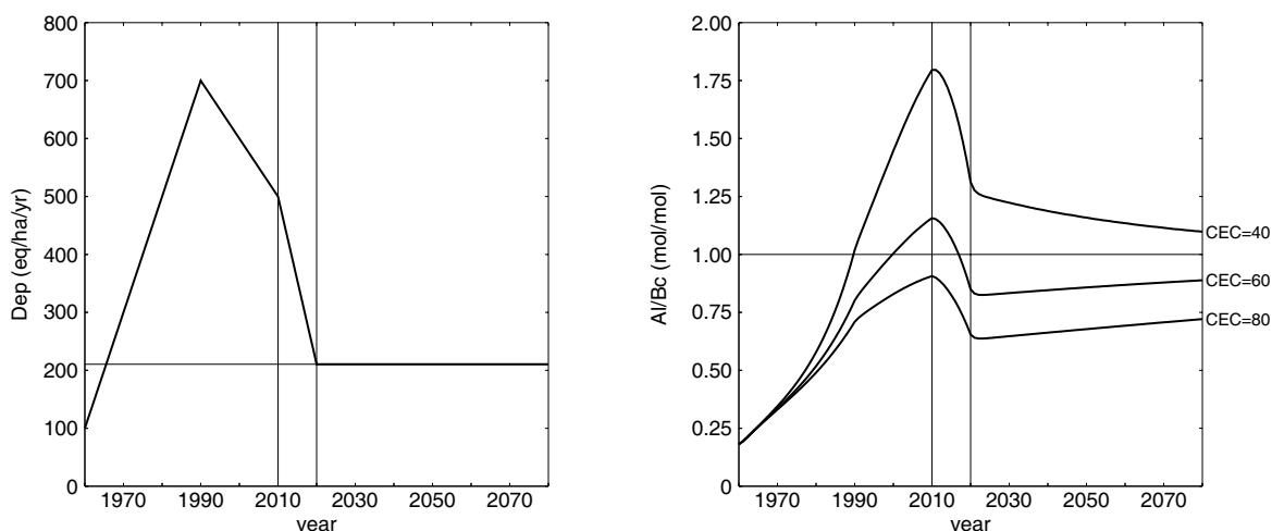
Figure 6.7: Temporal development of acidifying deposition (left) and corresponding molar Al/Bc -ratio (right) for 3 soils varying in CEC . The two vertical lines separate 50 years of 'history', 10 years (2010-2020) of implementation, and the future. Also shown are the critical load and the critical value (Al/Bc)_{crit}=1 as thin horizontal lines. The deposition drops to the critical load within the implementation period and the Al/Bc -ratios (slowly) approach the critical value.
