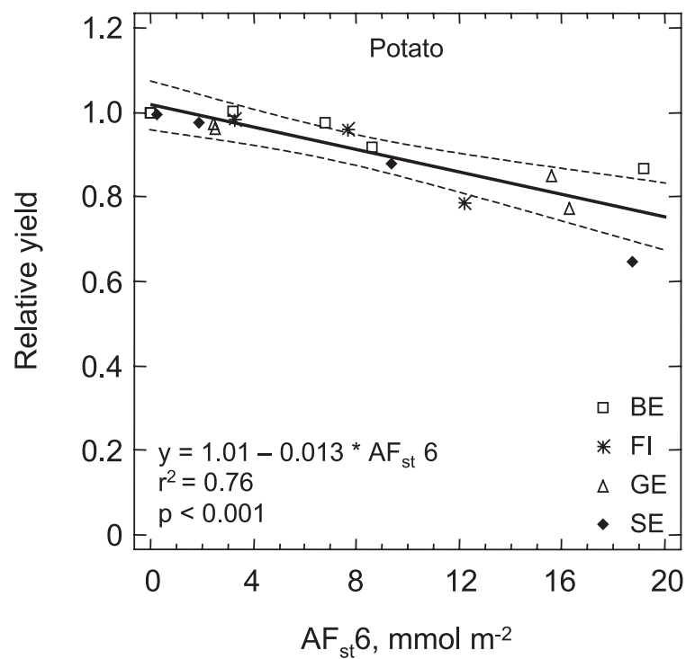
Figure 3.3: The relationship between the relative yield of potato and the AF_{st\ 6} for sunlit leaves based on data from four European countries and using effective temperature sum to describe phenology.
