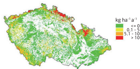
Figure CZ.2 Exceedances of empirical critical loads by atmospheric depositions of nitrogen in 2008.
