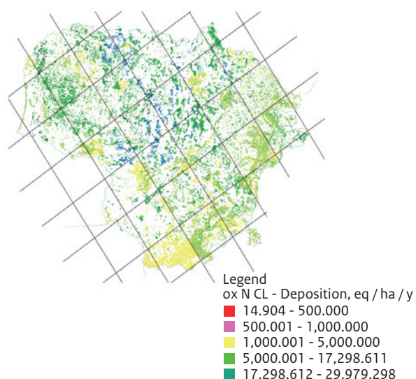
Figure LT.5 Difference of critical loads and deposition of oxidized nitrogen; negative values represent exceedances of critical load (in eq ha -1 yr -1 ).
