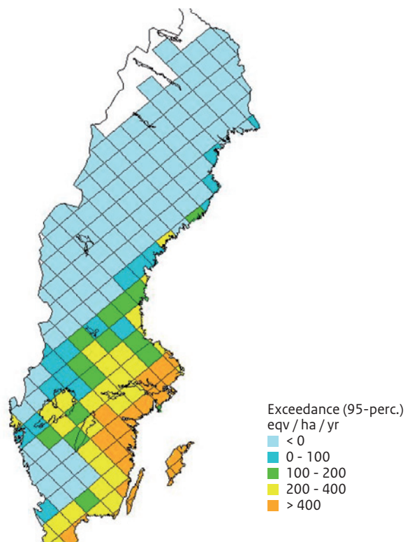
Figure SE.2 Exceedance of critical load of acidity, with the criteria molar BC/Al = 1 (root weighted), on 17,141 sites in Sweden. Exceedance based on EMEP deposition for 2010. For each square the 95 th percentile is shown, i.e. 5% of the ecosystem area has this or higher exceedance.
