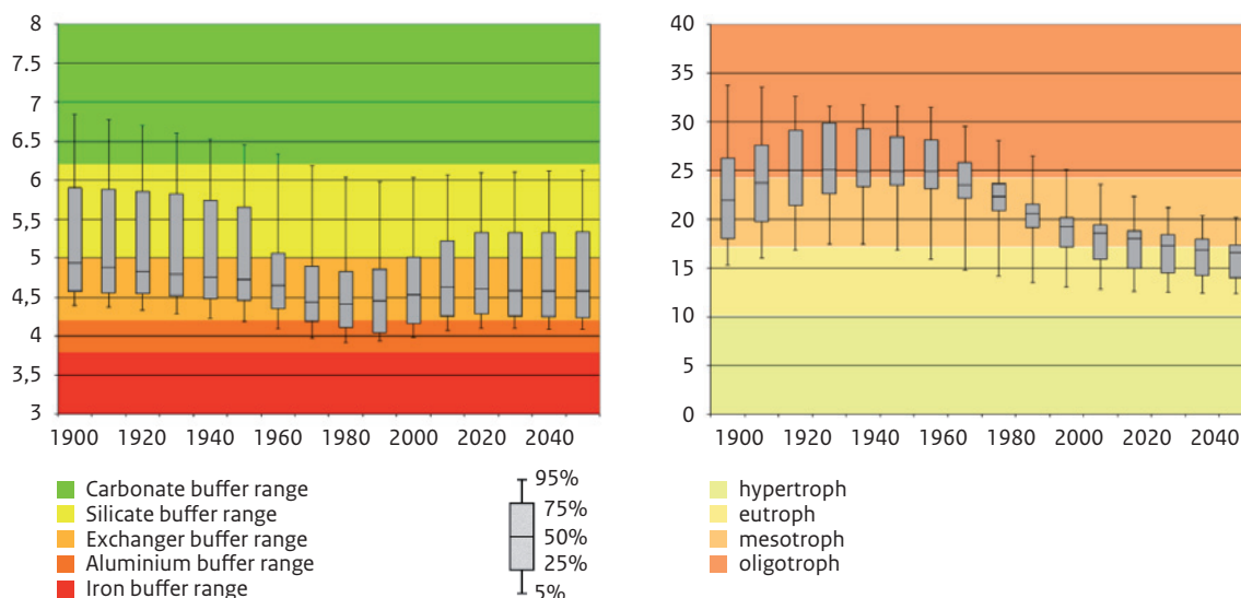
Figure DE.7 pH value (left) and C:N ratio (right) modelled with the VSD+ model.
