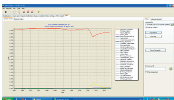
Figure BG.7 Results of the VSD+Veg modelling for Vitinya.
