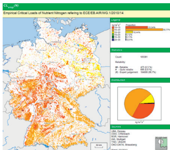
Figure DE.4 CL_{emp}(N) .
