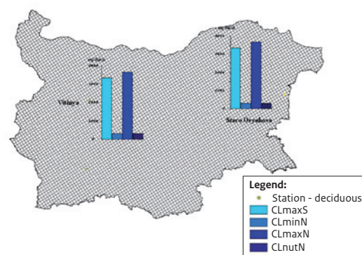
Figure BG.3 Map of the critical loads of S, N and nutr.N (eq ha -1 a -1 ) - Deciduous.
