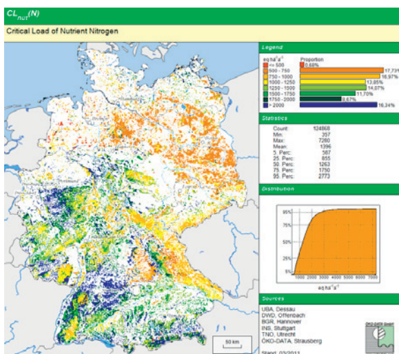
Figure DE.3 CL_{nut}(N) .
