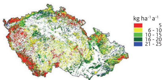
Figure CZ.1 Empirical critical loads for nitrogen for forest ecosystems including grassland.
