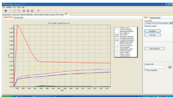
Figure BG.5 Results of the VSD+Veg modelling for Jundola.
