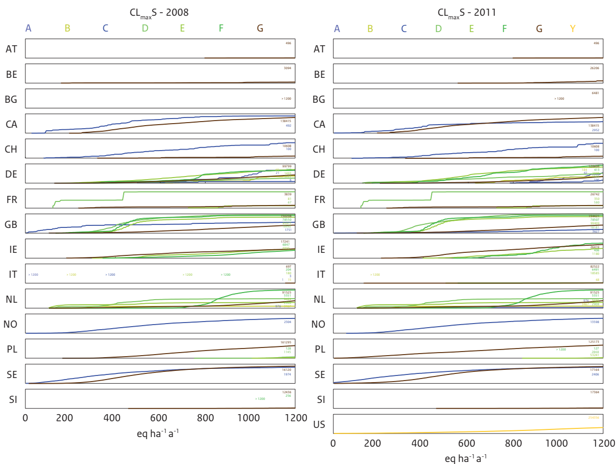
Figure 2.7 CDFs of the maximum critical load of acidity (CLmax5) of countries that submitted in both 2008 (left) and 2011(right), split by EUNIS class.
