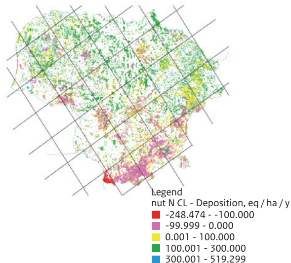
Figure LT.6 Difference of critical loads and deposition of nutrient nitrogen; negative values represent exceedances of critical load (in eq ha -1 yr -1 ).
