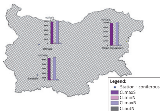
Figure BG.2 Map of the critical loads of S, N and nutr.N (eq ha -1 a -1 ) - Coniferous.
