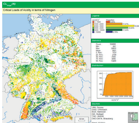
Figure DE.2 CL_{max}(N) .
