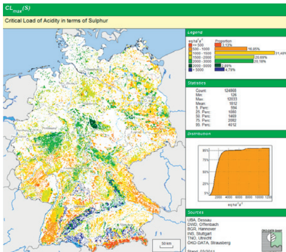
Figure DE.1 CL_{max}(S) .
