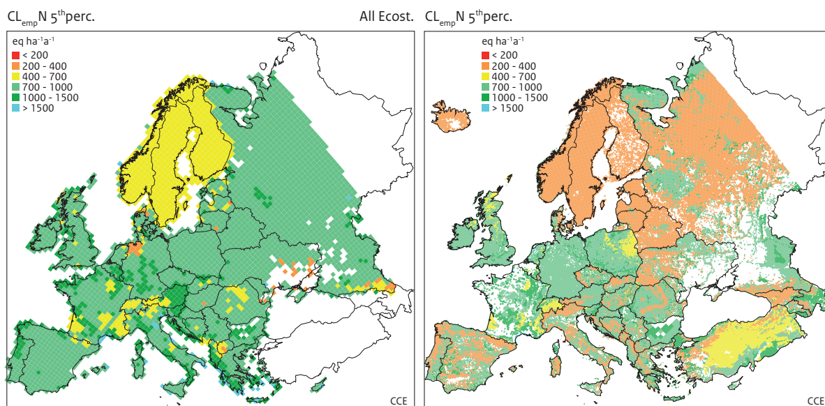
Figure 2.6 The 5 th percentiles of the empirical critical loads of N for the 2008 dataset (left, 50×50 km 2 EMEP grid) and the 2011 dataset (right, 10×10 km 2 EMEP grid).
