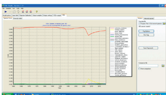
Figure BG.9 Results of the VSD+Veg modelling for Staro Oryahovo (Simpson Index).
