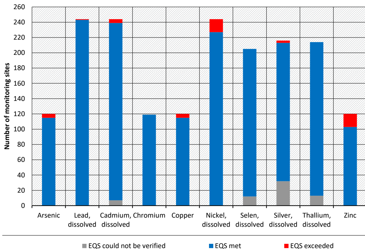
Comparison of annual means in 2016-2018 with the environmental quality standard (dissolved concentration and suspended solids/sediment, LAWA monitoring sites)
