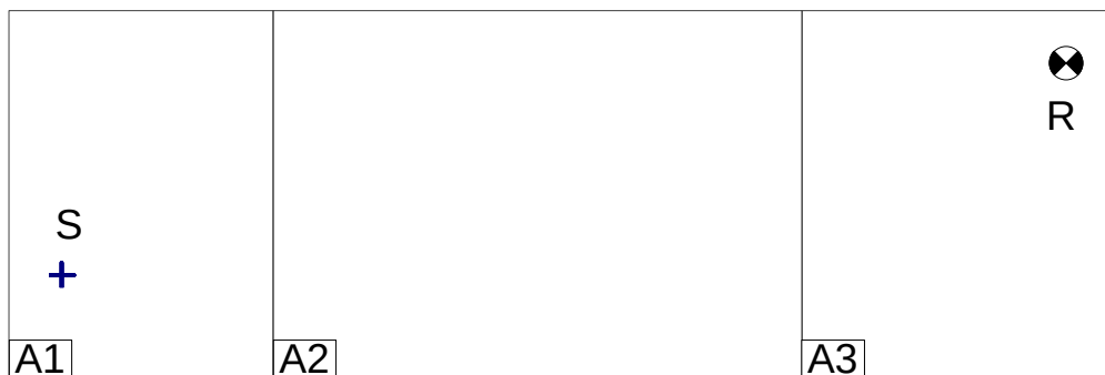
Figure 5.3.5-1: Scenario with level ground but varying acoustic properties (S source, R point of immission, A1 area with G=0.2, A2 area with G=0.5, A3 area with G=0.9) (Source: Umweltbundesamt [9])
