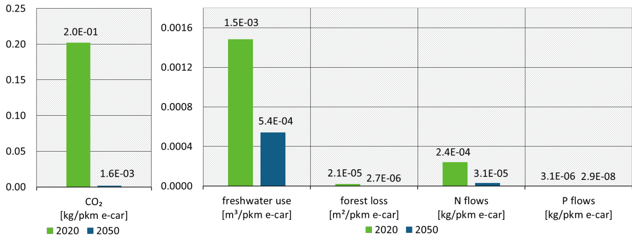
Figure 9: Environmental impacts of an electric car*, 2020 and 2050
