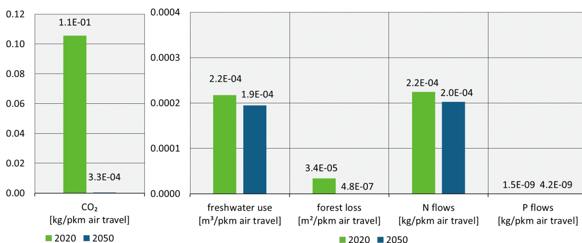
Figure 13: Environmental impacts of air travel (fuel only), 2020 and 2050
