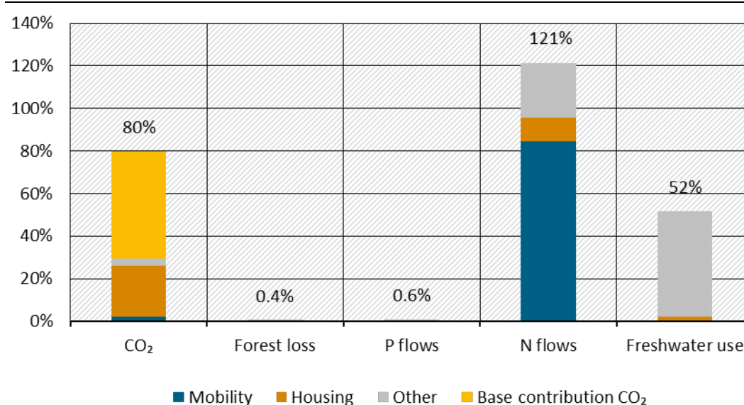
Figure 37: Kaulatz family – environmental impacts of consumption per person (excluding food) relative to planetary boundaries
