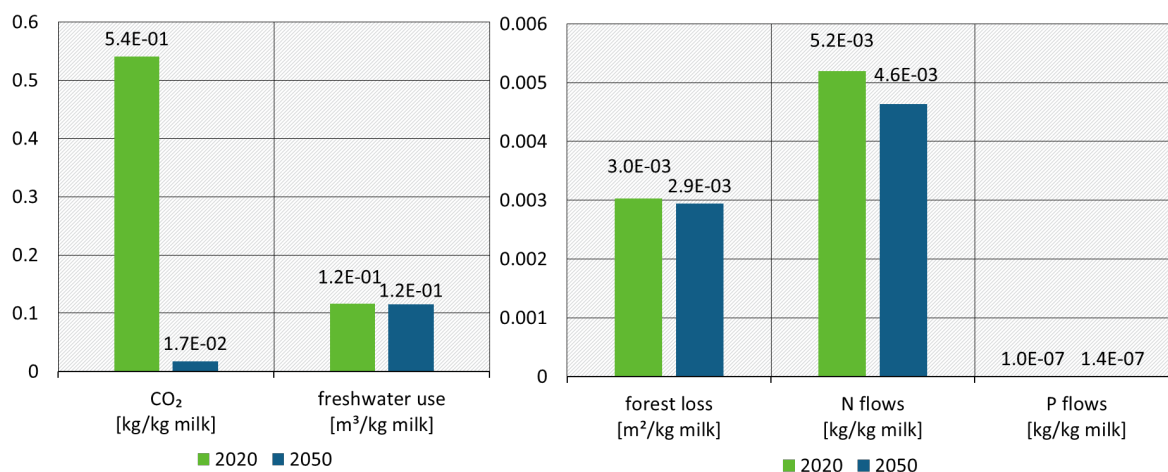
Figure 7: Environmental impacts of milk, today and in 2050
