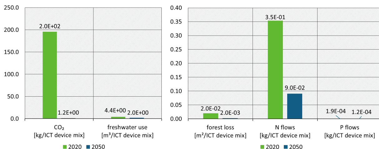
Figure 20: Environmental impacts of ICT devices, 2020 and 2050
