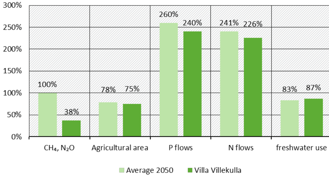
Figure 44: Villa Villekulla – environmental impacts of food per person relative to planetary boundaries compared to the average in 2050
