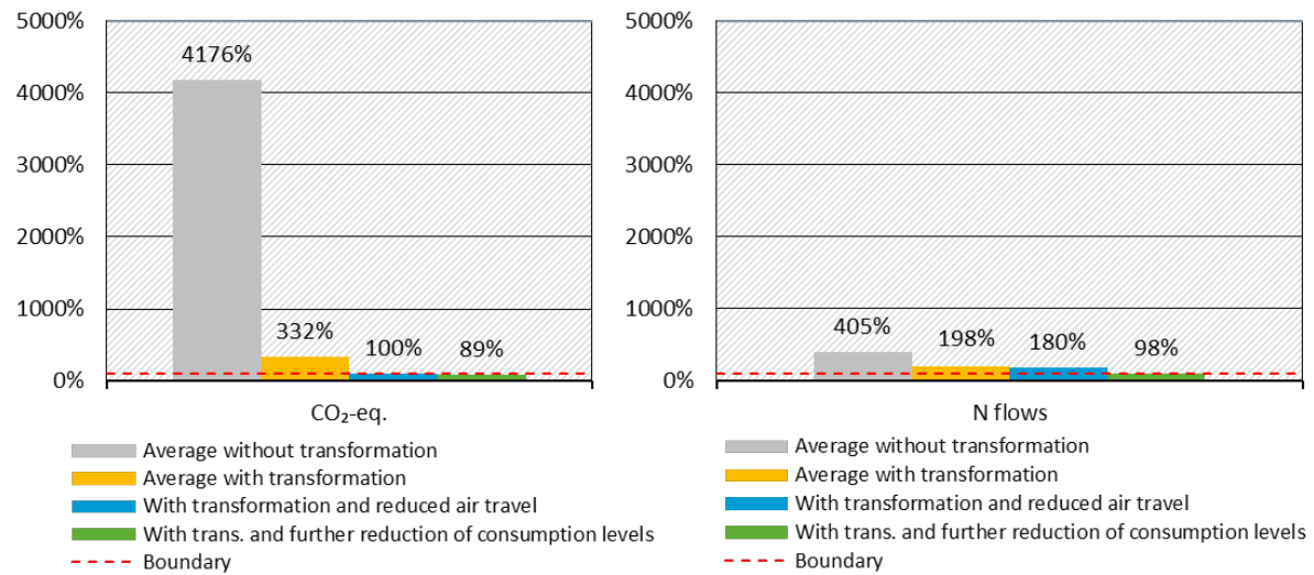
Figure 24: Environmental impacts of average German consumption (excluding food and base contribution) relative to CO 2 and nitrogen budgets without and with transformation as well as with reduced consumption levels
