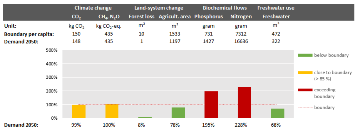
Figure 25: The consumption level of the GreenSupreme average citizen compared to the planetary boundaries (incl. only CO 2 from air travel)
