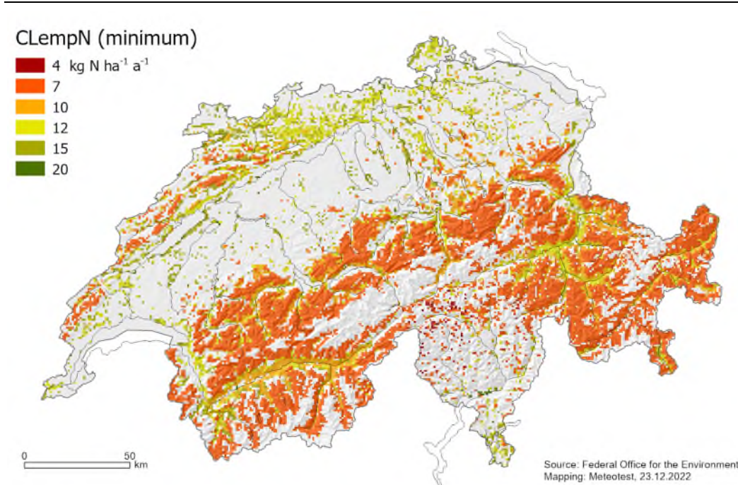
Figure 35 Empirical critical loads of nutrient nitrogen for (semi-)natural ecosystems, CL_{empN} , minimum per km 2 .
