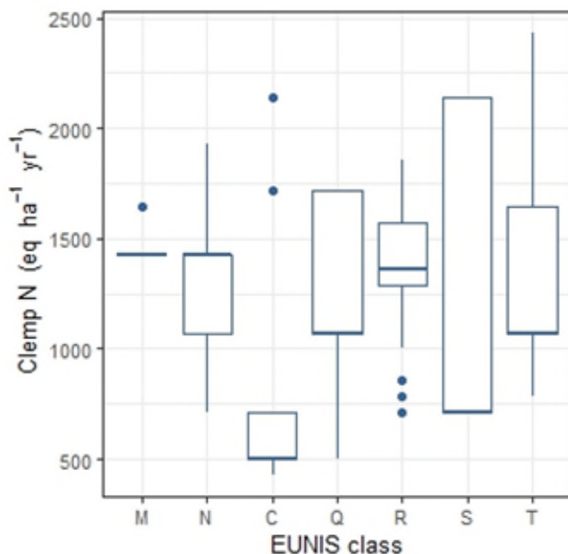
Figure 14 Box-plots of empirical Critical Load values from the 7 EUNIS classes, based on the selected records (in eq ha -1 a -1 , n = 71423)
