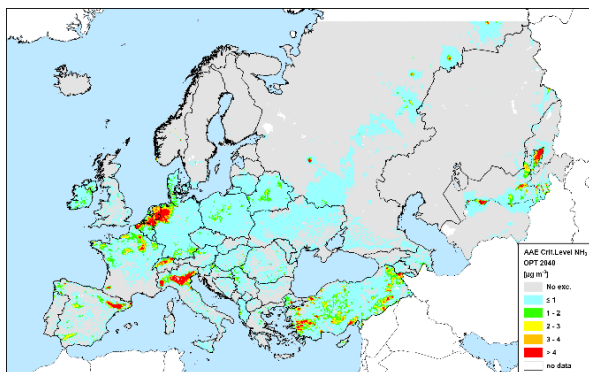
E: Exceedance of Critical Levels with 2040 MTRF scenario
