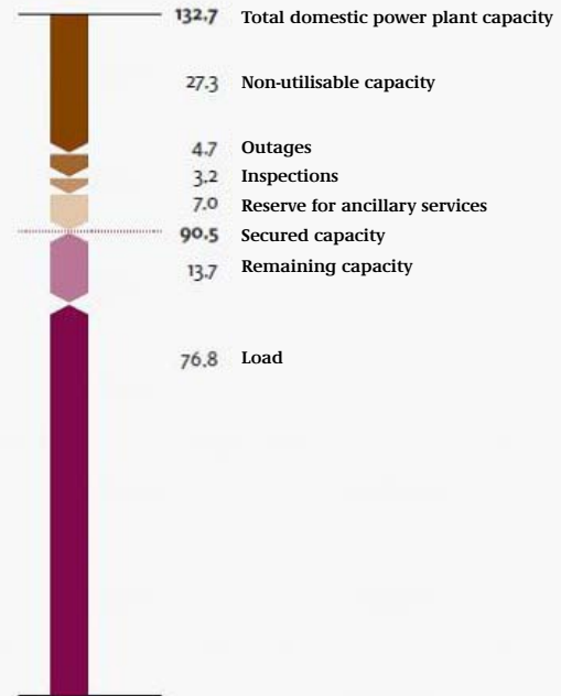
Performance of overall power supply in Germany at time of annual peak load (2008), in GW
