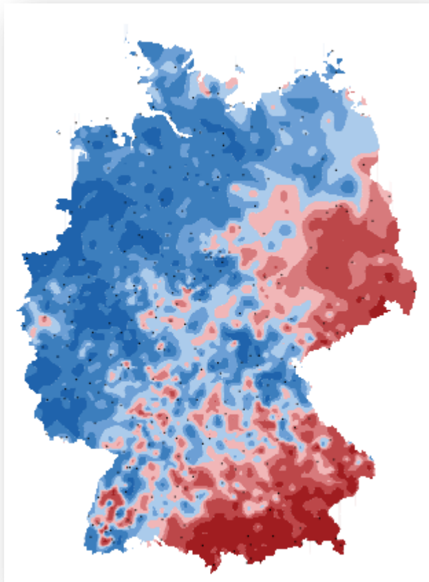
Change in precipitation 2051 – 2060 minus 1951 - 2006
