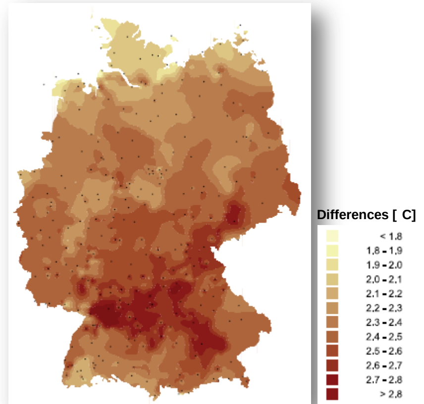
Change in temperature 2051 – 2060 minus 1951 - 2006
