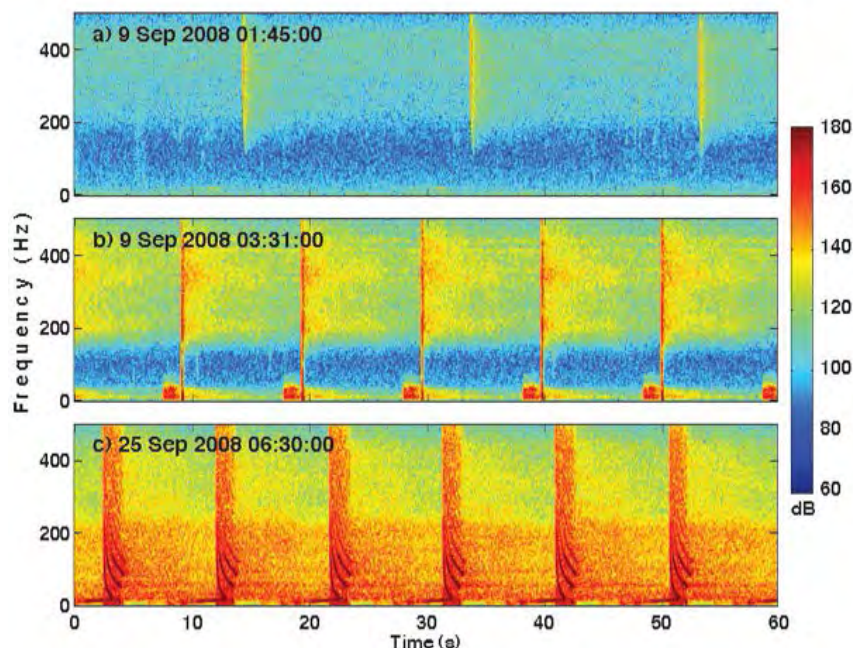
Fig. 8-1 Airgun impulses at different distances to the source
