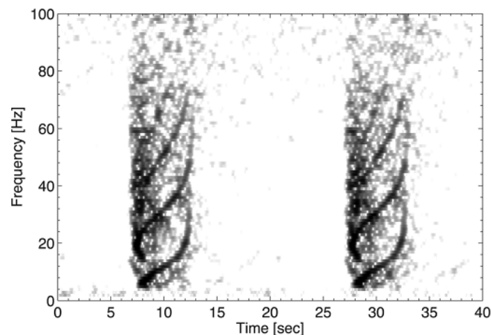
Fig. 8-2 Airgun shots registered in the Chukchi Sea
