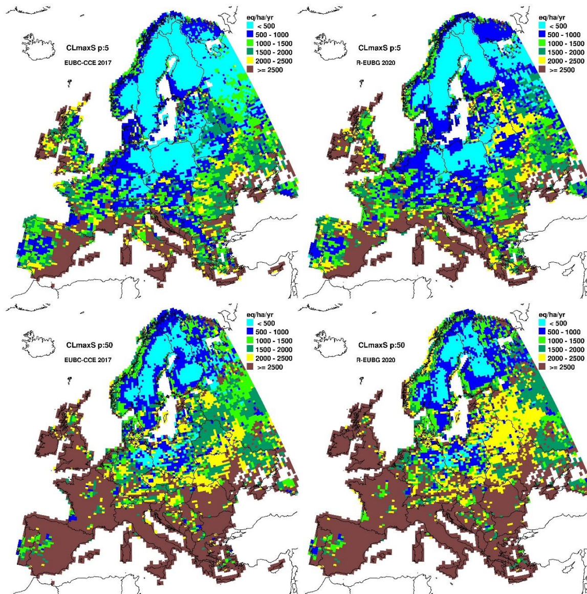
Figure 10: 5-th percentile (upper row) and median (lower row) CLmaxS in eq/ha/yr for the 2017 background DB (left) and the EUDB 2020 (right)
