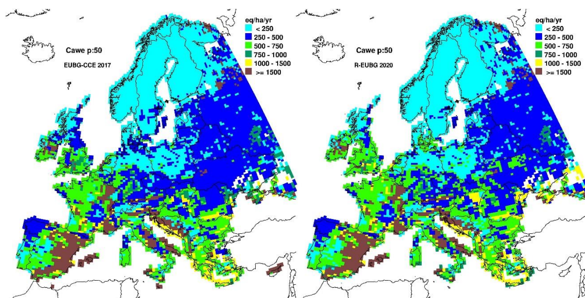
Figure 7: Median Calcium weathering (Cawe) in eq/ha/yr for the 2017 background DB (left) and the EUDB 2020 (right)
