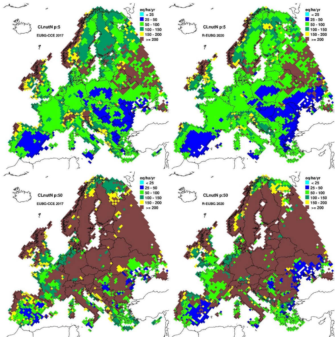
Figure 11: 5-th percentile (upper row) and median (lower row) CLnutN in eq/ha/yr for the 2017 background DB (left) and the EUDB 2020 (right)
