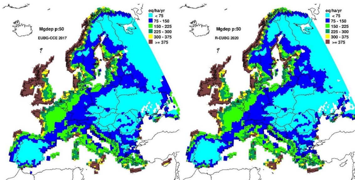
Figure 6: Median Magnesium deposition (Mgdep) in eq/ha/yr for the 2017 background DB (left) and the EUDB 2020 (right)
