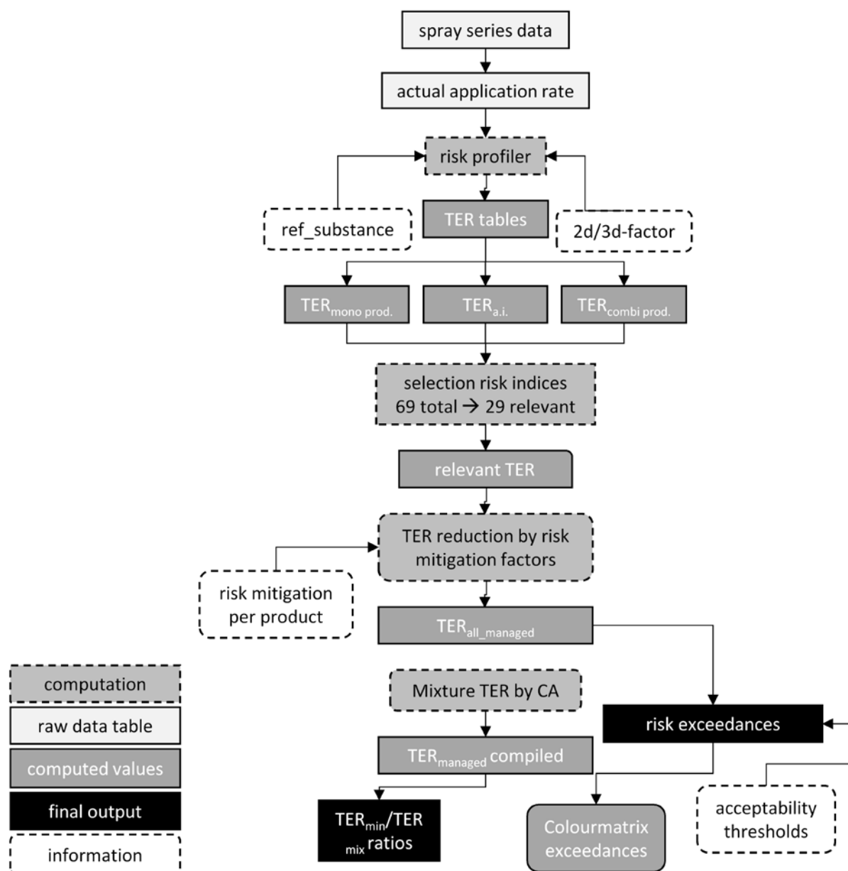
Figure 33: Generic workflow of spray series data processing and mixture risk indices calculations
