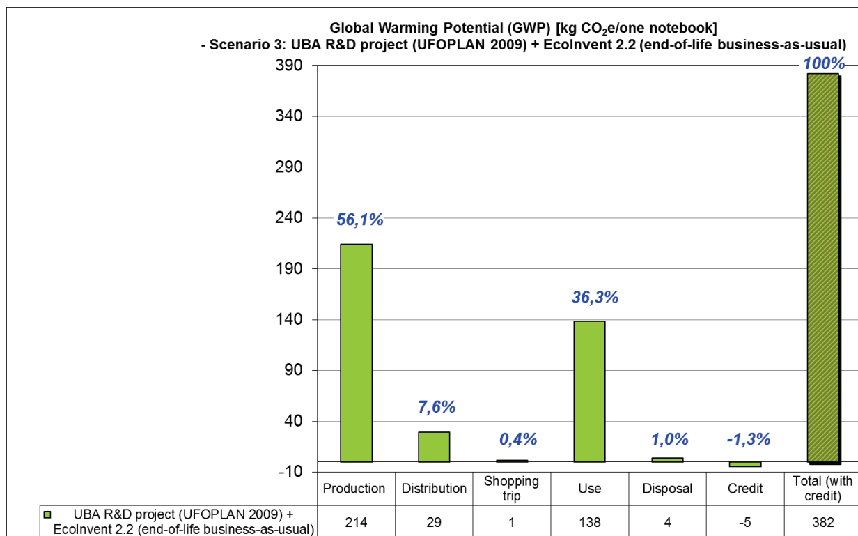
Figure 6: Absolute GWP values and percentage proportions of life cycle phases in Scenario 3: UBA R&D project (UFOPLAN 2009) + EcoInvent and end-of-life as business-as-usual
