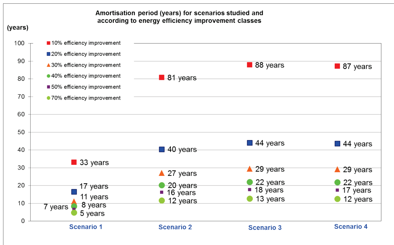
Figure 11: Overview of amortisation period as a function of energy efficiency improvement in the use phase, for all scenarios
