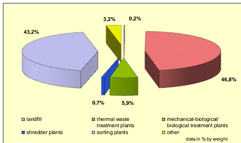
Figure 6-1: Allocation of mixed commercial municipal waste (EWL 20030102) and mixed packaging waste (EWL 15010600) to different disposal plants in the year 2007 8 (data in % by weight)
