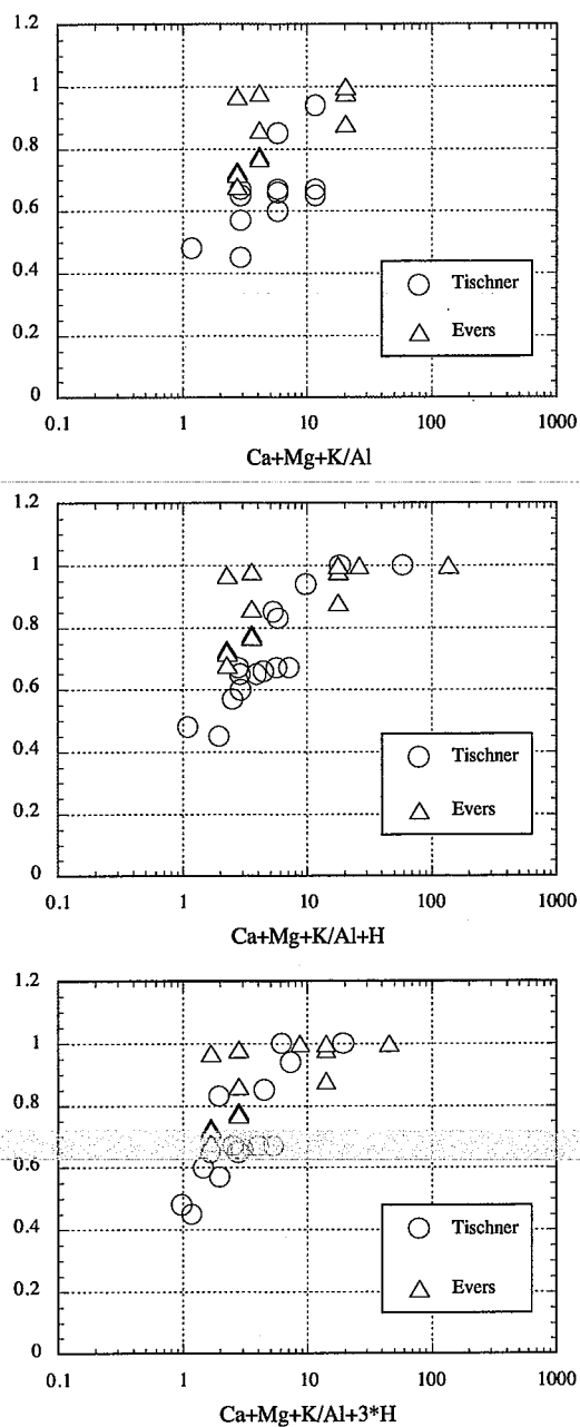
Figure 11: Test of different effect parameters on experiments on Norway spruce ( Picea abies ) performed by Tischner et al., (1985) and Evers (1983). The effect parameter tested is (\text{Ca}+\text{Mg}+\text{K})/(\text{Al}+p \cdot \text{H}) where p vary from 0 to 3.
