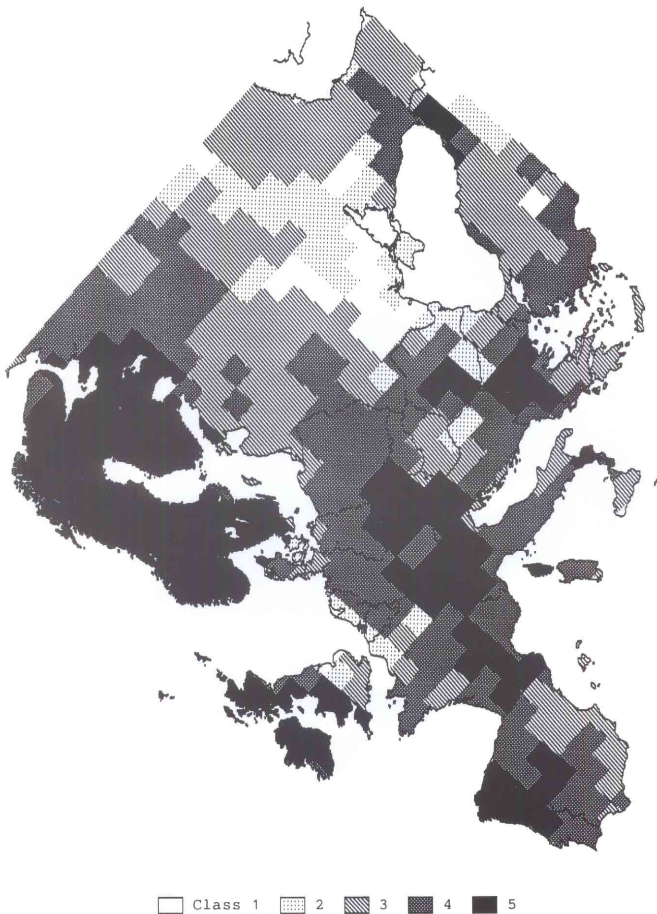
Figure 4.5. The Stockholm Environment Institute 1 percentile critical loads map presented as classes.
