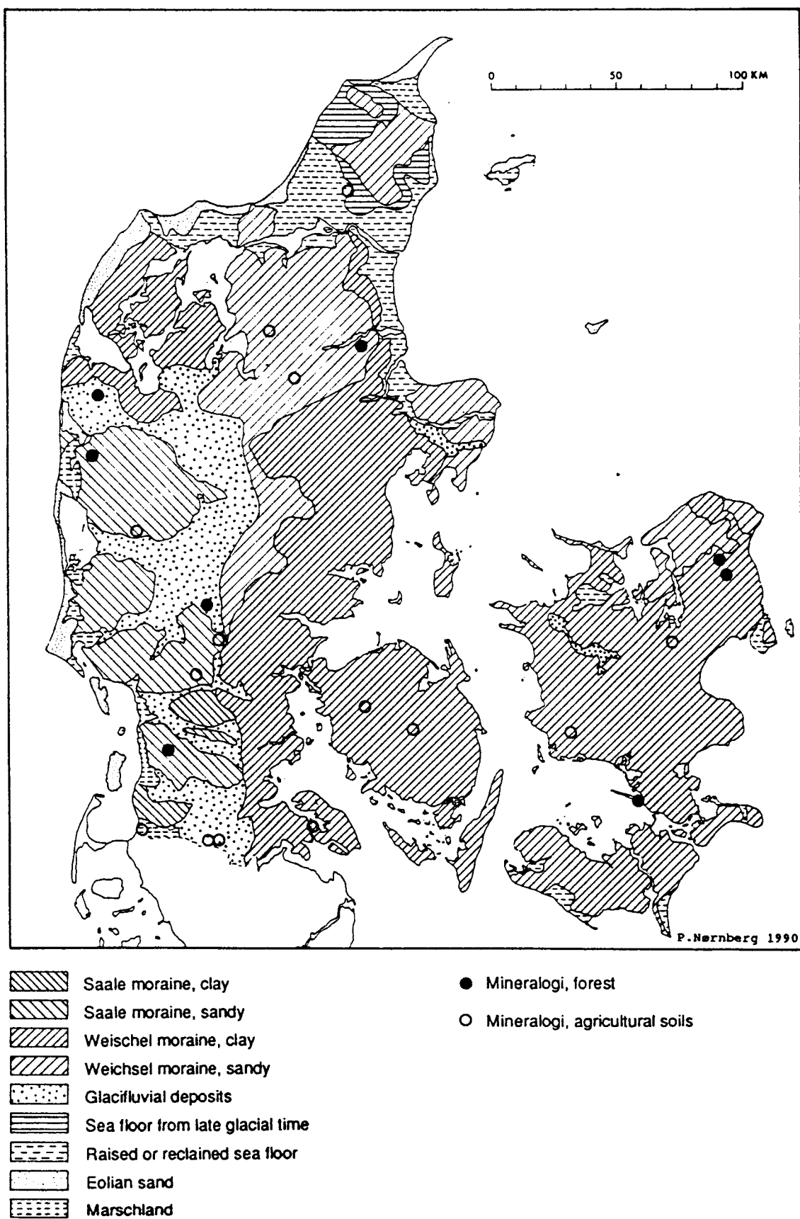
Figure A1.5. Denmark: Surface geology.
