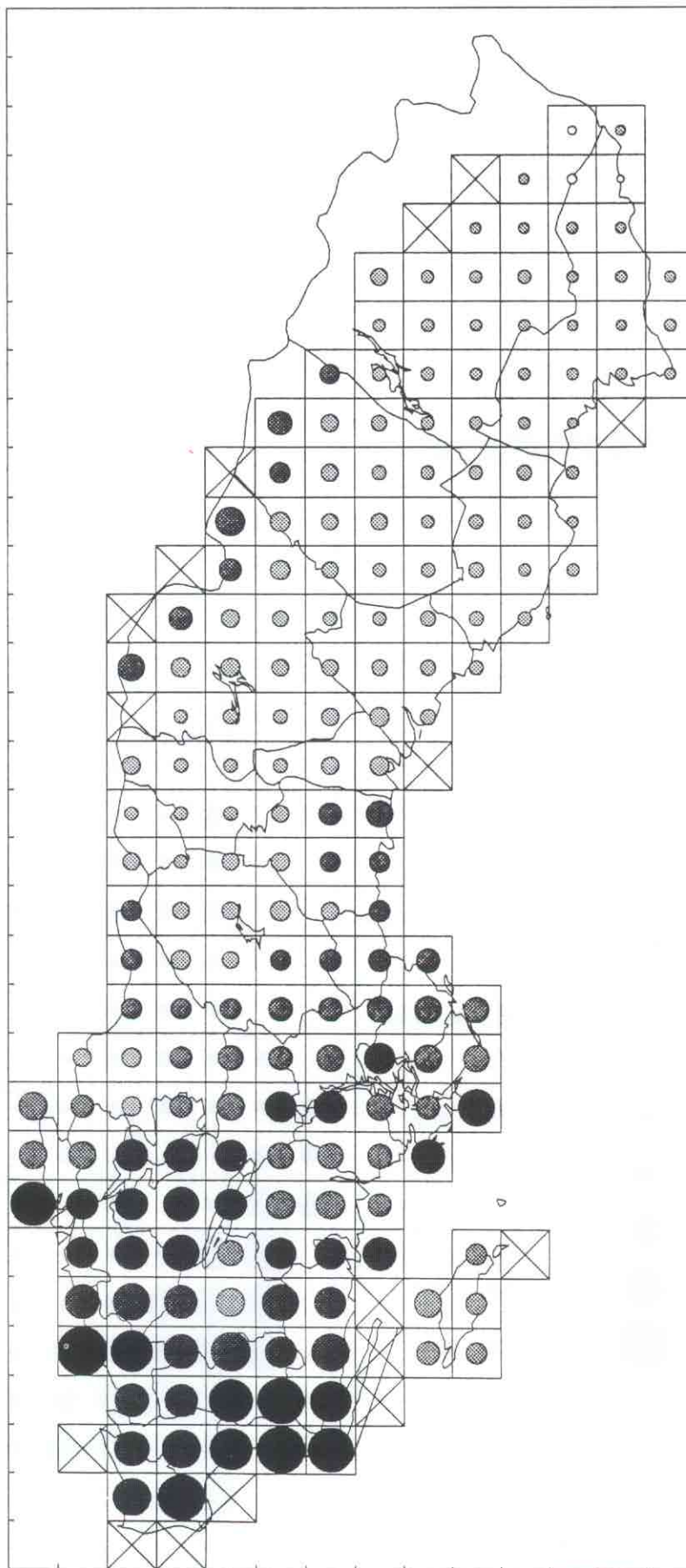
Figure A1.37. Sweden: Critical nitrogen nutrient load (5 percentile; Swedish national grid).
