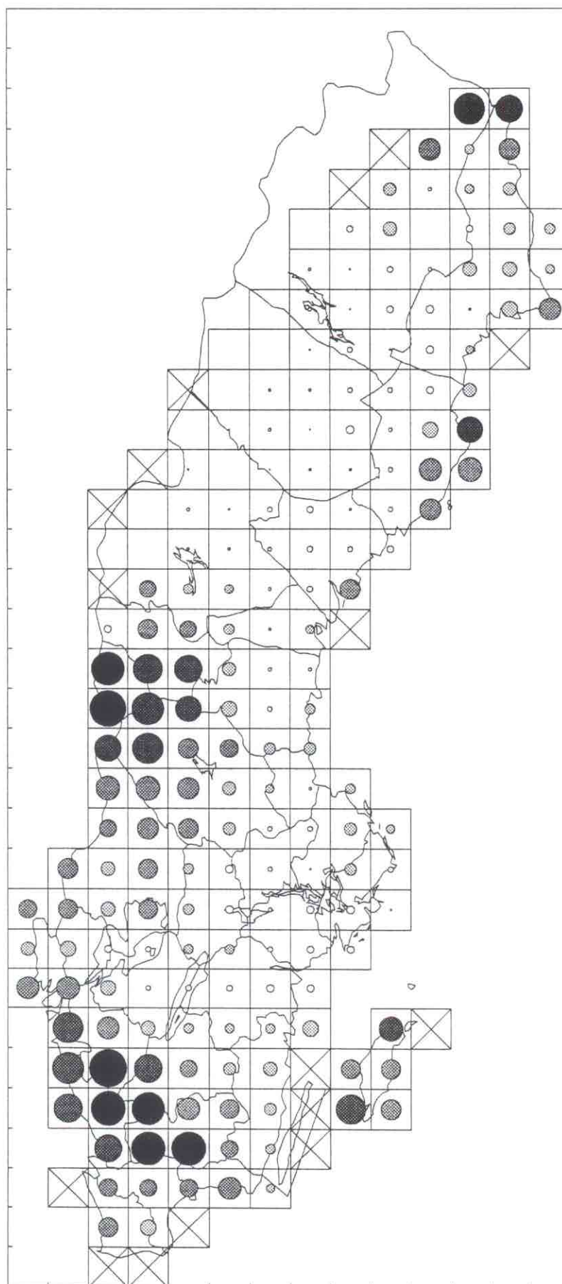
Figure A1.39. Sweden: Exceedance of critical load of nitrogen, expressed in percent area exceeded.
