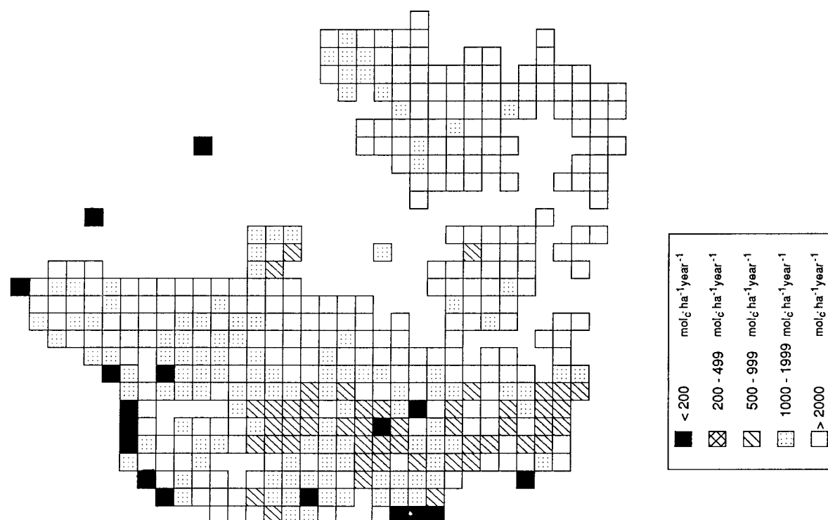
Figure A1.8. Denmark: Critical load of potential acidity for beech.
