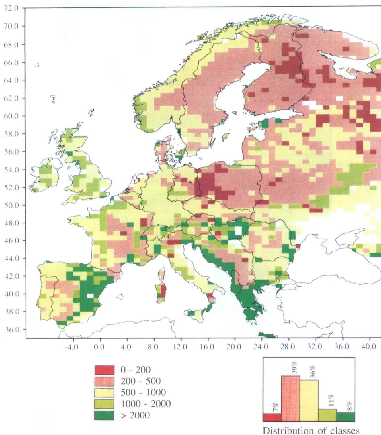
Figure A2.7. 1 percentile critical load map of potential acidity. (See Sverdrup et al. , 1990).
