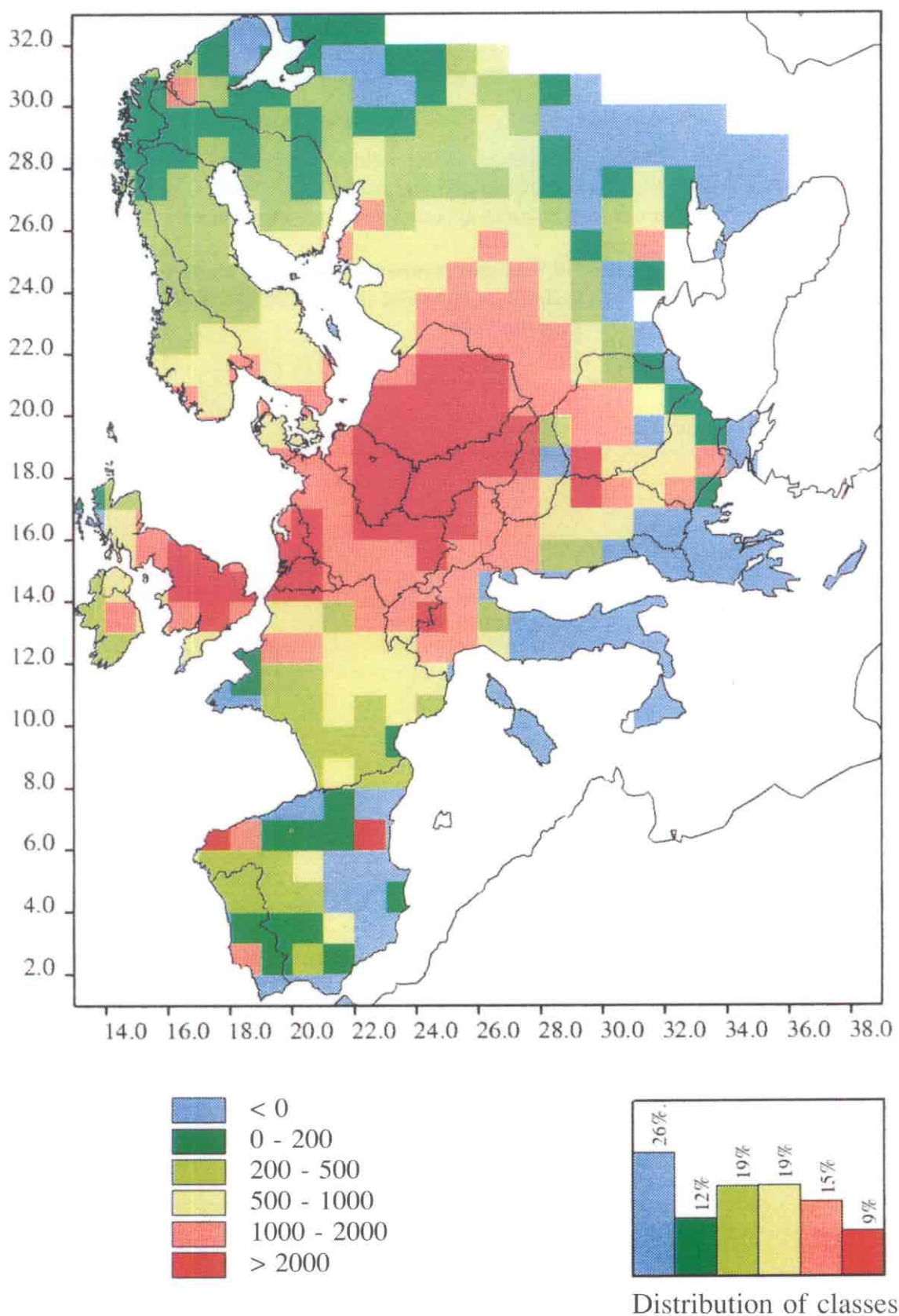
Figure 2.5a. Exceedance of the critical load of sulphur (1 percentile). Units = equivalents \text{ha}^{-1} \text{yr}^{-1} .
