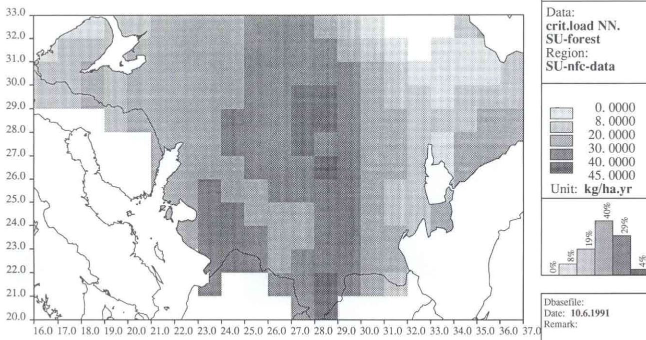
Figure A1.45. USSR: Distribution of critical loads of nutrient nitrogen.
