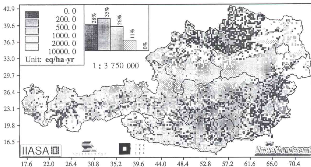
Figure A1.3. Austria: Sulphur fraction of critical loads of acidity.
