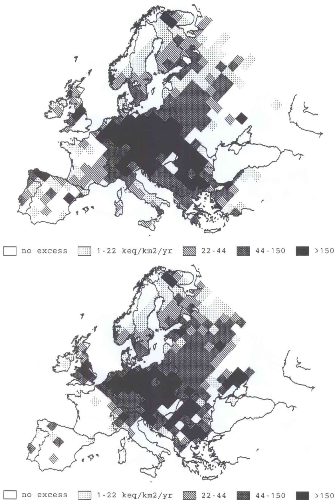
Figure 4.17. The exceedance of the SEI (upper map) and CCE (lower map) 5 percentile critical loads by the 2000 sulphur deposition (calculated using SEI emission estimates and EMEP transfer coefficients).
