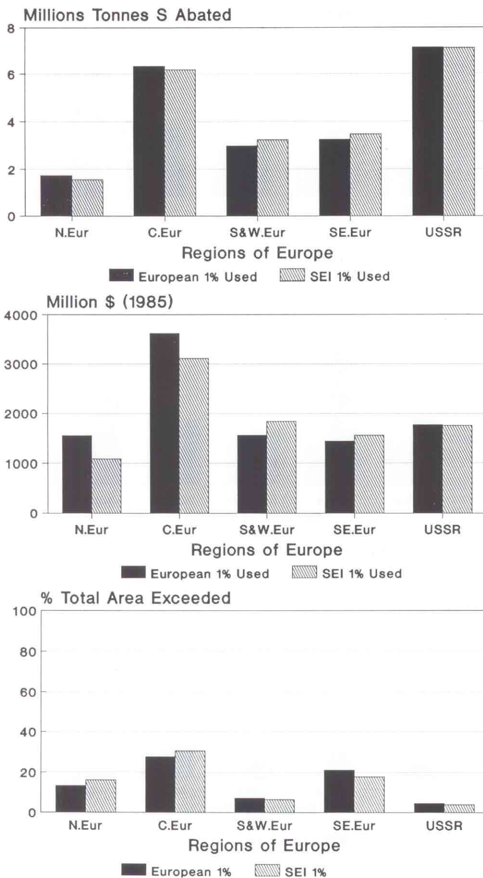
Figure 4.20. The amount of sulphur abated; the cost of abatement, and the exceedance of resulting deposition over SEI high-resolution targets using the 1 percentile SEI and CCE critical loads for an exceedance minimization at the cost of a uniform 50% reduction in emissions (using CASM).
