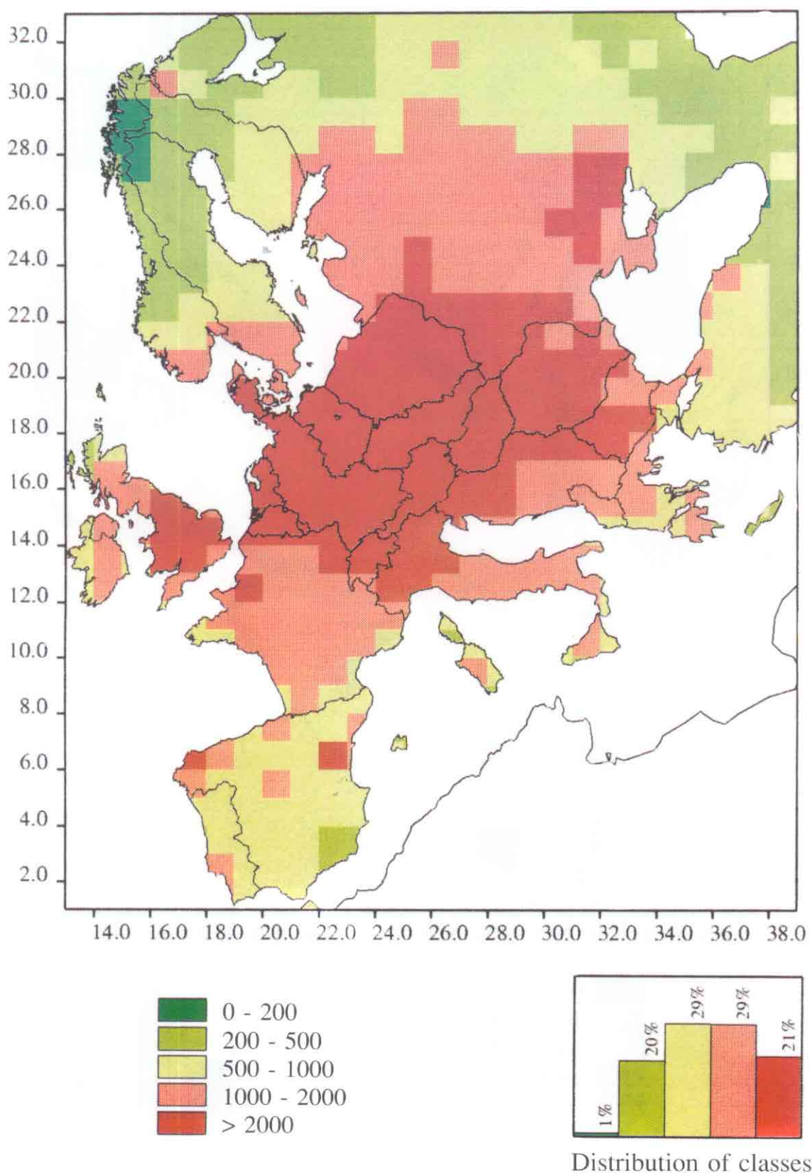
Figure A2.6. Present load computation of acidity using the 1988/1989 EMEP source-receptor matrix.
