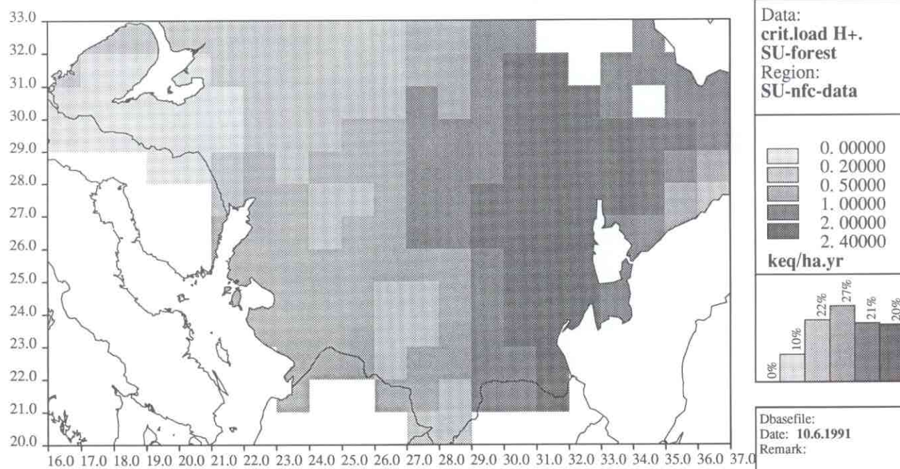
Figure A1.43. USSR: Distribution of critical loads of acidity.
