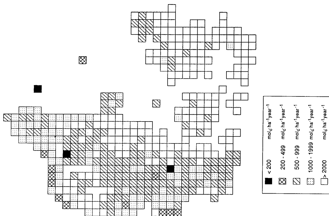
Figure A1.6. Denmark: Critical load of potential acidity for spruce.
