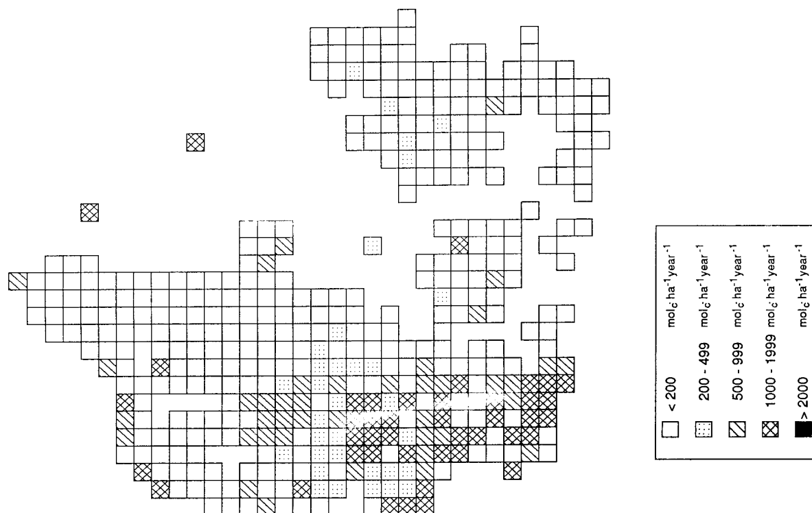
Figure A1.9. Denmark: Exceedance of critical load of acidity for beech.
