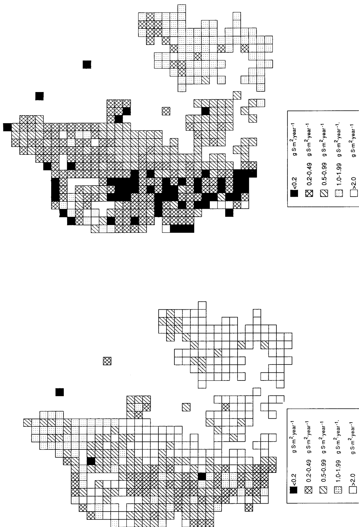
Figure A1.12. Denmark: Sulphur impact load (EMEP) for spruce when 0% of surplus nitrogen is leached.
