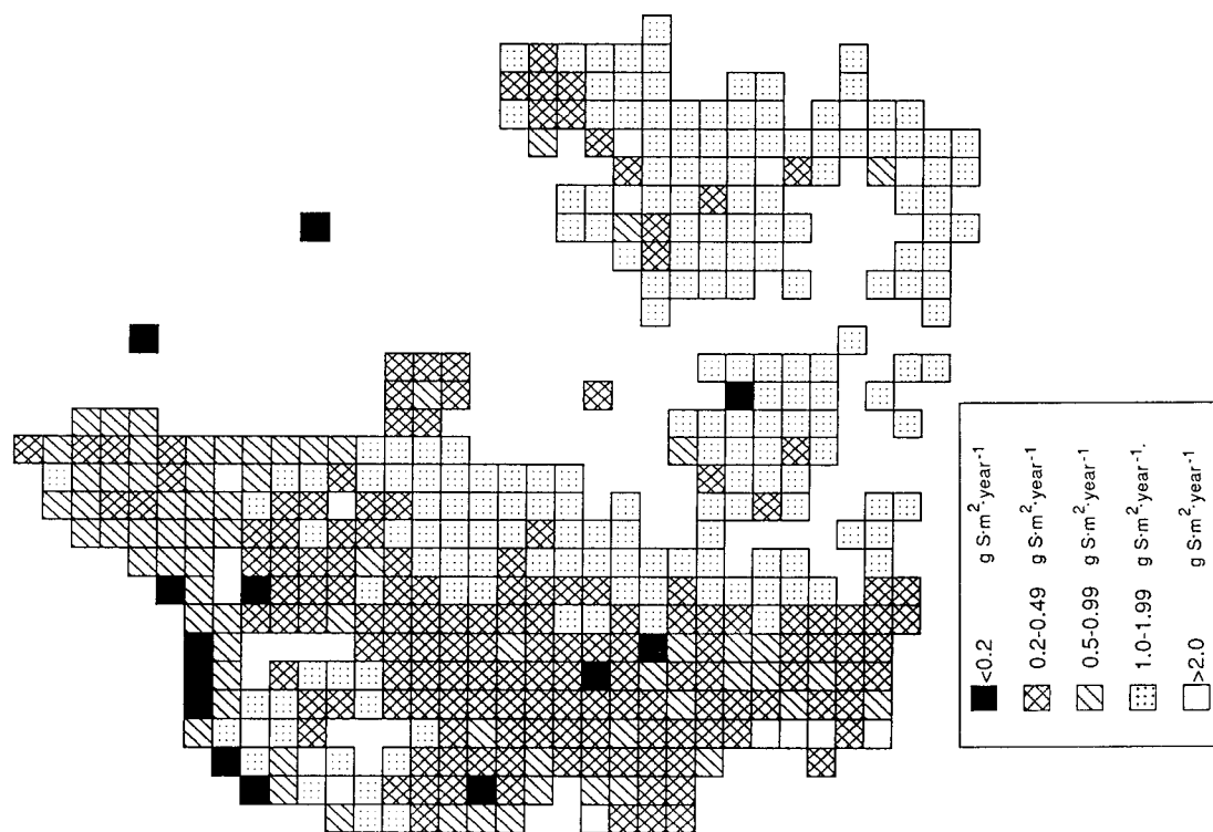
Figure A1.11. Denmark: Sulphur impact load (EMEP) for spruce when 50% of surplus nitrogen is leached.
