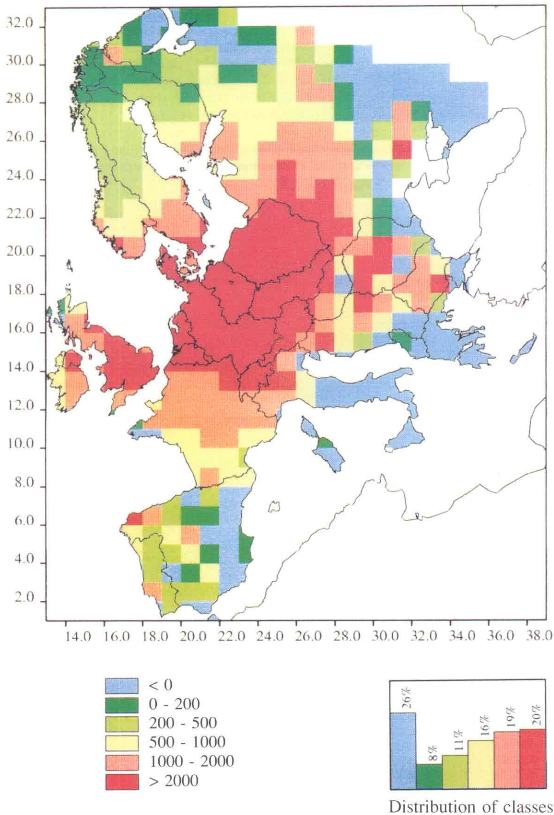
Figure 2.4a. Exceedance of the critical load of actual acidity (1 percentile). Units = equivalents \text{ha}^{-1} \text{yr}^{-1} .
