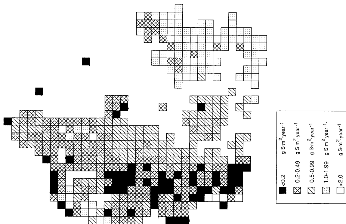
Figure A1.10. Denmark: Sulphur impact load (EMEP) for spruce when 100% of surplus nitrogen is leached.
