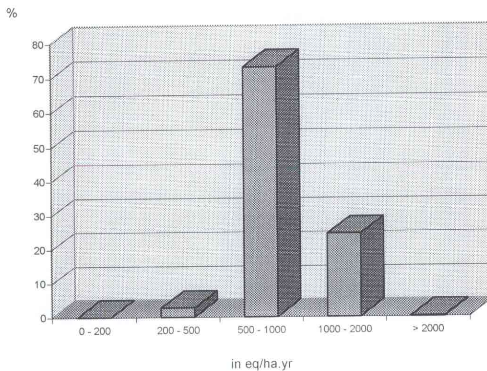
Figure AT-2. Distribution of classes of critical loads of nutrient nitrogen.
