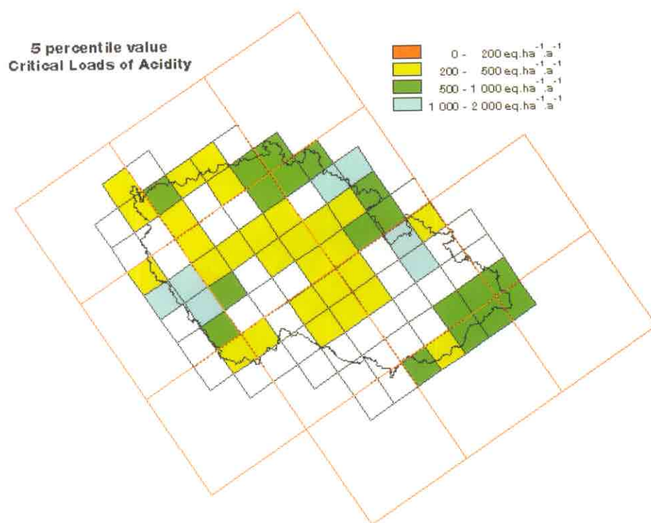
Figure CZ-1. Critical loads of acidity (5 percentile).
