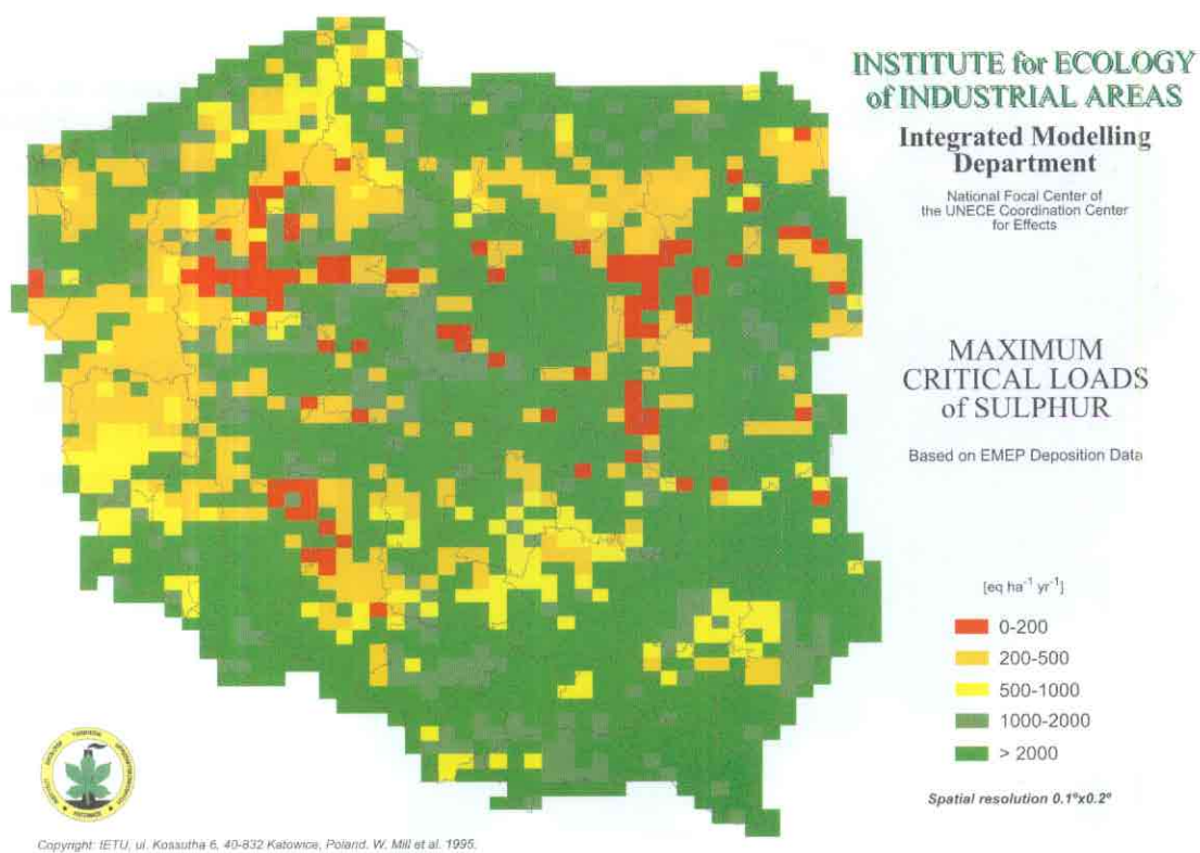
Figure PL-2. Maximum critical loads of sulfur.
