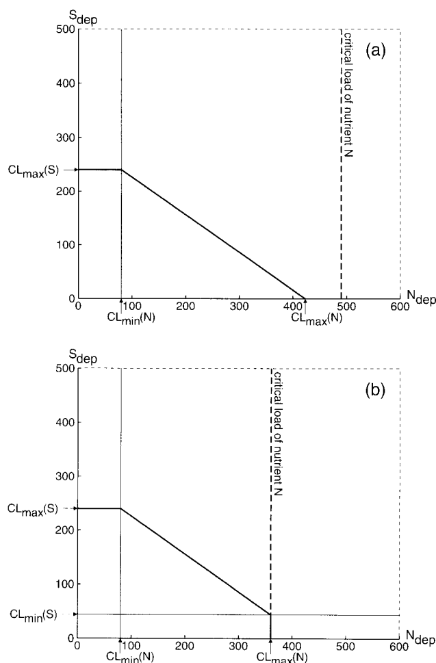
Figure 3.3. Relationship between sulfur and nitrogen deposition and the critical loads of acidifying N and S and the critical load of nutrient N: (a) CL_{nut}(N) > CL_{max}(N) , (b) CL_{nut}(N) < CL_{max}(N) . The grey area indicates deposition combinations causing no exceedance.
