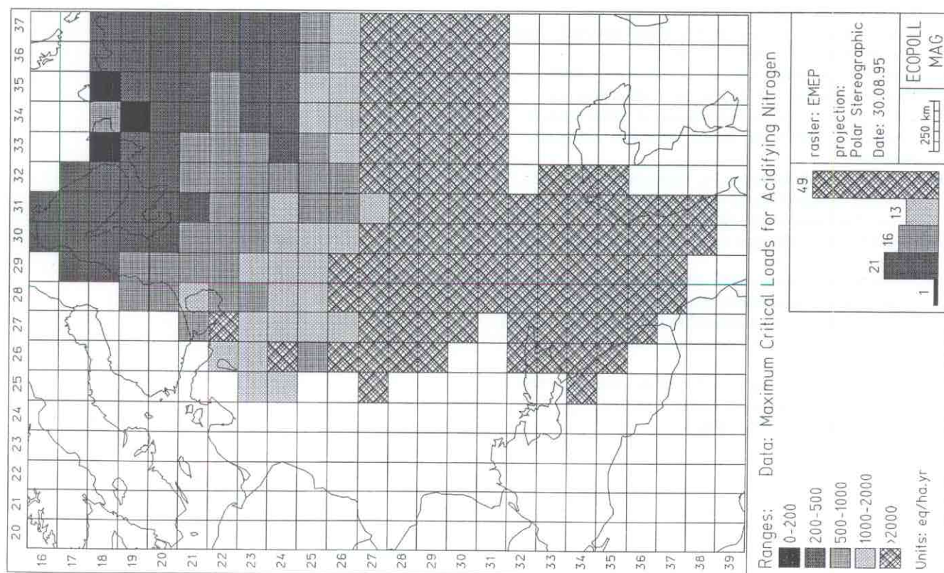
Figure RU-2. Maximum critical loads for acidifying nitrogen.
