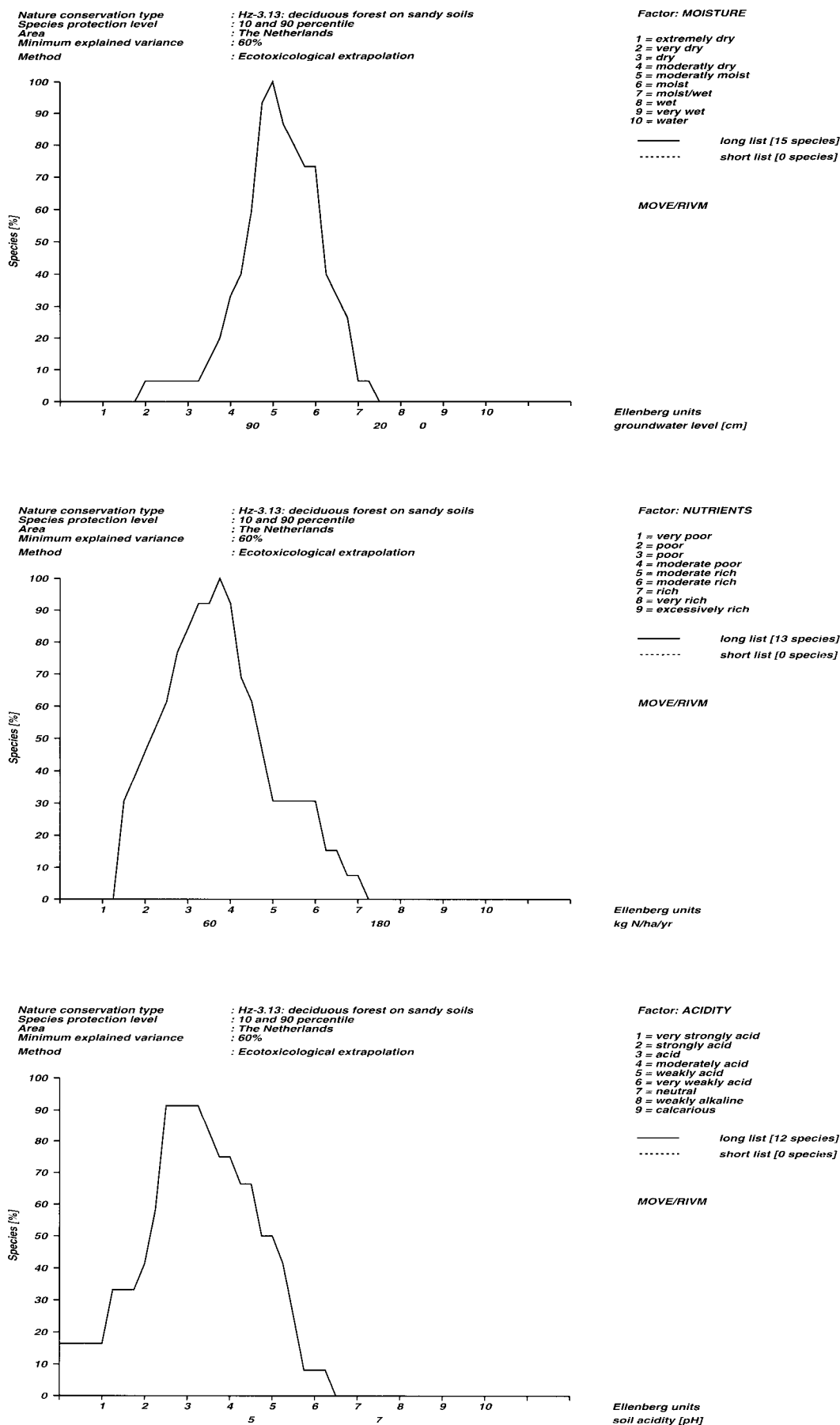
Figure 2. Percentage of the protected species of the nature conservation target type "nutrient-poor deciduous forest" as a function of nitrogen availability in the soil, soil moisture and soil acidity.
