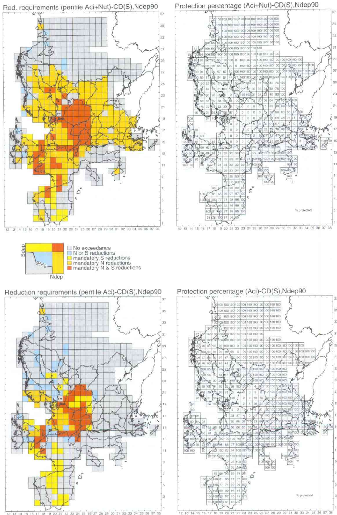
Figure 1.7. Using the critical sulfur deposition developed for the support of the Second Sulfur Protocol and CRP emission based depositions of oxidized and reduced nitrogen in 1990, the following graphs are shown: (a) Acidifying and eutrophying (sulfur and nitrogen based) deposition reduction requirements (upper left graph); (b) Ecosystem protection against acidification and eutrophication (upper right graph); (c) Acidifying deposition reduction requirements (lower left graph); (d) Ecosystem protection against acidification (lower right graph).
