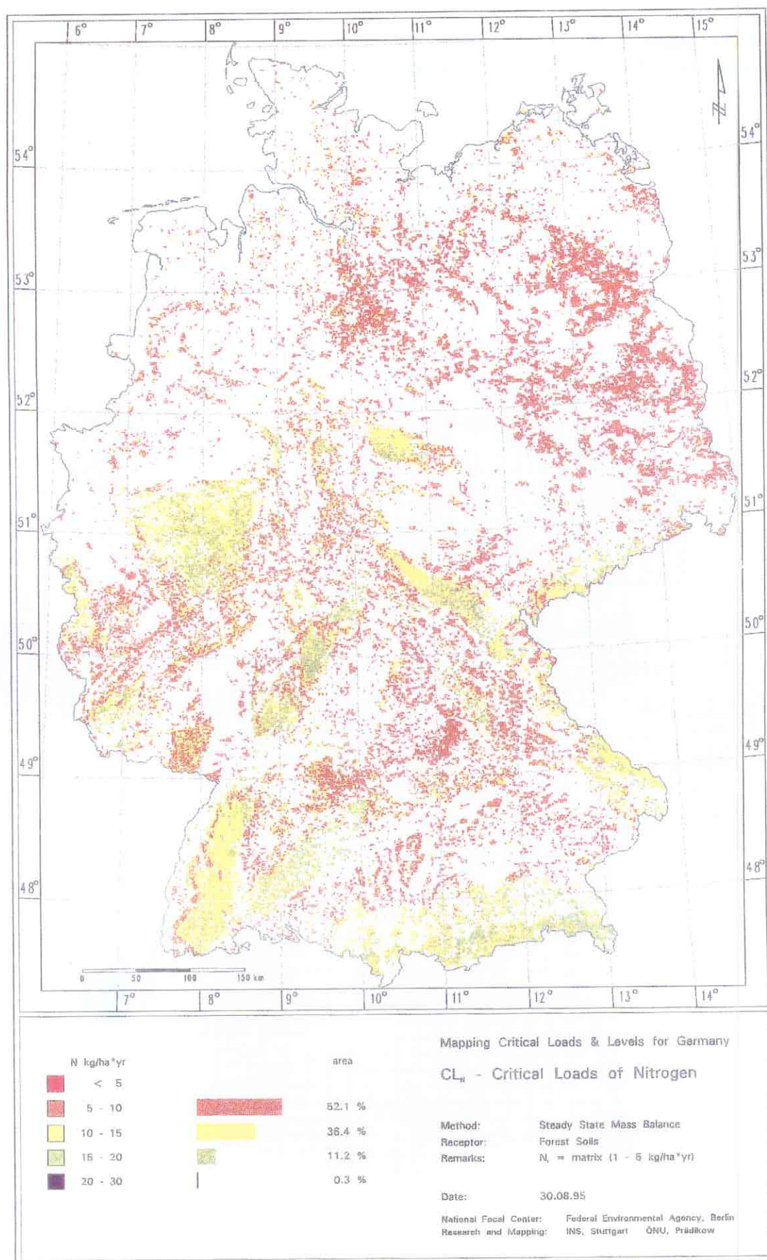
Figure DE-2. Critical loads of nutrient nitrogen for forest ecosystems ( \text{kg N ha}^{-1} \text{ yr}^{-1} ).
