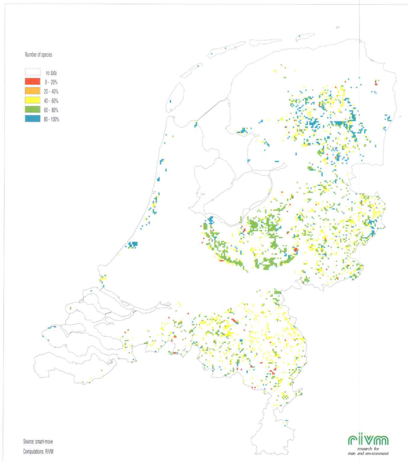
Figure 4. Predicted occurrence of plant species of deciduous forests as a function of modelled soil pH.
