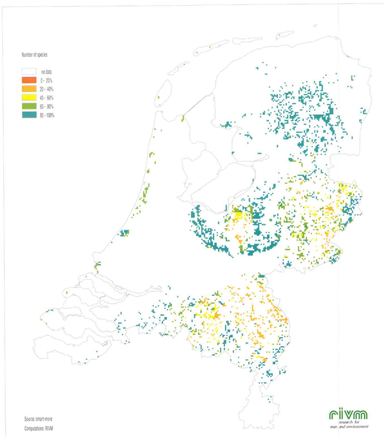
Figure 3. Predicted occurrence of plant species of deciduous forests as a function of modelled nitrogen availability.
