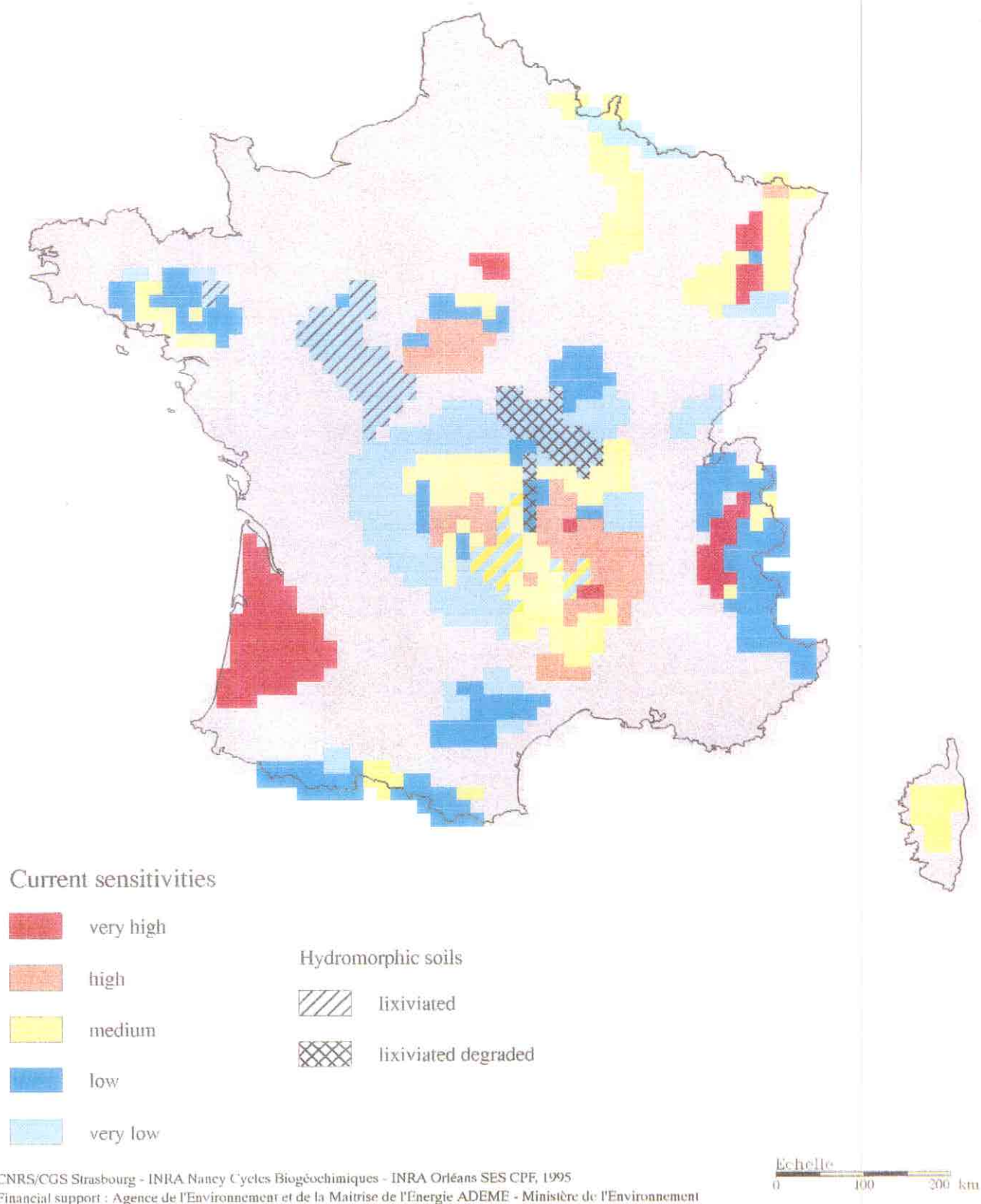
Figure FR-4. Current sensitivity of the French regions to the acid atmospheric deposition.
