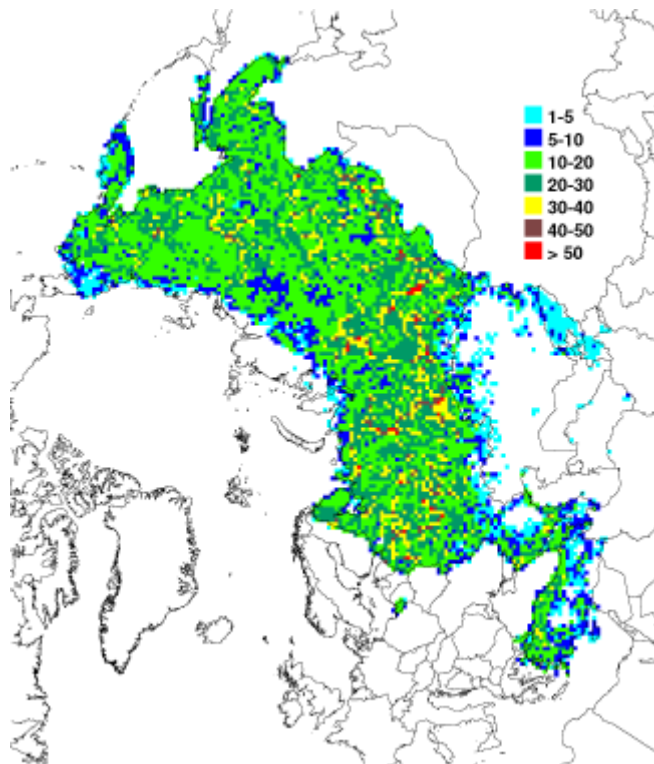
Figure 7-5. Number of receptors per EMEP grid cell.
