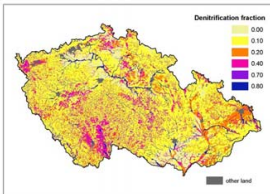
Figure CZ-1. Spatial distribution of denitrification factors for soil types of the Czech Republic.
