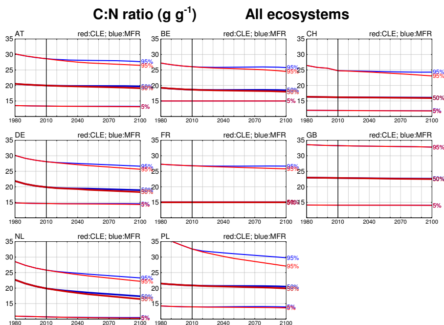
Figure 2-11. Temporal development of the 5 th , 50 th and 95 th percentile of the C:N ratio for all ecosystems in eight countries for two scenarios: CLE (red) and MFR (blue).
