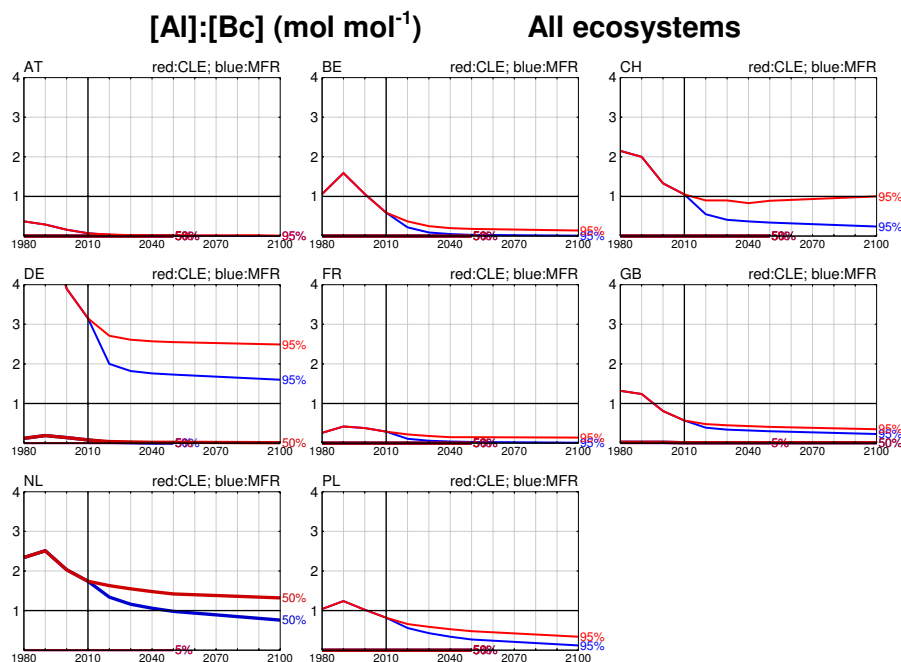
Figure 2-9. Temporal development of the 5 th , 50 th and 95 th percentile of the molar Al:Bc ratio for all ecosystems in eight countries for two scenarios: CLE (red) and MFR (blue).
