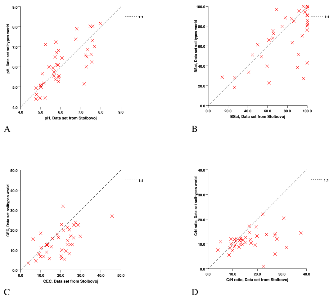
Figure 7-3. Comparison of soil attributes; pH (A), Base Saturation (B), CEC (C) and C/N ratio in the topsoil (D).
