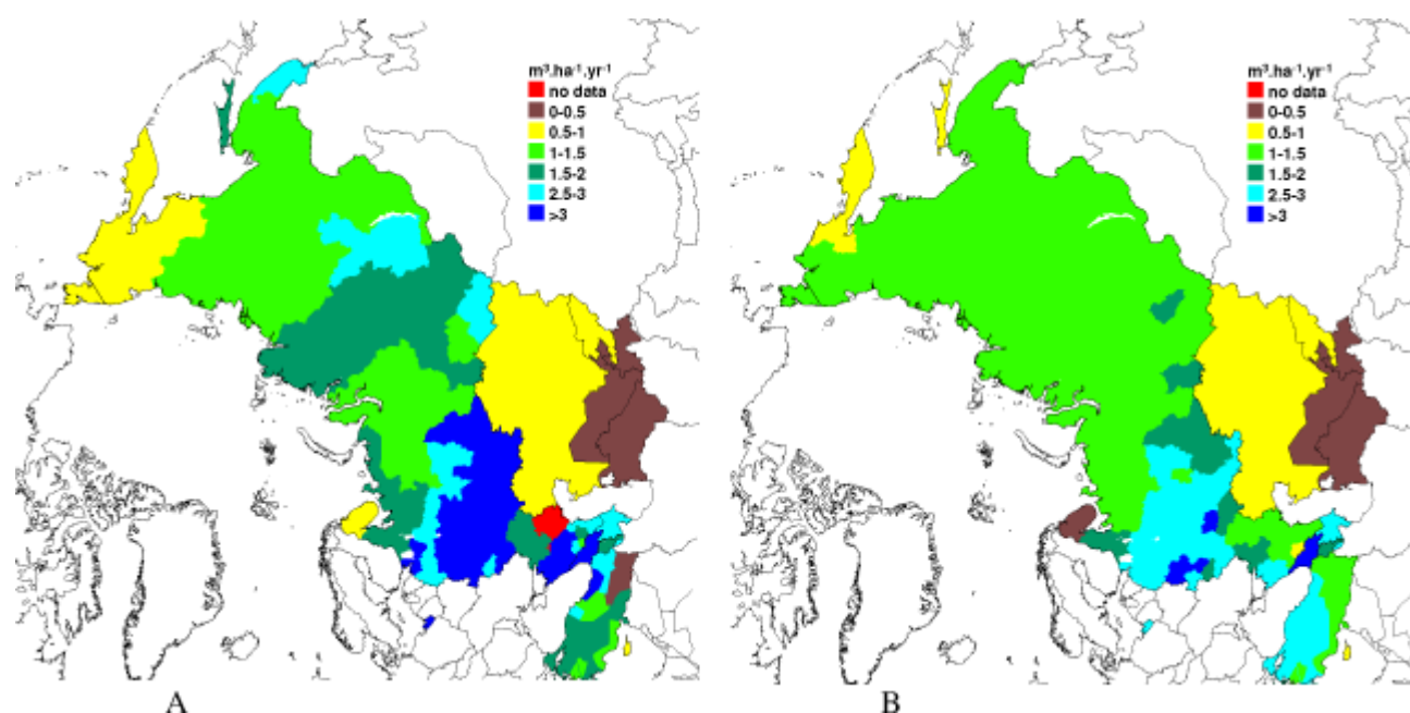
Figure 7-4. Average forest growth (A=conifers, B=broadleaves).
