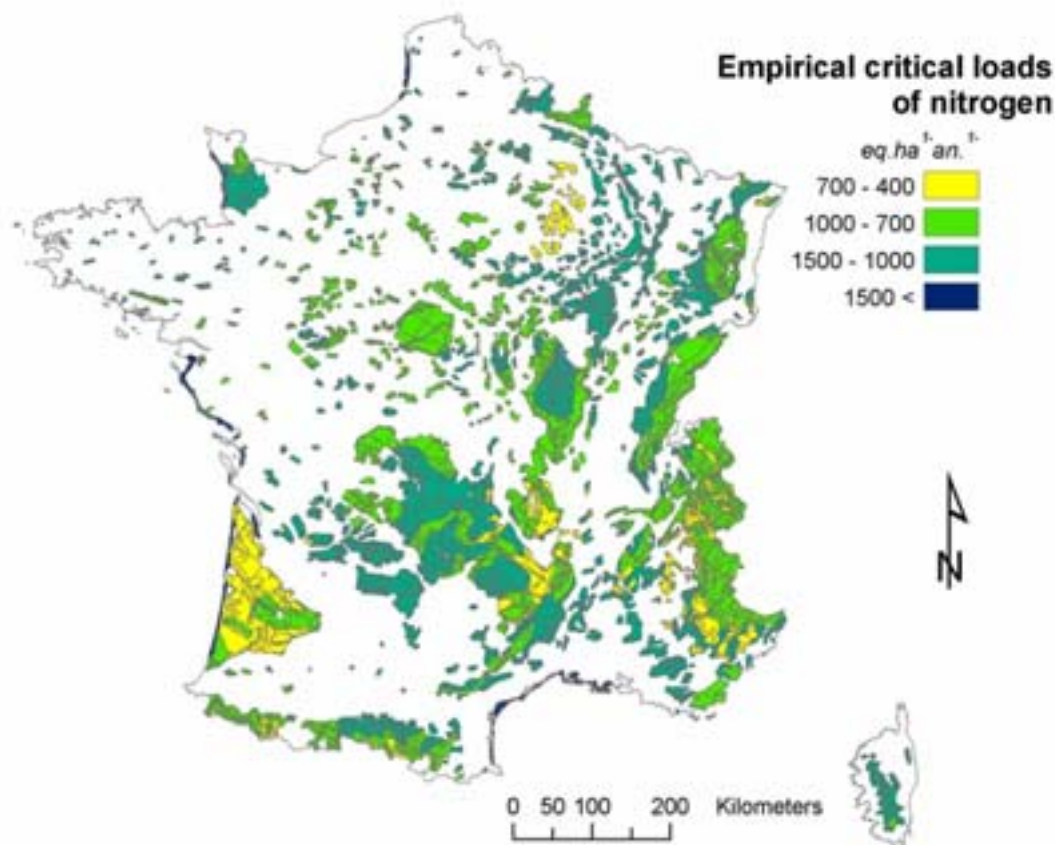
Figure FR-1. Map of empirical critical loads of nitrogen.
