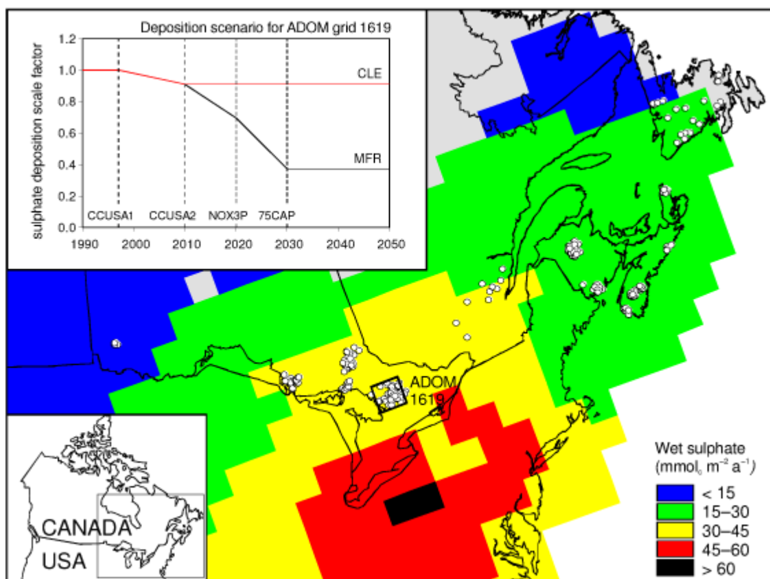
Figure CA-1. Wet deposition of sulphate in eastern North America as estimated using the Acid Deposition and Oxidant Model (ADOM). The ADOM is a comprehensive eulerian acid deposition model with a grid spacing of 127 km × 127 km (ADOM grid 1619 in south-central Ontario is shown). The location of the study lakes is also shown (white dots). The inset depicts the Current LEGislation (CLE) and Maximum Feasible Reductions (MFR) deposition scenarios for ADOM grid 1619 derived from several current and proposed control scenario (CCUSA1, CCUSA2, NOX3P and 75CAP).
