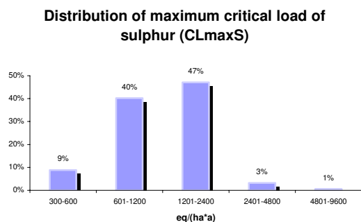
Figure LV-2. Distribution of CL_{maxS} concentrations.
