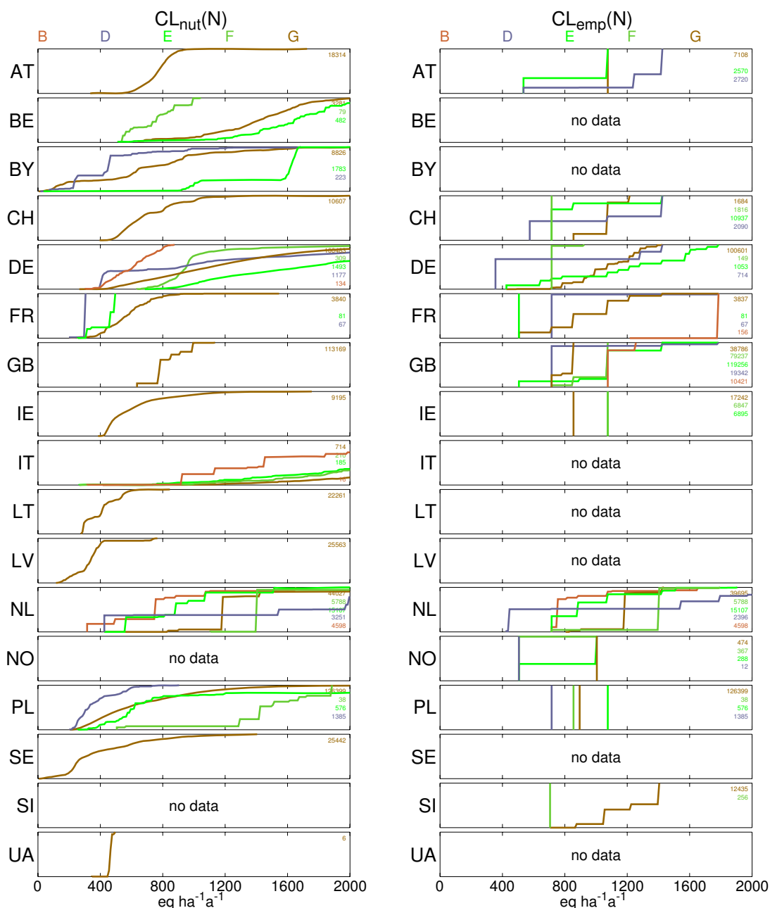
Figure 2-3. National distribution of CL nut N (left) and CL emp N (right) for most commonly considered EUNIS-1 ecosystems.
