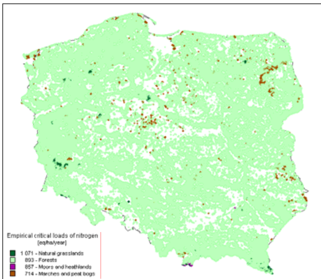
Figure PL-1. Spatial distribution of empirical critical loads of nitrogen.
