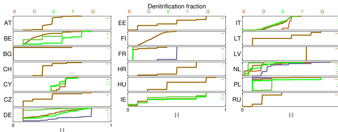
Figure 2-20. Distributions of the denitrification fraction ( fde ).
