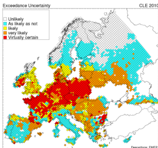
Figure 4-2. The likelihood that the Average Accumulated Exceedance of an EMEP grid cell exceeds zero, i.e. that it contains at least one ecosystem of which the critical load of nutrient N is exceeded with current legislation.
