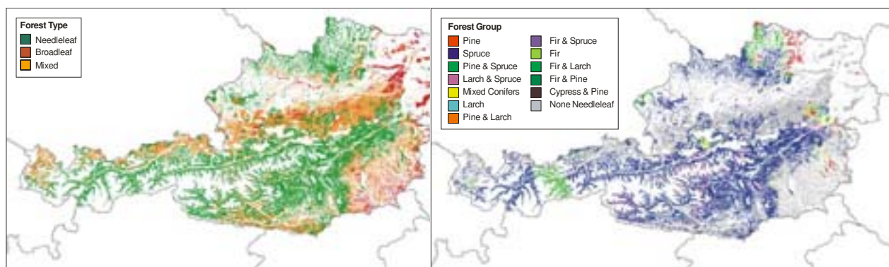
Figure 5-4. Clipping of Thiessen polygons based on Corine 2000 class boundaries to derive forest species and type information.
