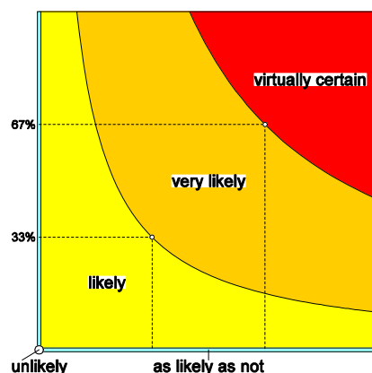
Figure 4-1. The likelihood scale indicating the simultaneous probability of an exceedance of the empirical critical load and the modelled critical load of nutrient nitrogen.
