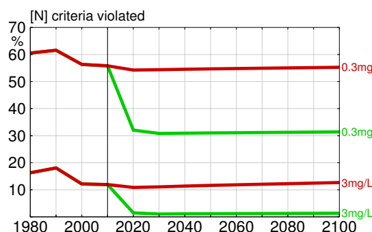
Figure 3-6. Temporal development of the European ecosystem area (expressed as percent of total area) for which the N concentration violates two criteria ( [N]_{acc}=0.3 and [N]_{acc}=3 mg N L -1 ) for the CLE (red) and MFR (green) scenarios.
