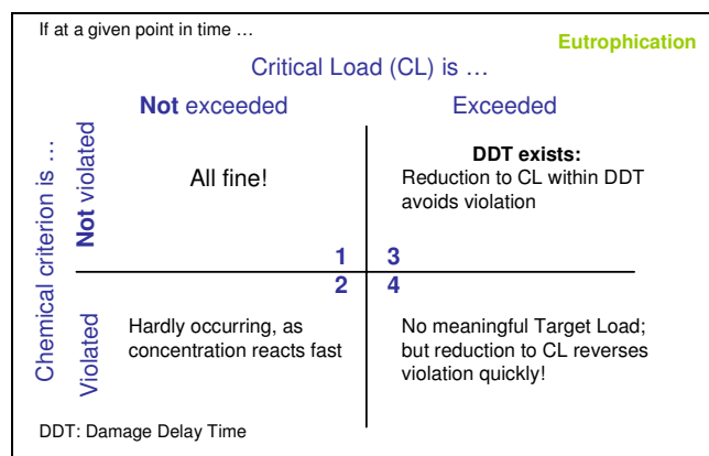
Figure 3-7. Possible combinations of critical load (non-)exceedance and criterion (non-)violation.
