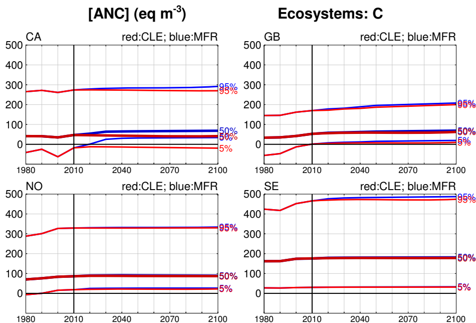
Figure 2-10. Temporal development of the 5 th , 50 th and 95 th percentile of ANC in surface waters (EUNIS-code C) in four countries for two scenarios: CLE (red) and MFR (blue).
