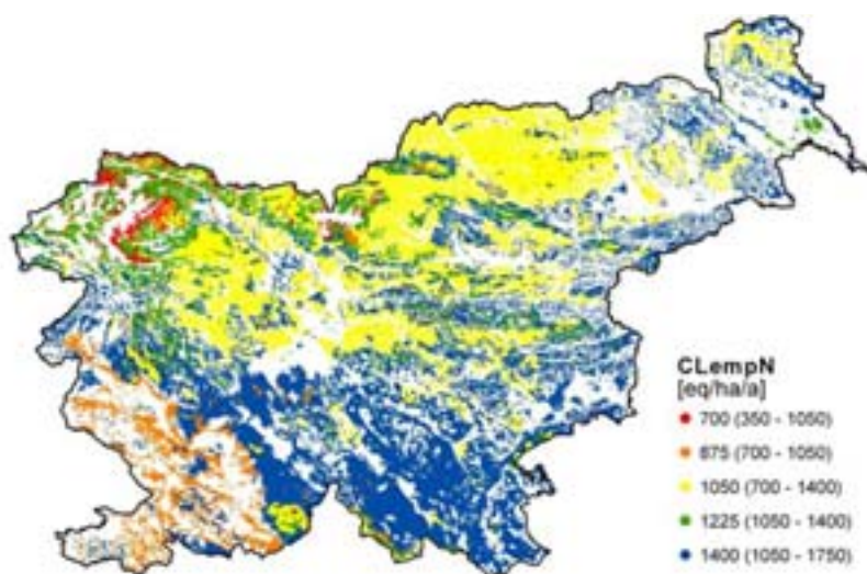
Figure SI-1. Empirical critical loads of nitrogen for forests.
