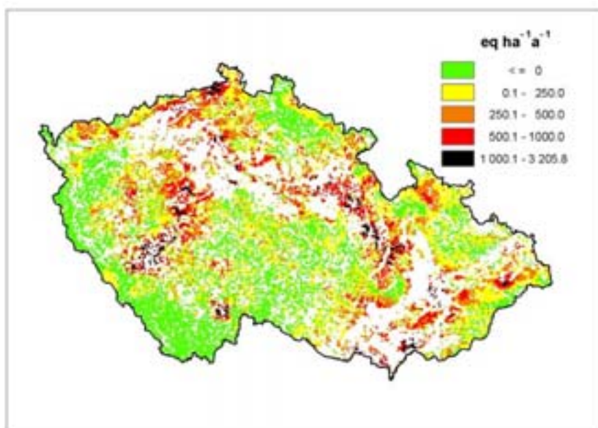
Figure CZ-3. Critical load exceedances for nutrient nitrogen.
