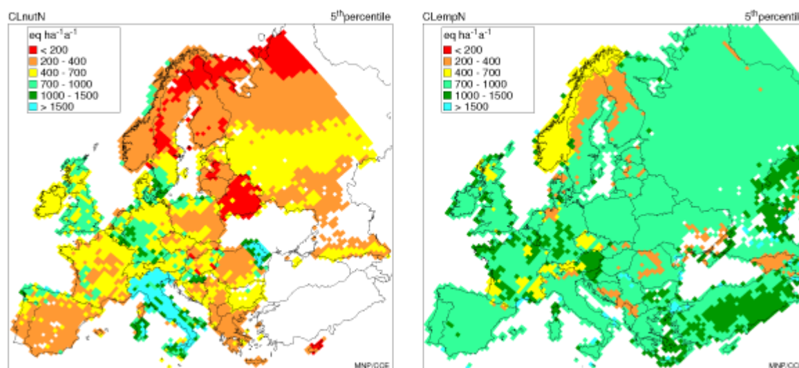
Figure 1-1. The 5 th percentiles of the modelled critical loads of nutrient nitrogen for all ecosystems (left) and of the empirical critical loads (right) on the EMEP50 grid.
