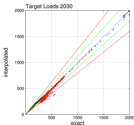
Figure 3-12. Exact versus interpolated target loads (in eq/ha/a). The black and red crosses show TLs entering ('TLS') and leaving ('TLN'), respectively, the rectangle defined by the deposition scenarios. The green and red lines show the 10% and 20% deviation, respectively, from the blue 1-to-1 line.
