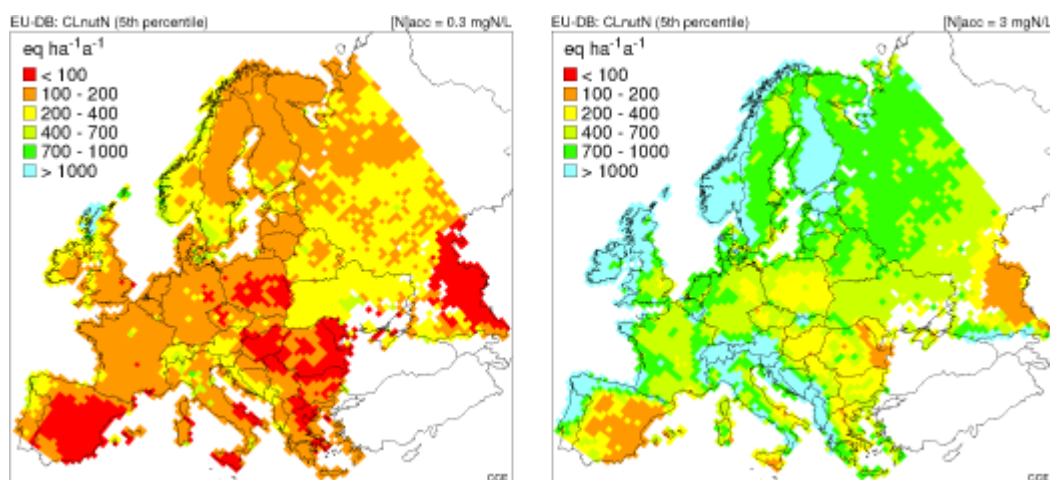
Figure 3-1. 5 th percentile of the critical loads of nutrient nitrogen, CL_{nutN} , on the EMEP50 grid computed with the European background data base (EU-DB) and two different acceptable nitrogen concentrations: 0.3 \text{ mg N L}^{-1} (left) and 3 \text{ mg N L}^{-1} (right).
