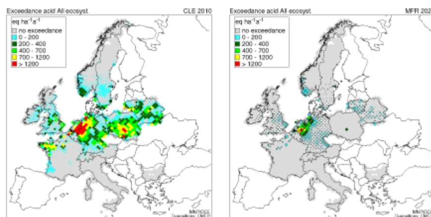
Figure 2-8. Exceedance of critical loads of acidity CLE 2010 (left) and MFR 2020 (right).
