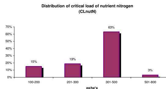
Figure LV-5. Distribution of CL_{nutN} .
