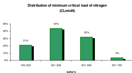
Figure LV-4. Distribution of CL_{minN} .
