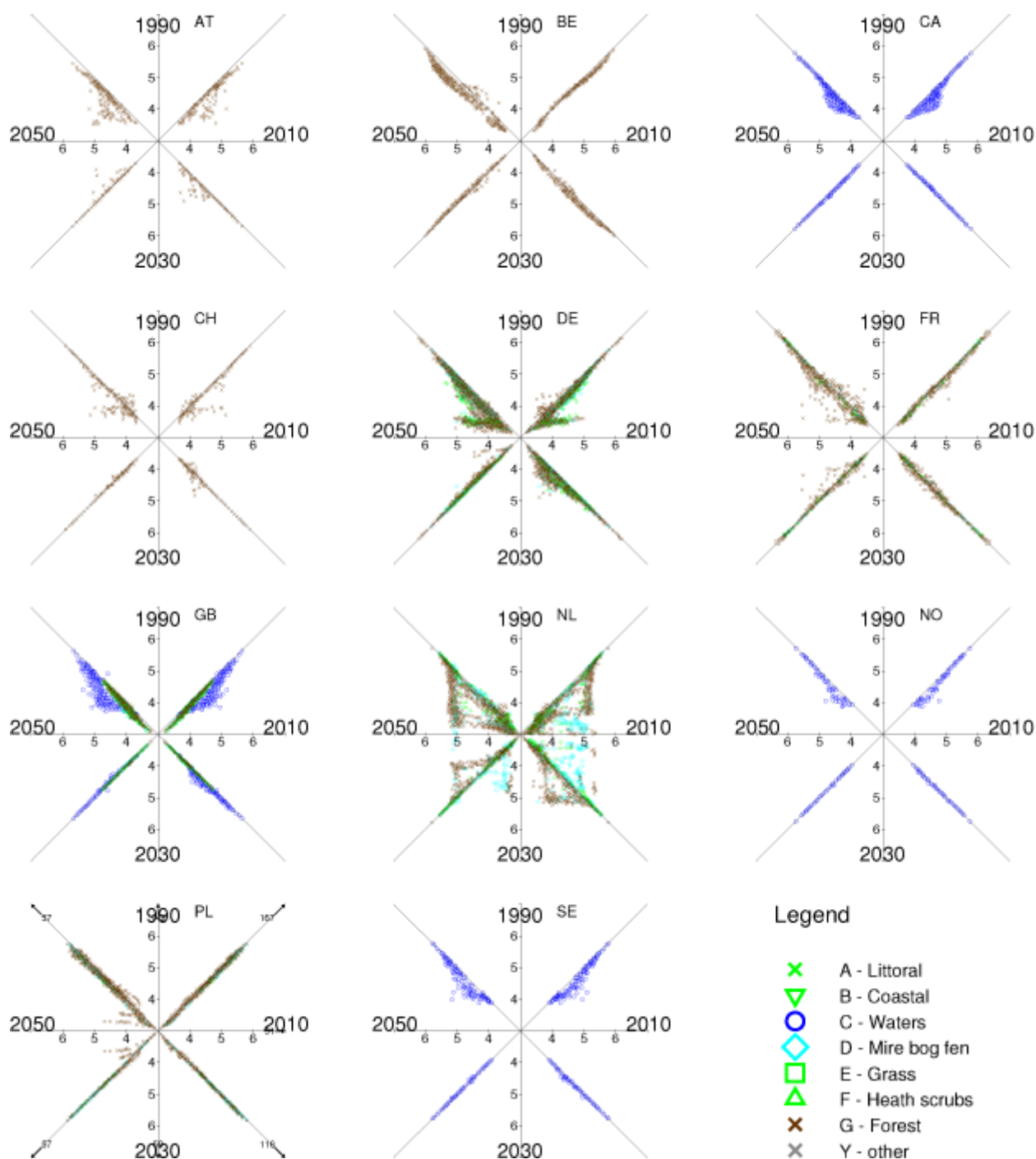
Figure 2-14. Four year-to-year correlations (windmill plots) of the soil/lake pH from dynamic modelling of all ecosystems (ca. 550,000) and the CLE scenario, distinguished by their EUNIS class.
