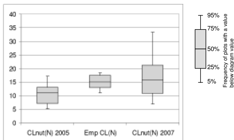
Figure DE-4. Comparison of Nitrogen Critical Load values, data calculation 2005, empirical Critical Loads and data calculation of 2007.
