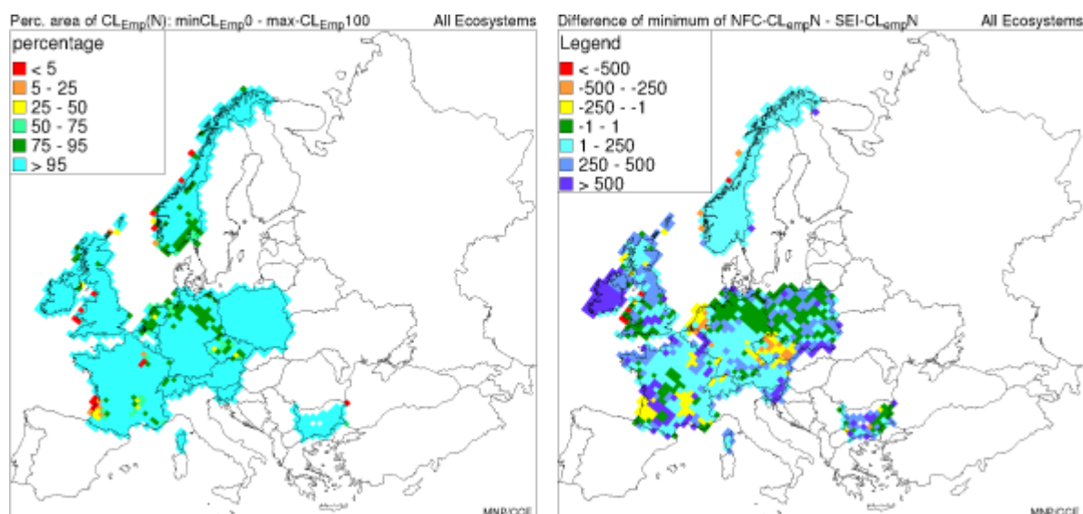
Figure 6-9. Left: Percentage of NFC-sites of which the CL emp N is within the range of CL emp N of the SEI-map; Right: Difference of minimum critical load (eq ha -1 a -1 ) between the NFC-CL emp N and the CL emp N of the SEI-map.
