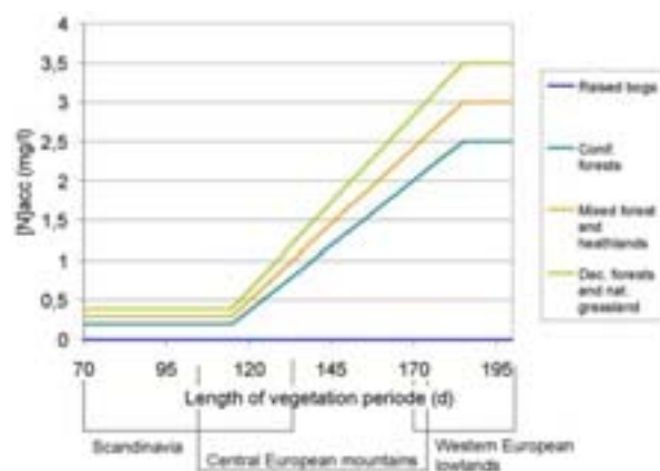
Figure DE-3. Critical (acceptable) N concentrations in soil solution for calculating CL nutN .
