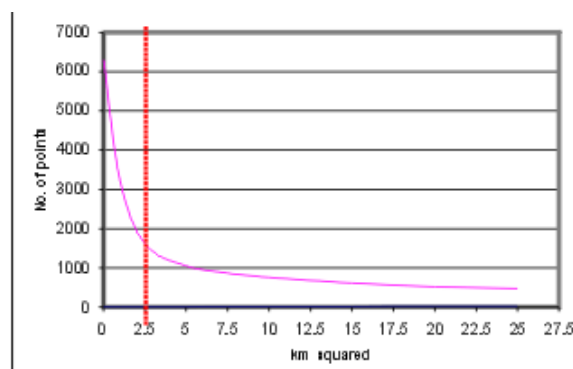
Figure 5-2. Comparison of centroid numbers and area of originating polygons.
