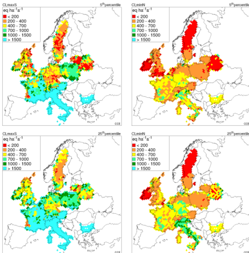
Figure 2-5. The 5 th (top) and 25 th (bottom) percentile maps of CL_{maxS} (left) and CL_{minN} (right).
