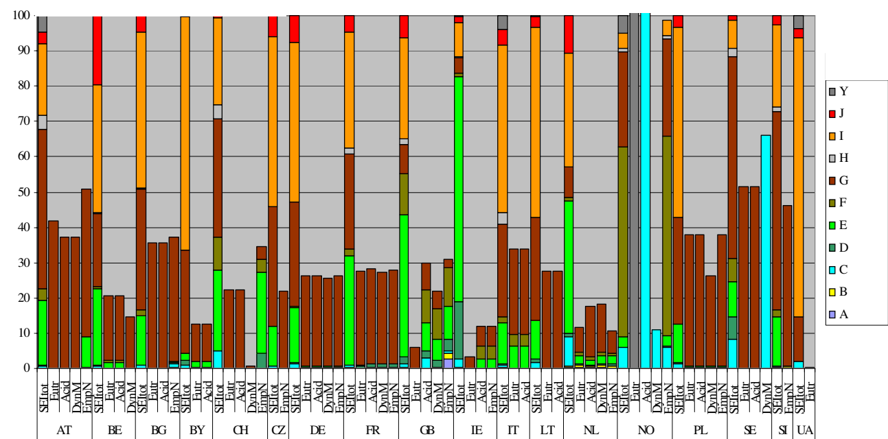
Figure 2-1. National distributions of ecosystem types as percent of total country area according to the harmonised land cover map (SEItot) and for the submissions for CLnutN (Eutr), CLempN (EmpN), CLmaxS (Acid) and dynamic modelling (DynM).
