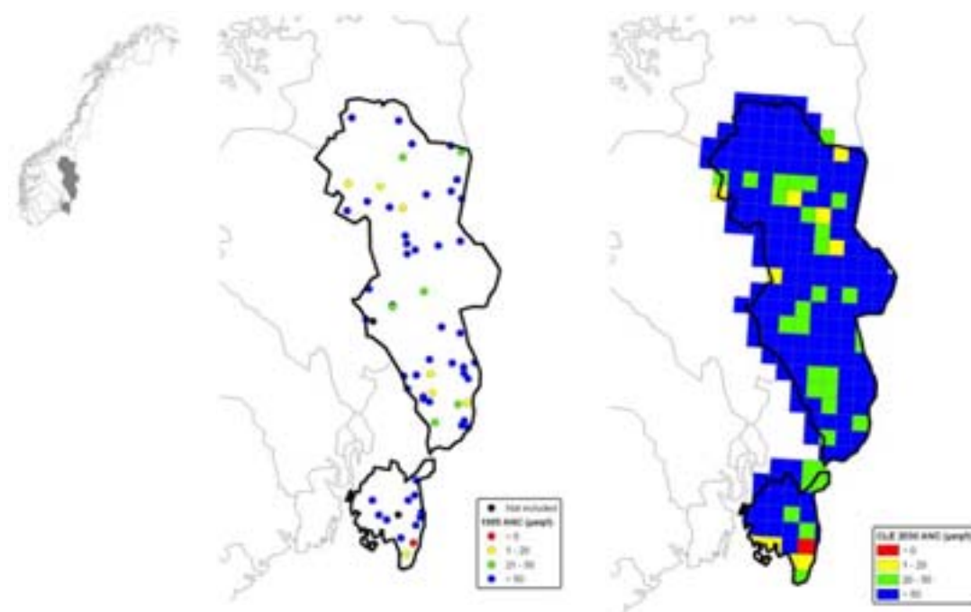
Figure NO-1. Left map: Observed ANC in 1995 for each calibrated lake. Right map: Modelled ANC in 2030 according to the CLE scenario for each 'grid cell lake'. Open circle on the left map show: disregarded lake due to very high phosphorus concentrations (and ANC) from local pollution: Stomperudtjern (128-I-4) and Kinnlitjernet (412-I-20).
