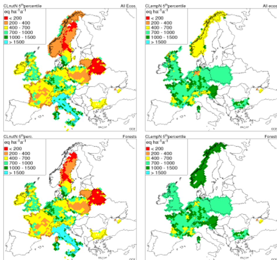
Figure 2-2. Submitted critical loads of nitrogen, modelled at the left and empirical at the right; for all ecosystems at the top and for forests only at the lower half of the figure.
