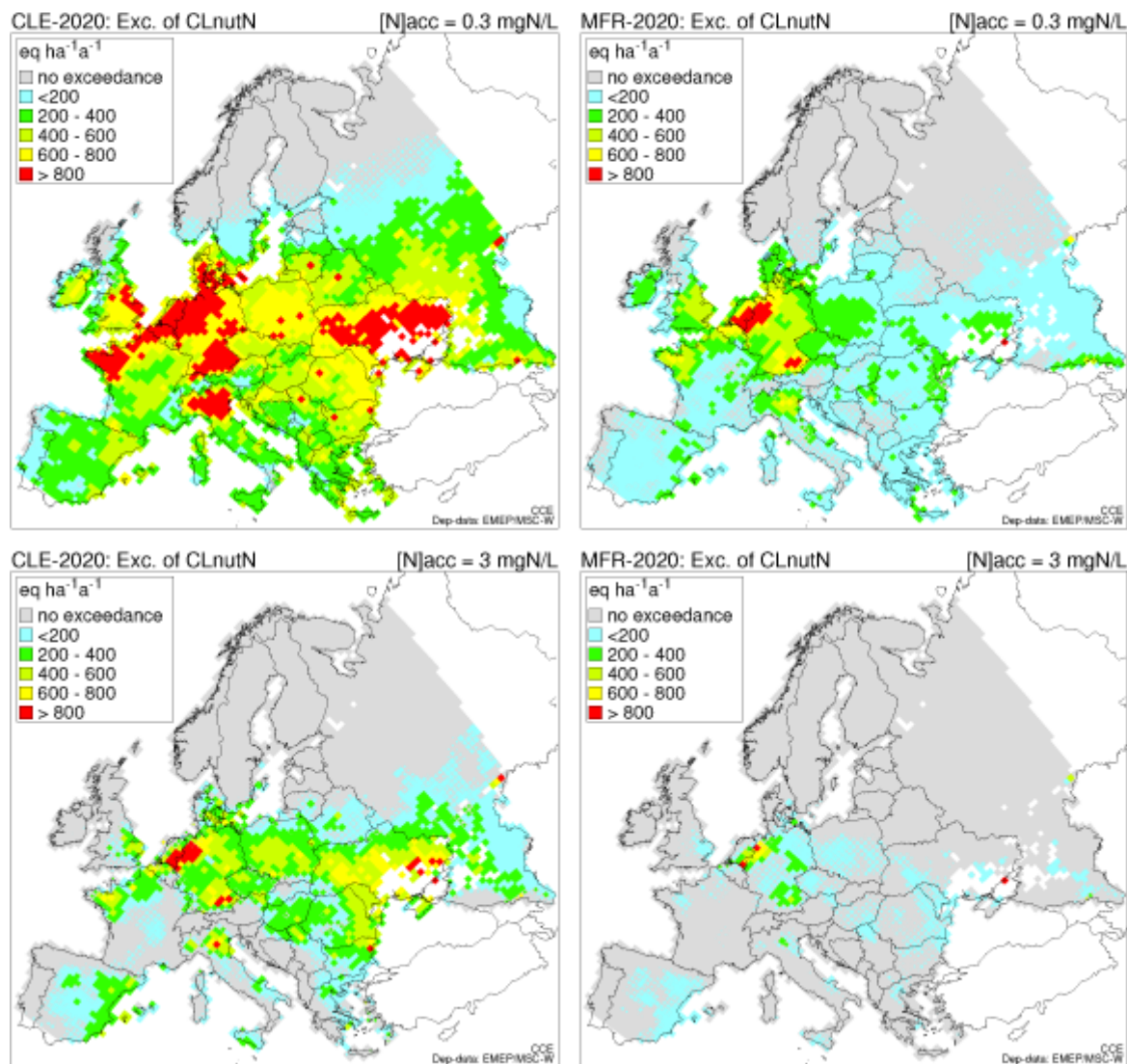
Figure 3-3. Exceedance (AAE) of CLnutN in 2020 computed with the EU-DB for the CLE (left) and MFR (right) scenarios and two different acceptable nitrogen concentrations: 0.3 \text{ mg N L}^{-1} (top) and 3 \text{ mg N L}^{-1} (bottom). Note: The size of the coloured grids is proportional to the percentage of ecosystem area exceeded in the grid.
