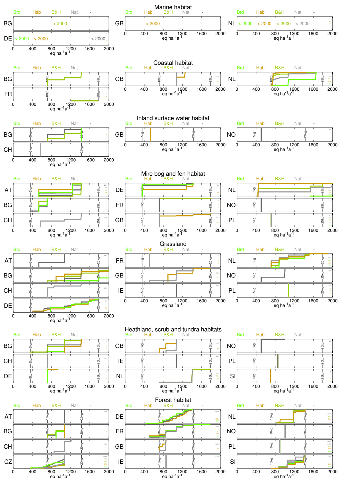
Figure 2-4. Empirical critical loads of areas protected by the birds directive, the habitat directive, both the bird and habitat directive, other (national) nature protection legislation or no protection.
