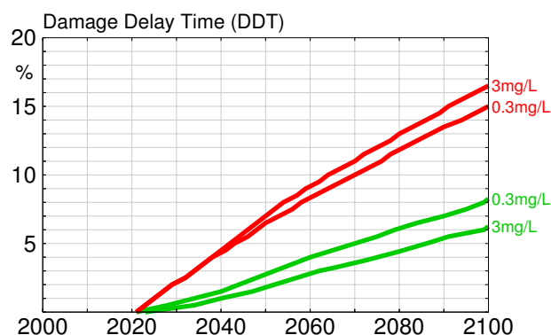
Figure 3-9. Cumulative distribution of Damage Delay Times (DDTs) for the CLE (red) and MFR (green) scenarios and two criteria ( [N]_{acc}=0.3 and [N]_{acc}=3 \text{ mg N L}^{-1} ). Note that the percentages in this figure are relative to the percentages for category 3 in Table 3-1.
