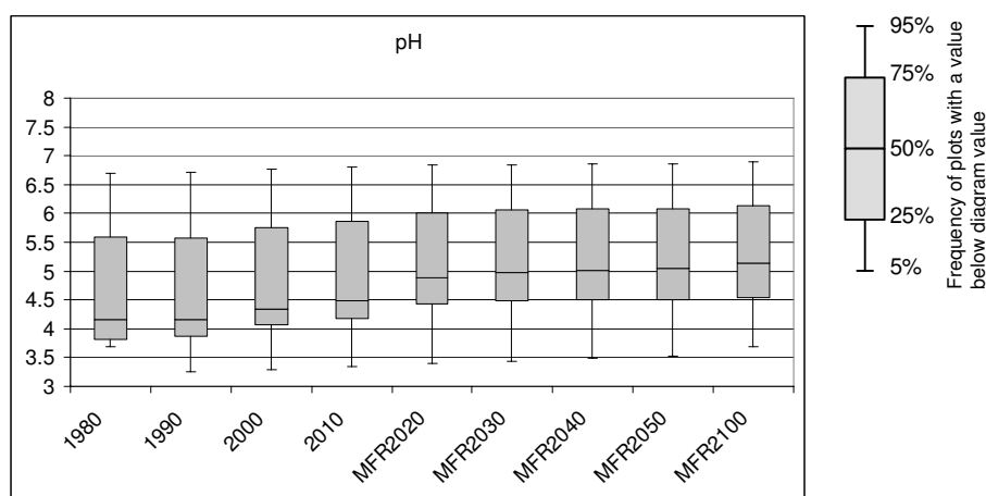
Figure DE-6. Trend of the distribution of pH values in Germany following the 'maximal feasible reduction' deposition scenario (101098 plots calculated).
