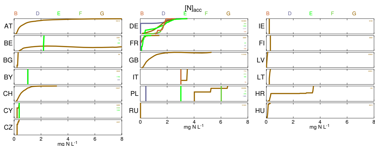
Figure 2-18. Distribution of the acceptable nitrogen concentration submitted, or calculated from submitted acceptable leaching nitrogen flux and Q_{le} , for the most often considered ecosystem types.
