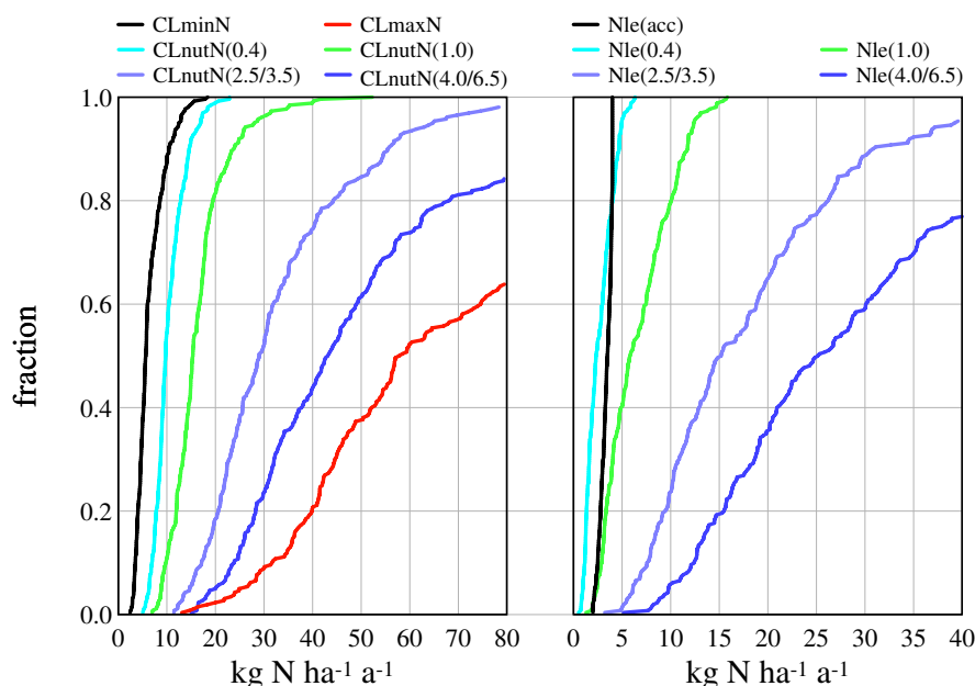
Figure CH-2. Cumulative frequency distributions of Nutrient N critical loads (left) and N leaching rates (right) under different critical concentrations in soil solution.
