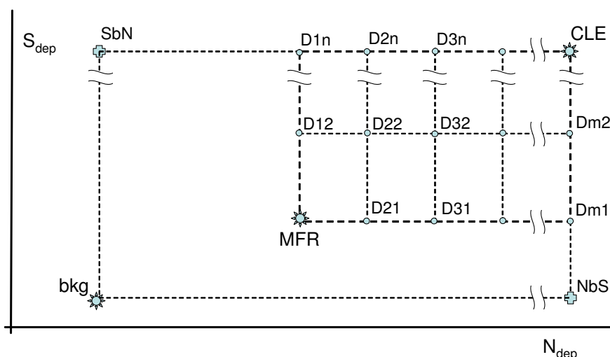
Figure 1: Graphic representation in the (N_{\text{dep}}, S_{\text{dep}}) -plane of the N and S deposition scenarios for 2020–2100 derived from the CLE, MFR and bkg scenarios. Also shown is the naming of the scenarios (Note: D11=MFR, Dmn=CLE, m between 1 and (max.) 6, n between 1 and (max.) 4).
