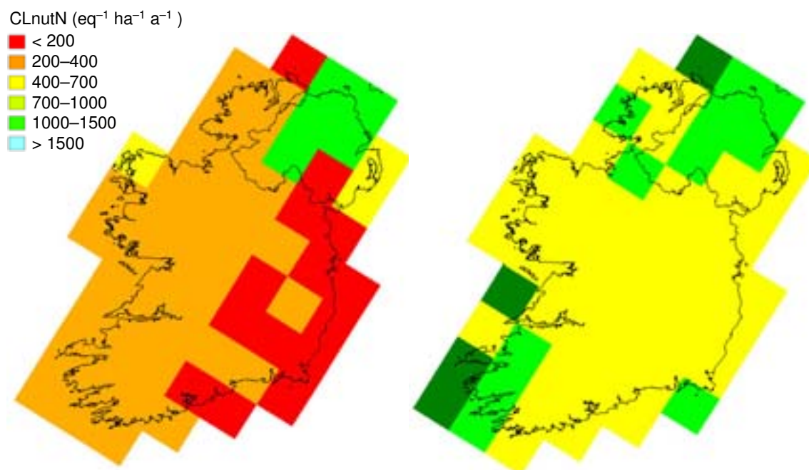
Figure IE-1. Critical loads of nutrient nitrogen (CLnutN) under the 2005 data call (left) and the 2007 voluntary data call (right). Northern Ireland is shown for completeness (2005 data); ecosystems are similar across both regions indicating that critical loads should be consistent. The CLnutN data submitted to the 2007 voluntary call (right) are consistent with the United Kingdom (i.e. Northern Ireland) data.
