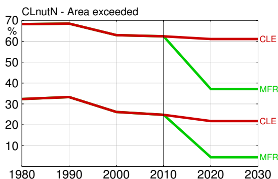
Figure 3-4. Temporal development of the European ecosystem area exceeded (expressed as percent of total) for CLnutN using EU-DB and the CLE (red) and MFR (green) scenarios. The upper curve(s) are for [N]_{acc} = 0.3 \text{ mg N L}^{-1} and the lower ones for [N]_{acc} = 3 \text{ mg N L}^{-1} .
