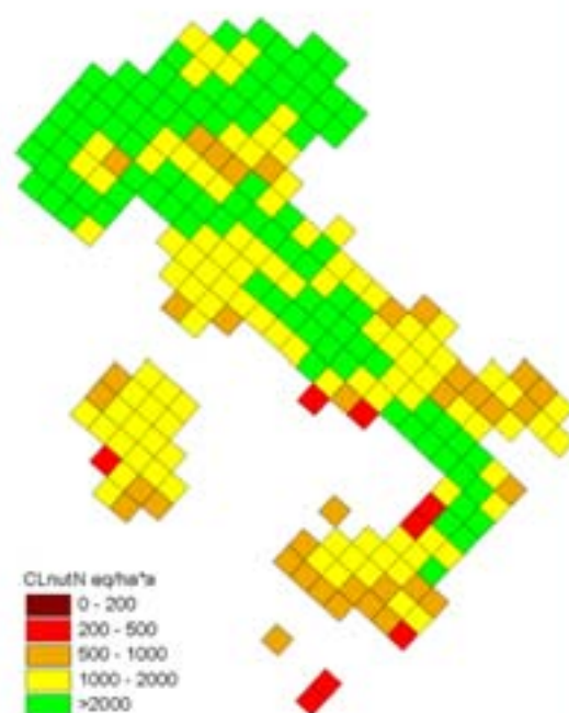
Figure IT-2. Critical load of nutrient nitrogen.
