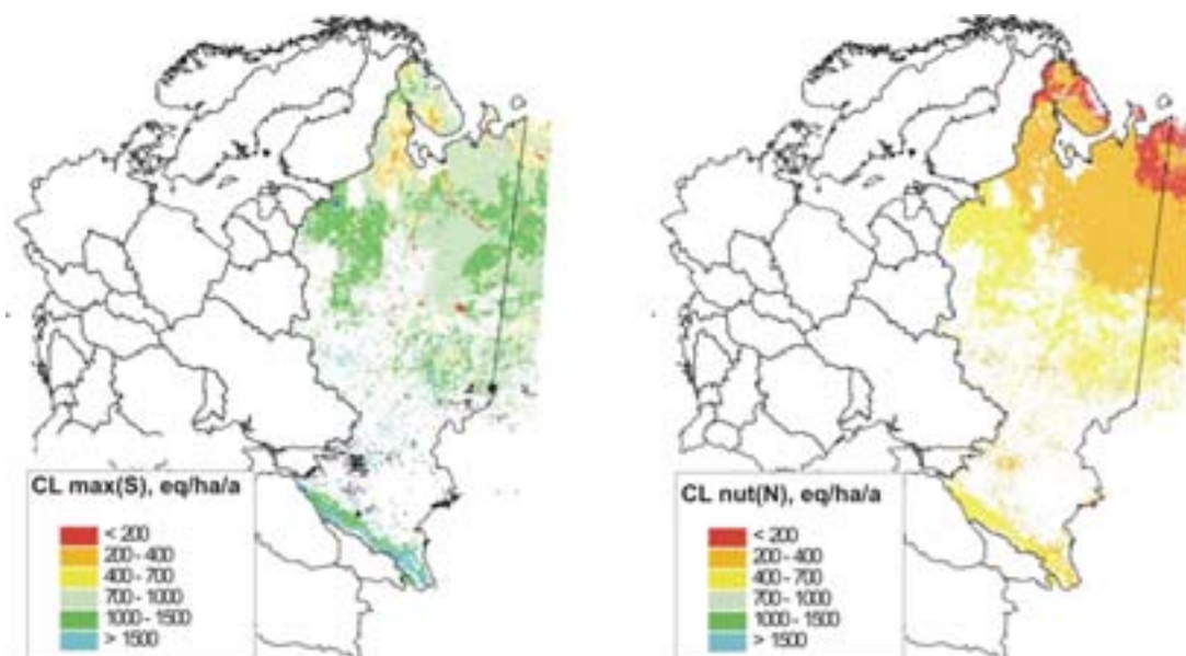
Figure RU-1. Critical loads for acidity (left) and nutrient nitrogen (right) for forest ecosystems of European Russia.
