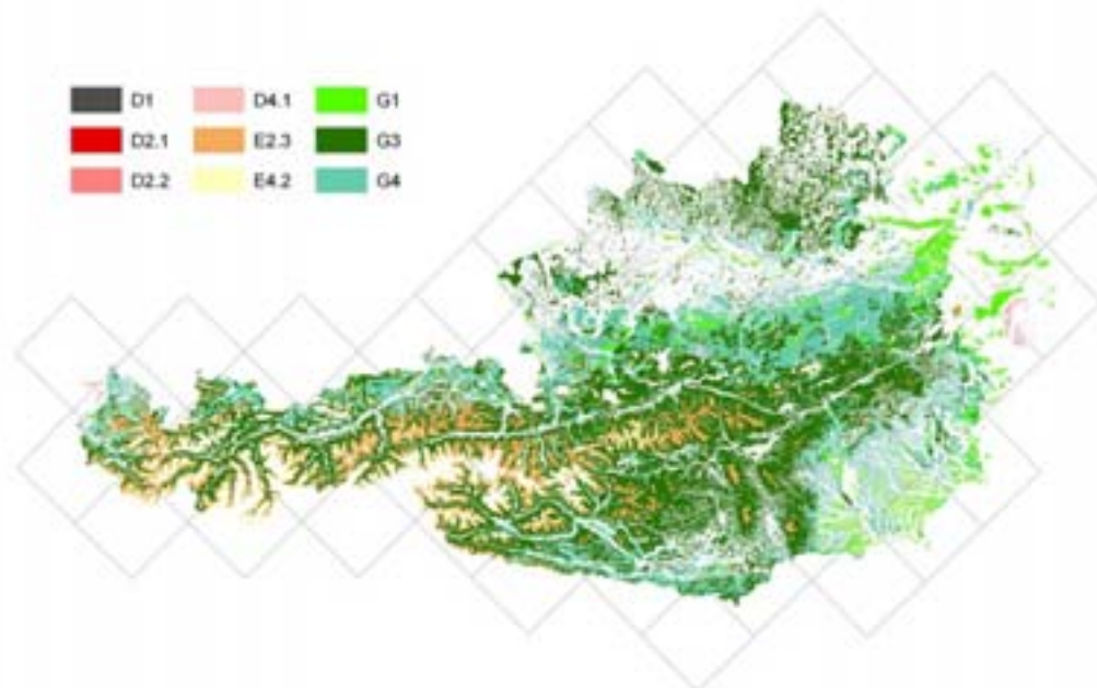
Figure AT-1. Natural and semi-natural habitats in Austria (Corine Land Cover 2000).
