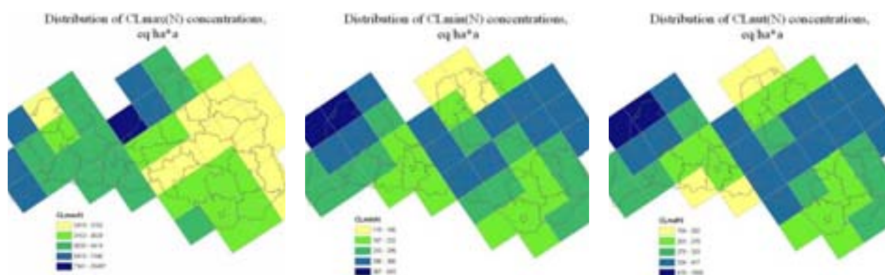
Figure LV- 6. Average CL_{maxN} , CL_{minN} and CL_{nutN} in EMEP grid cells.
