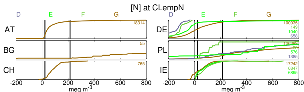
Figure 2-19. Fictive nitrogen concentrations, based on empirical critical loads and SMB input parameters.
