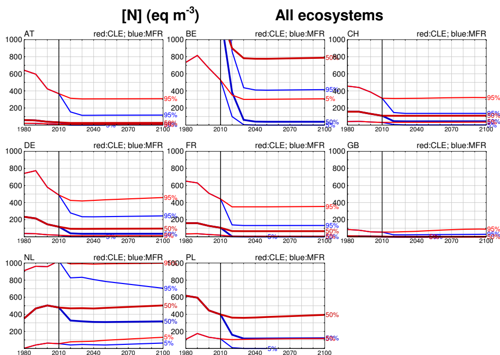
Figure 2-12. Temporal development of the 5 th , 50 th and 95 th percentile of the total N concentration in solution for all ecosystems in eight countries for two scenarios: CLE (red) and MFR (blue).
