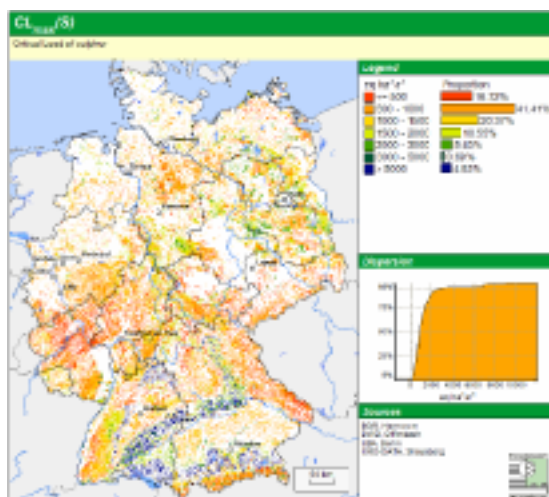
Figure DE-1. Critical load of sulphur, CL maxS .
