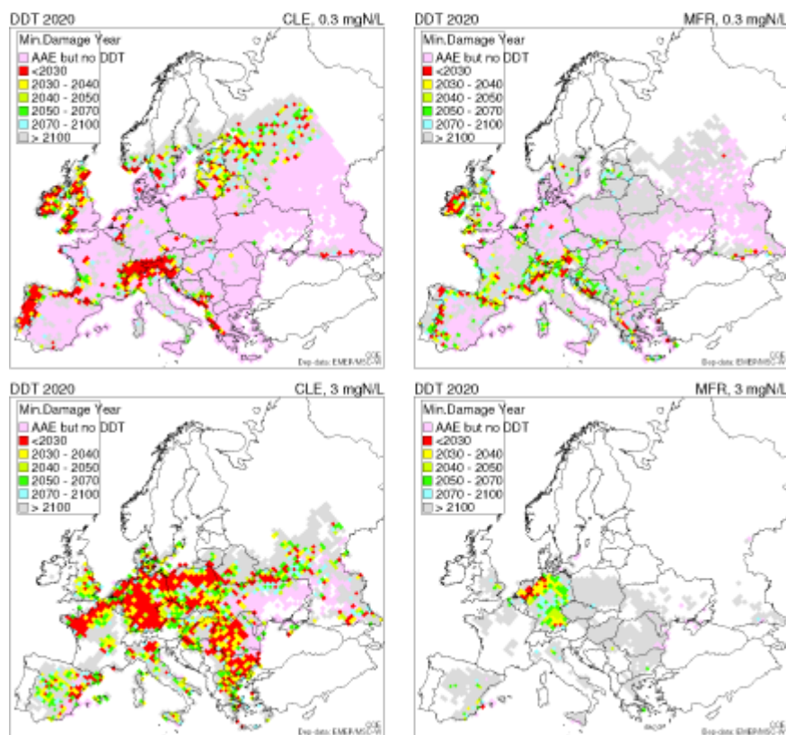
Figure 3-10: Minimum Damage Delay Time (DDT) after 2020 in every EMEP grid cell. The pink area indicates grid cells with exceedance but no DDT, the white areas where there is no exceedance or no data (see also Figure 3-3).
