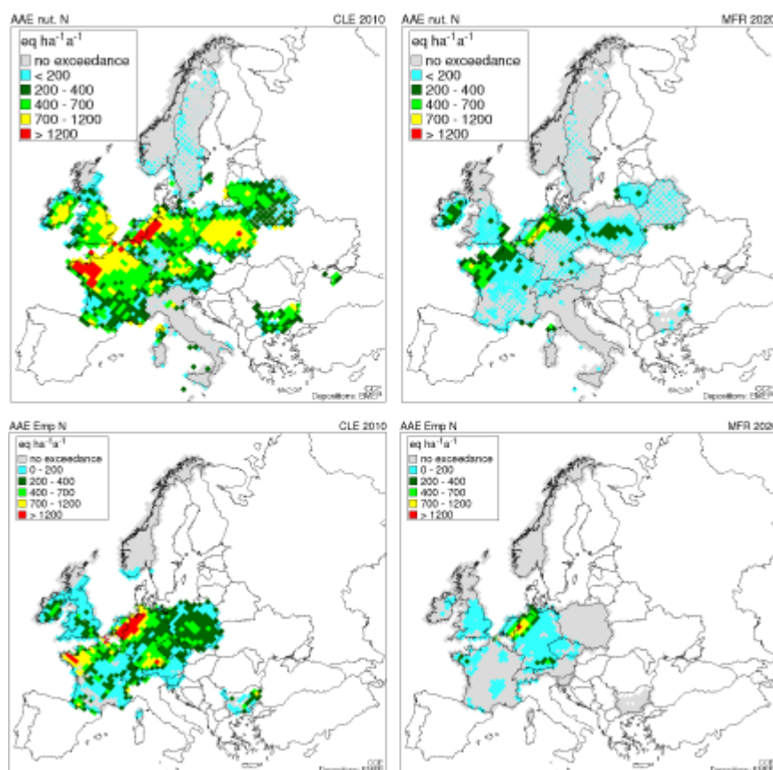
Figure 2-6. Exceedances for CLE 2010 (left) and MFR 2020 (right) for modelled critical loads (top row) and empirical loads (bottom row) of nitrogen.
