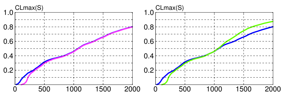
Figure 2-17. Cumulative distributions of \text{CL}_{\text{maxS}} computed from the European background data base using \text{Al:Bc}=1 (blue), \text{Al:Bc} = 1 only if [\text{Al}] > 0.1 \text{ eq m}^{-3} (magenta, left) and with the additional condition that [\text{Al}] < 1 \text{ eq m}^{-3} (green, right).
