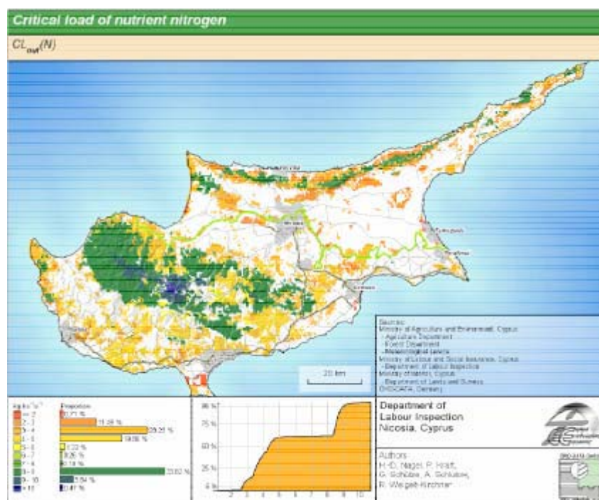
Figure CY-2. Regional distribution of critical loads of nutrient nitrogen, CL_{nut}N , in Cyprus.
