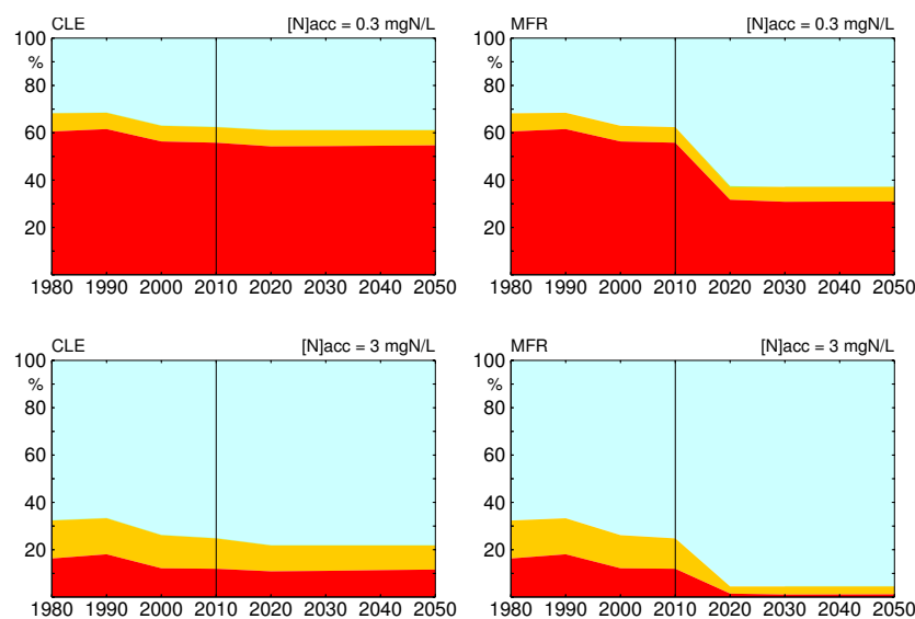
Figure 3-8: Temporal development of the areal share of the four categories defined in Figure 3-7 for the two scenarios (CLE and MFR) and two criteria ( [N]_{acc}=0.3 and [N]_{acc}=3 \text{ mg N L}^{-1} ). See Table 3-1 for colour codes (and exact values in 2020).
