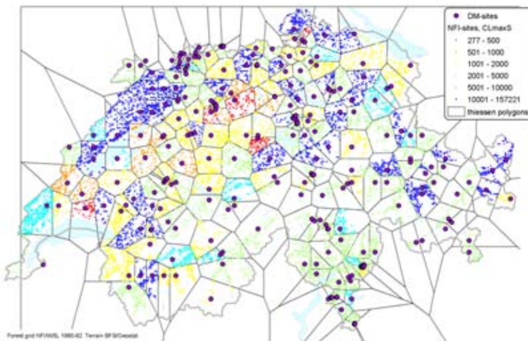
Figure CH-1. The acidity parameters (e.g. CL_{maxS} in \text{eq ha}^{-1} \text{ a}^{-1} ) at the DM-sites are spatially expanded to the NFI-sites using Thiessen-polygons.
