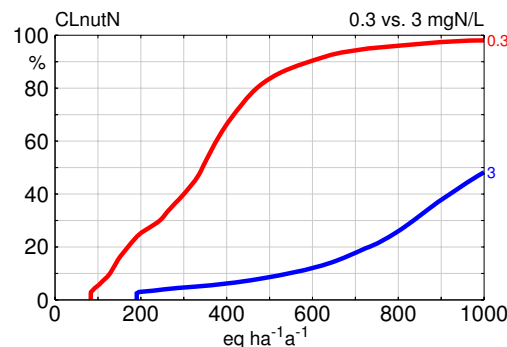
Figure 3-2. Cumulative distribution functions (cdfs) of the European nutrient N critical loads (653,962 sites) computed with EU-DB and two different acceptable nitrogen concentrations: 0.3 mg N L -1 (red cdf) and 3 mg N L -1 (blue cdf).
