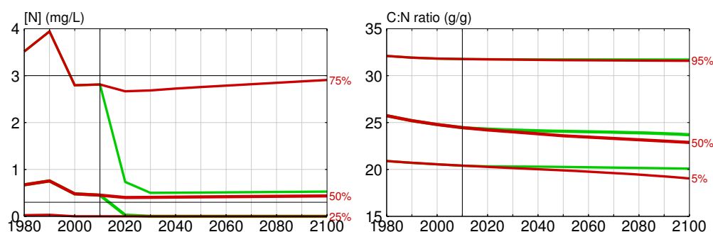
Figure 3-5. 25 th , median and 75 th percentile traces of the N concentration (left) and the 5 th , median and 95 th percentile traces of the C:N ratio (right) for the CLE (red) and MFR (green) scenarios.
