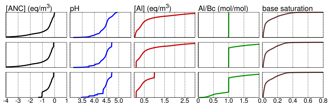
Figure 2-16. Cumulative distributions of the variables in Figure 2-15 computed from the European background data base using \text{Al:Bc} = 1 (top row), \text{Al:Bc} = 1 only if [\text{Al}] > 0.1 \text{ eq m}^{-3} (centre) and with the additional condition that [\text{Al}] < 1 \text{ eq m}^{-3} (bottom).
