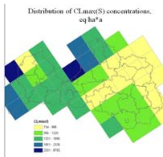
Figure LV-7. Average CL_{max}S in EMEP grid cells.
