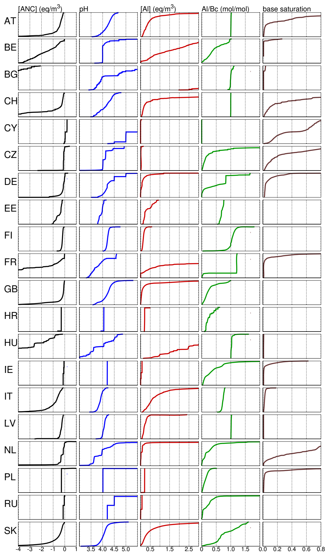
Figure 2-15. Cumulative distributions of variables used as chemical criteria computed from the given ANC flux. The Oliver model was assumed for organic ion dissociation and the Gapon model for cation exchange. Base saturation is not shown if exchange constants were not available.
