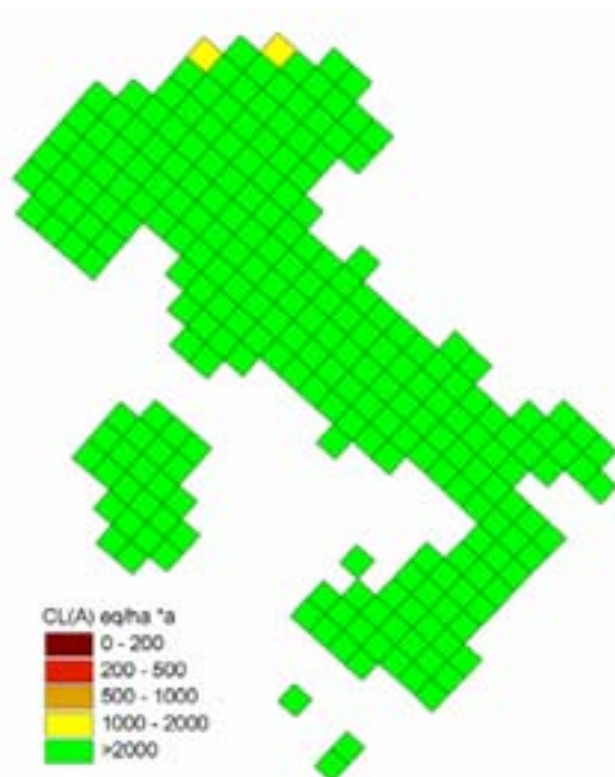
Figure IT-1. Critical load of acidity.
