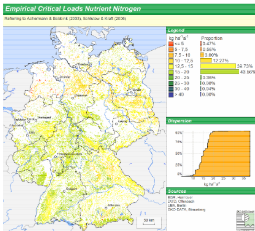
Figure DE-8. Regional distribution of empirical critical loads of nitrogen for terrestrial ecosystems in Germany.
