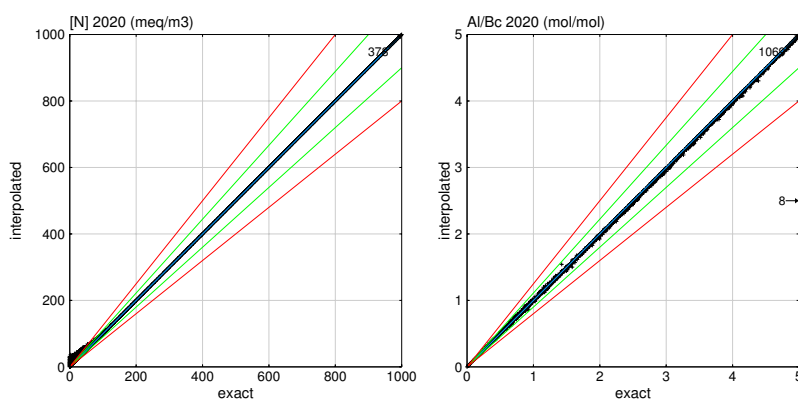
Figure 3-11. Exact versus interpolated N concentration (left) and Al:Bc ratio (right). The green and red lines show the 10% and 20% deviation, respectively, from the 1-to-1 line.
