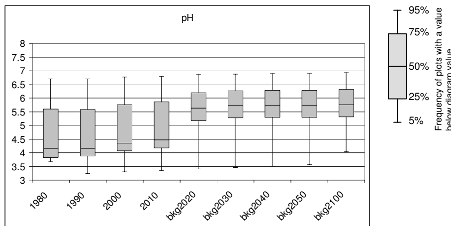
Figure DE-7. Trend of the distribution of pH values in Germany following the 'background' deposition scenario (only natural sources from 2020) (101098 plots calculated).
