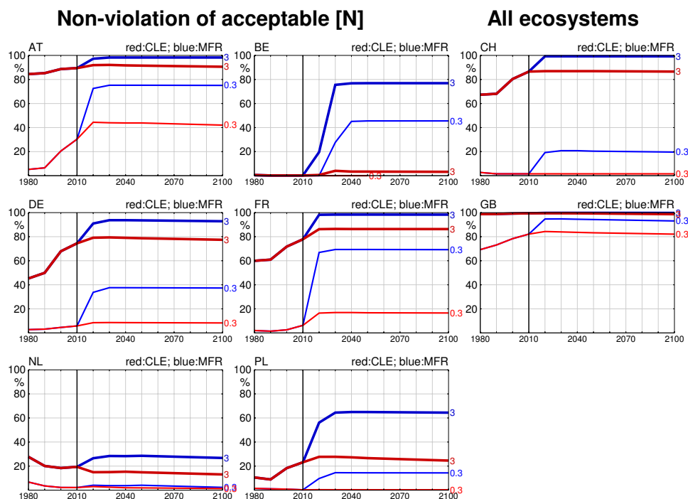
Figure 2-13. Temporal development of the ecosystem area (in % of total) on which the total N concentration is below the limits of 0.3 and 3 mgN L -1 , resp., for the CLE (red) and MFR (blue) scenarios.
