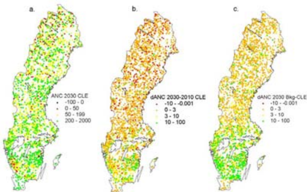
Figure SE-1. Map of Sweden, with the RI00 lakes marked with different colours according to their ANC values in 2030 under the CLE scenario (a), marked with different colours according to the ANC improvement between 2010 and 2030 under the CLE scenario (b) and marked with different colours according to the difference in ANC 2030 between CLE and the Bkg scenarios (c).
