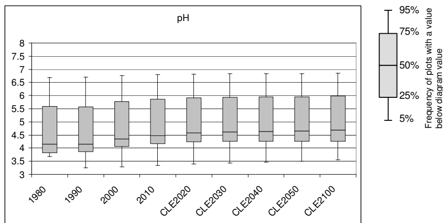
Figure DE-5. Trend of the distribution of pH values in Germany following the 'current legislation' deposition scenario (101098 Plots calculated).
