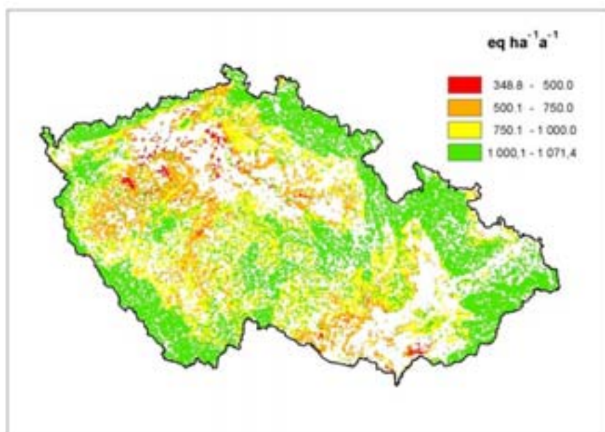
Figure CZ-2. Critical loads of nutrient nitrogen and empirical critical loads for forest ecosystems.
