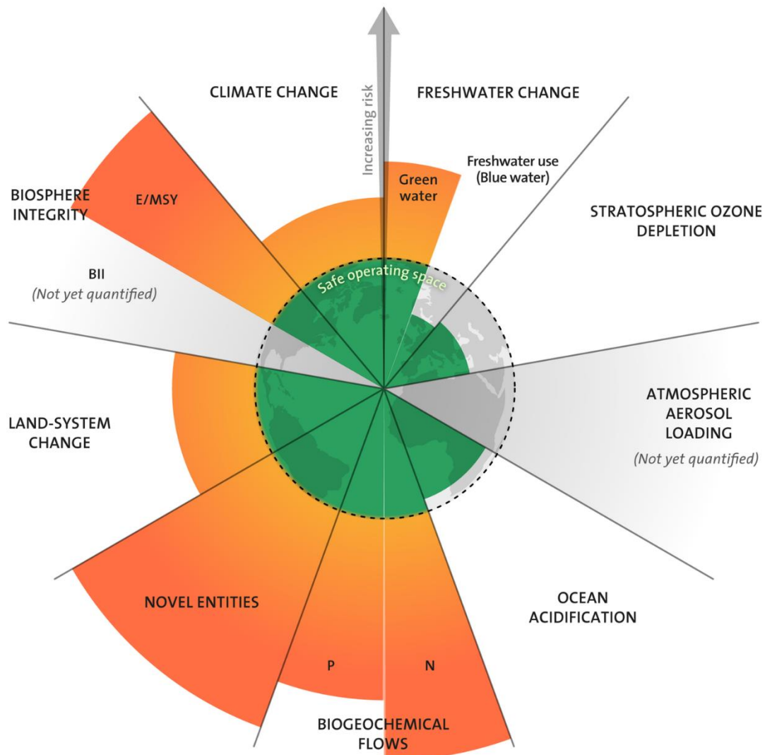
Figure 3. Planetary boundaries
