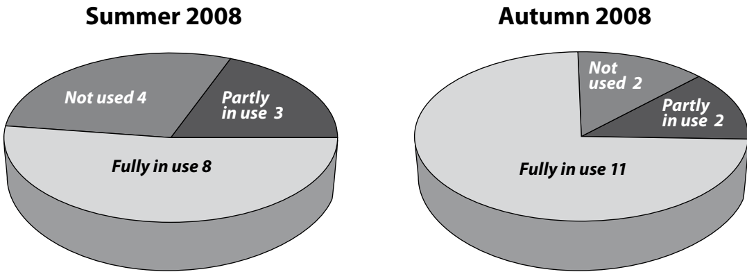
Figure 3: UDDT acceptance. 18
