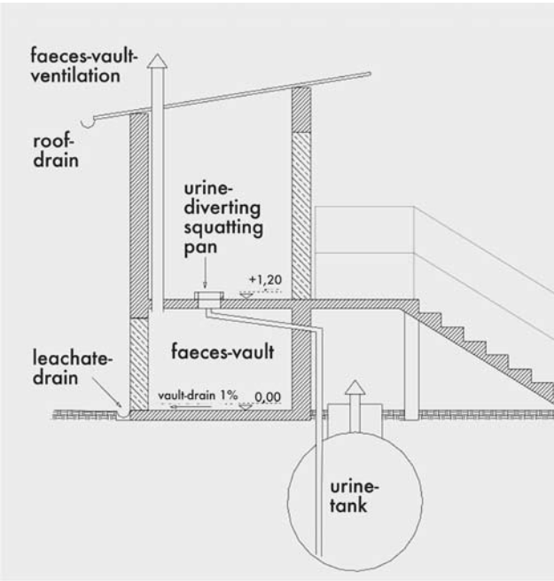
Figure 1. Cross section of UDDT. Source: WECF.
