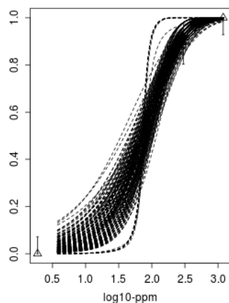
bootstrap curves based on model averaging
